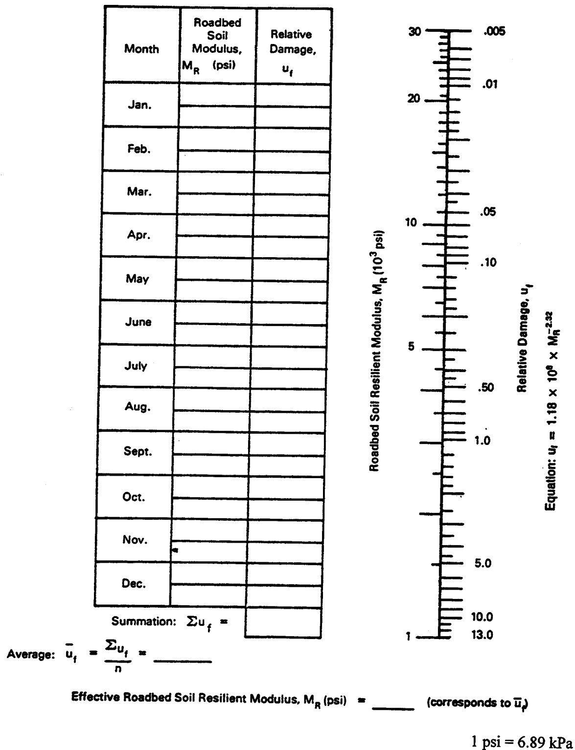
Figure 45. Chart for estimating effective roadbed soil resilient modulus for flexible pavements designed using the serviceability criteria (1).
