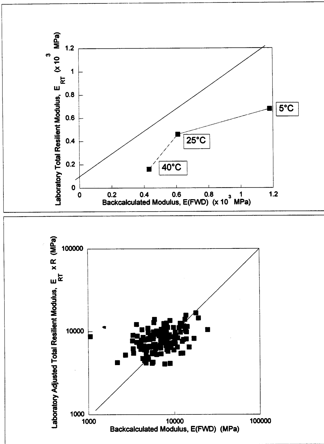
Figure 27. Comparison of laboratory measured values determined at the mid-depth temperature to the backcalculated moduli.
