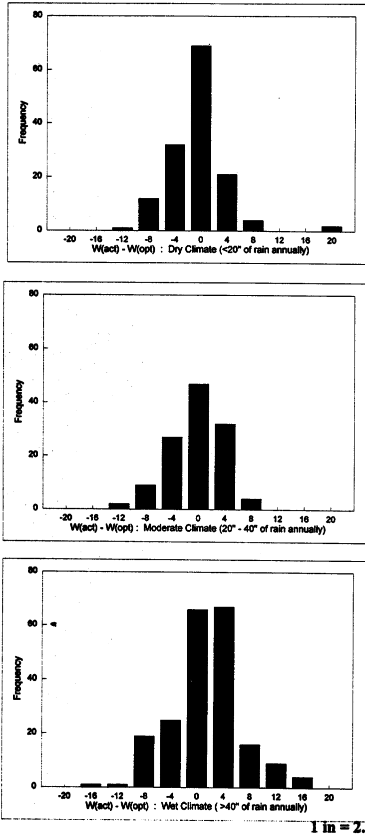
Figure 35. Frequency of difference between optimum and actual moisture contents for granular base layers in GPS sections with no positive drainage system.
