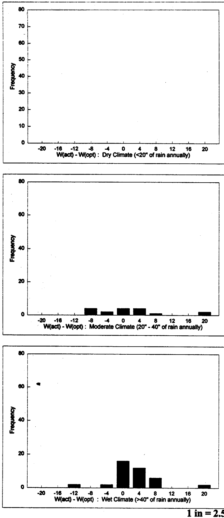
Figure 36. Frequency of difference between optimum and actual moisture contents for granular base layers in GPS sections with positive drainage systems.
