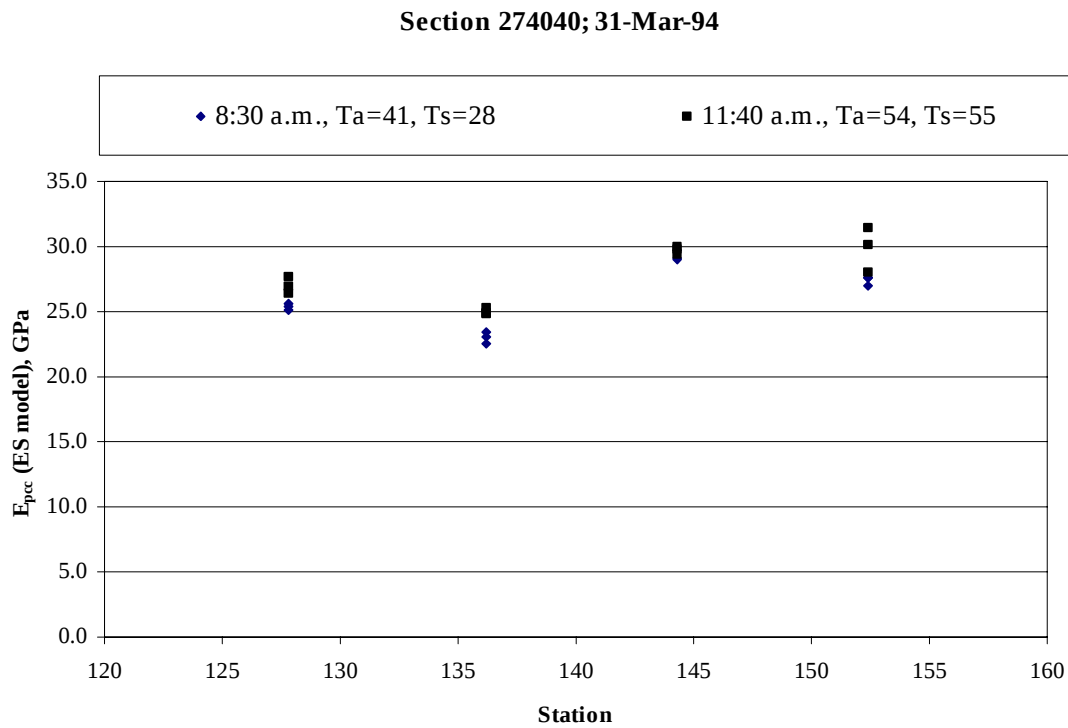
Figure 78. Daily variation in backcalculated PCC modulus of elasticity (ES model), section 274040 (March 1994).
