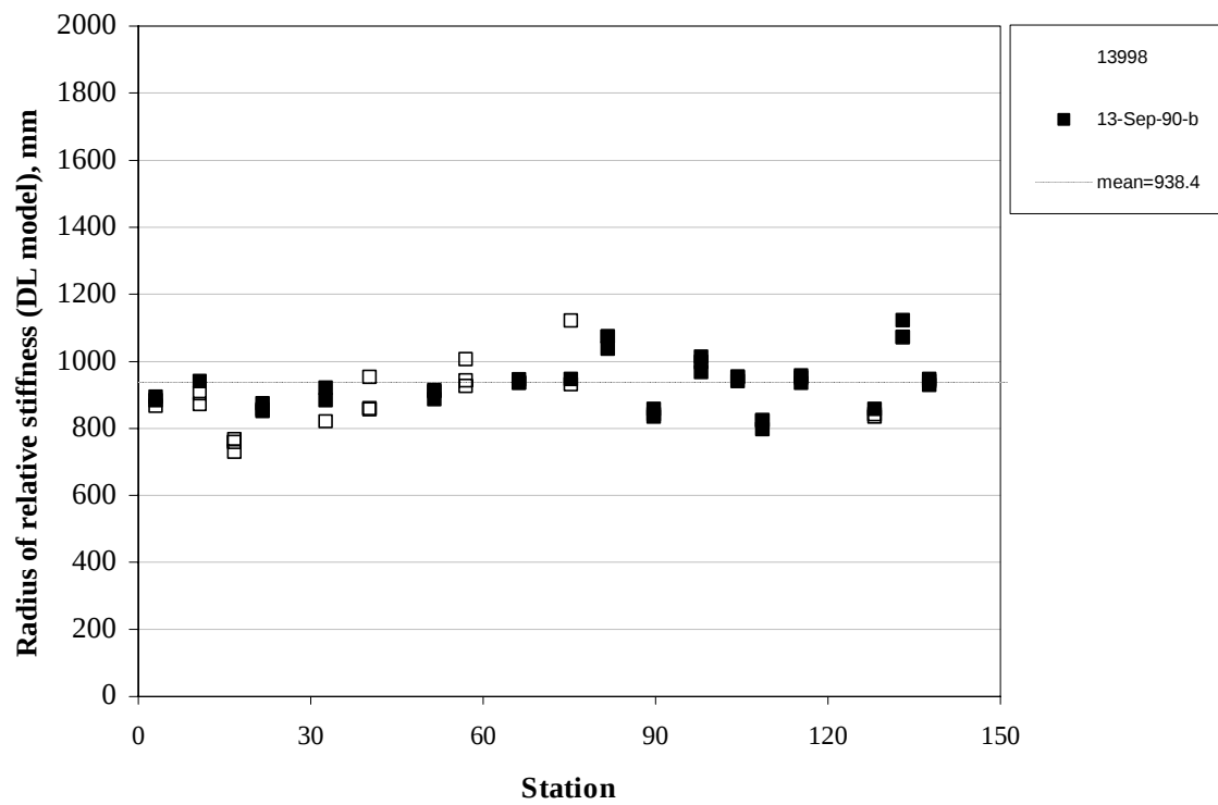
Figure 94. Backcalculated radius of relative stiffness (DL model) for section 013998.
