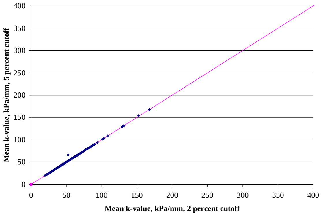
Figure 19. Comparison of mean k-values with 2 and 5 percent cutoff limit for deflection basin acceptance for LTPP SPS section.
