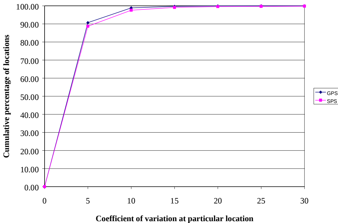
Figure 29. Coefficient of variation in radius of relative stiffness (ES model) for multiple load levels (GPS and SPS sections).
