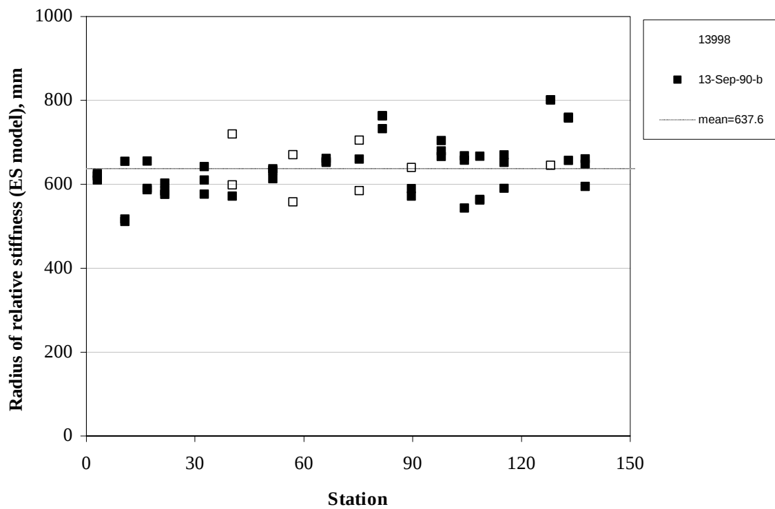
Figure 106. Backcalculated radius of relative stiffness (ES model) for section 015008.
