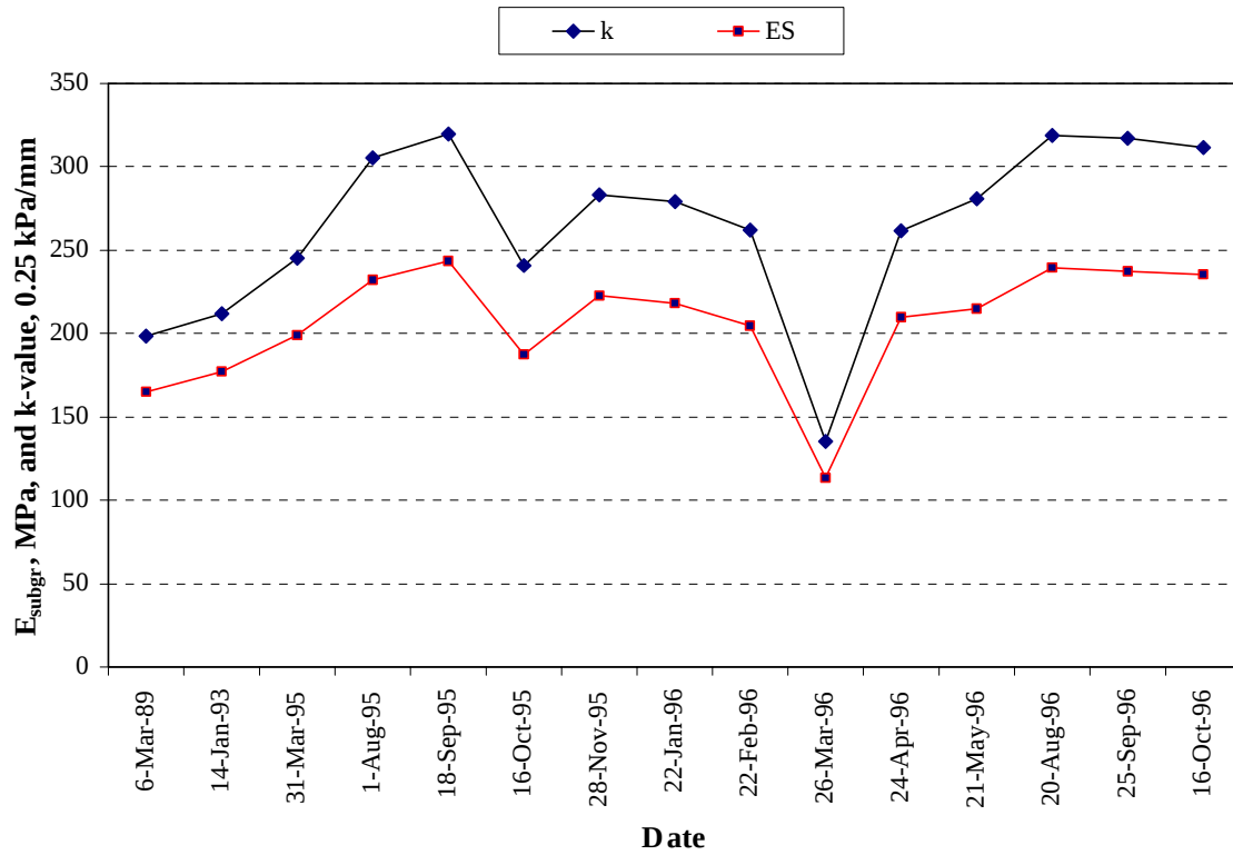
Figure 79. Seasonal variation in backcalculated subgrade moduli, section 133019.
