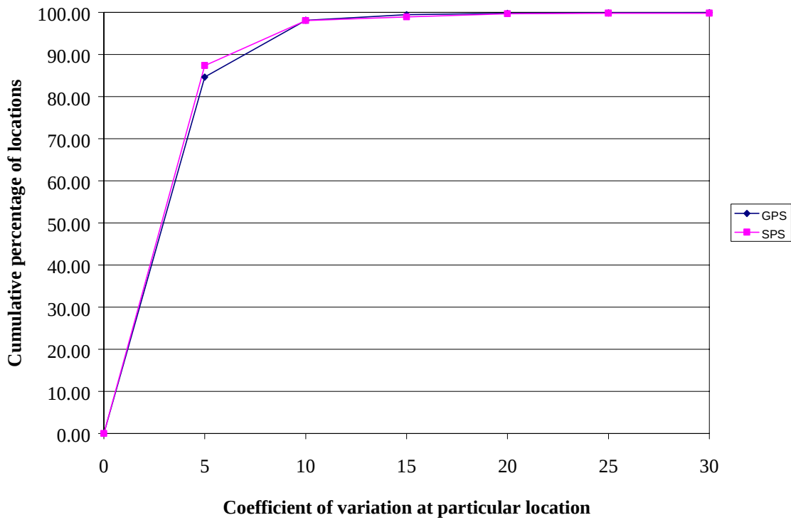
Figure 28. Coefficient of variation in backcalculated modulus of elasticity of subgrade for multiple load levels (GPS and SPS sections).
