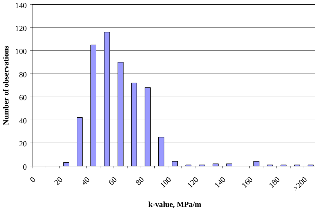
Figure 56. Frequency distribution of backcalculated k -values for SMP LTPP sections.
