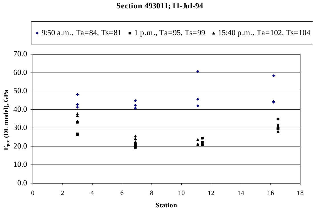
Figure 73. Daily variation in backcalculated PCC modulus of elasticity (DL model), section 493011 (July 1994).
