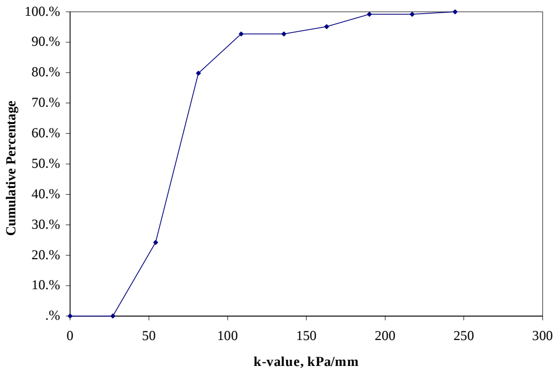
Figure 14. Distribution of k-values from Best Fit 4 method for the FWD passes for which Best Fit 7 was not successful.
