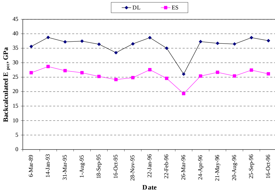
Figure 80. Seasonal variation in backcalculated PCC modulus of elasticity, section 133019.
