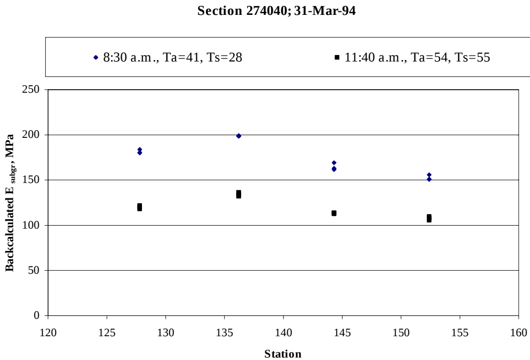
Figure 76. Daily variation in backcalculated subgrade modulus of elasticity, section 274040 (March 1994).
