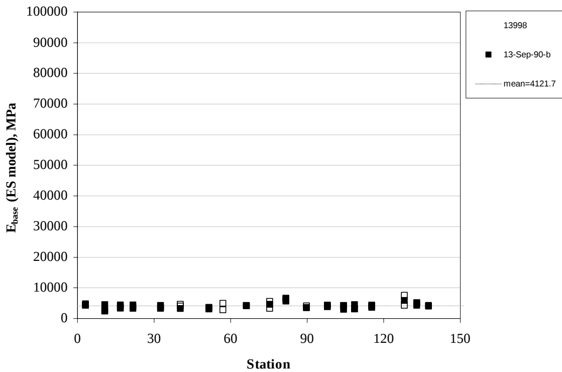
Figure 108. Backcalculated elastic modulus of base (ES model) for section 015008.
