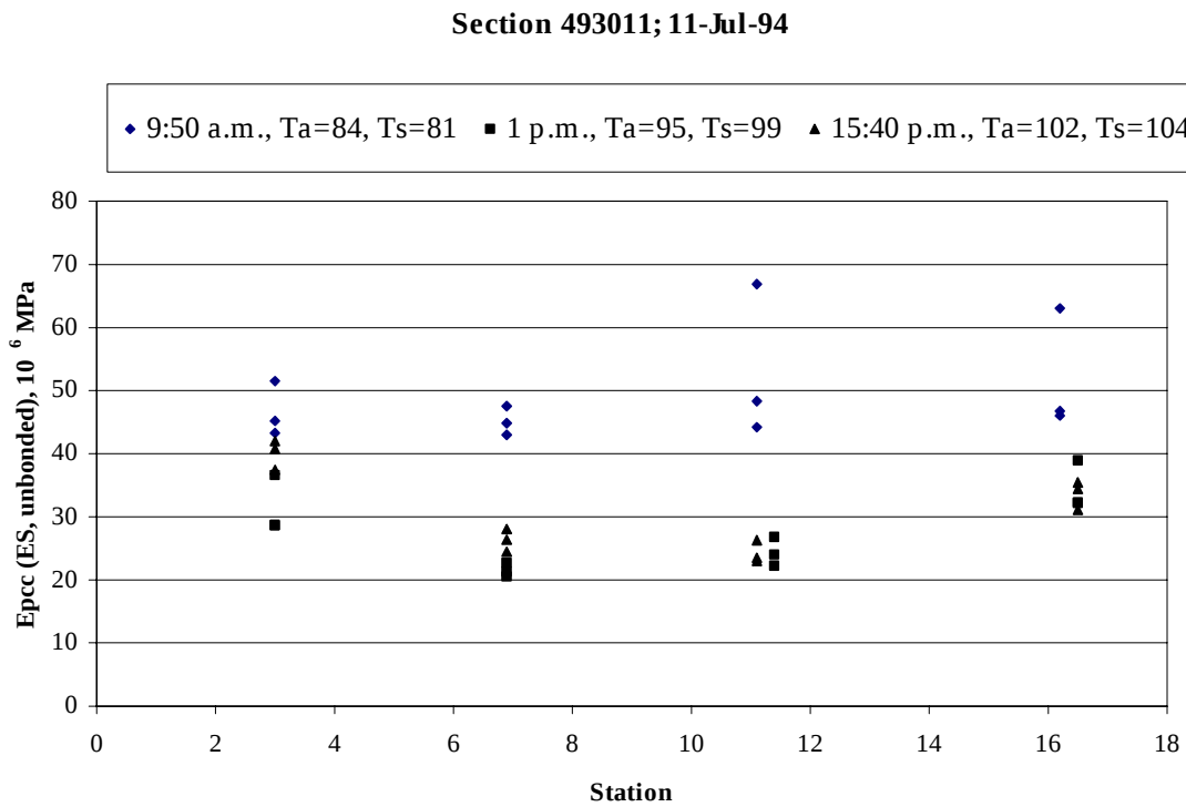
Figure 74. Daily variation in backcalculated PCC modulus of elasticity (ES model), section 493011 (July 1994).
