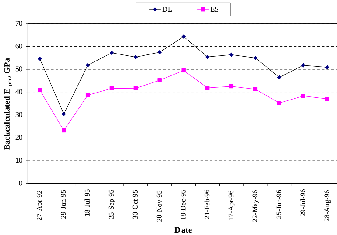
Figure 82. Seasonal variation in backcalculated PCC modulus of elasticity, section 533813.
