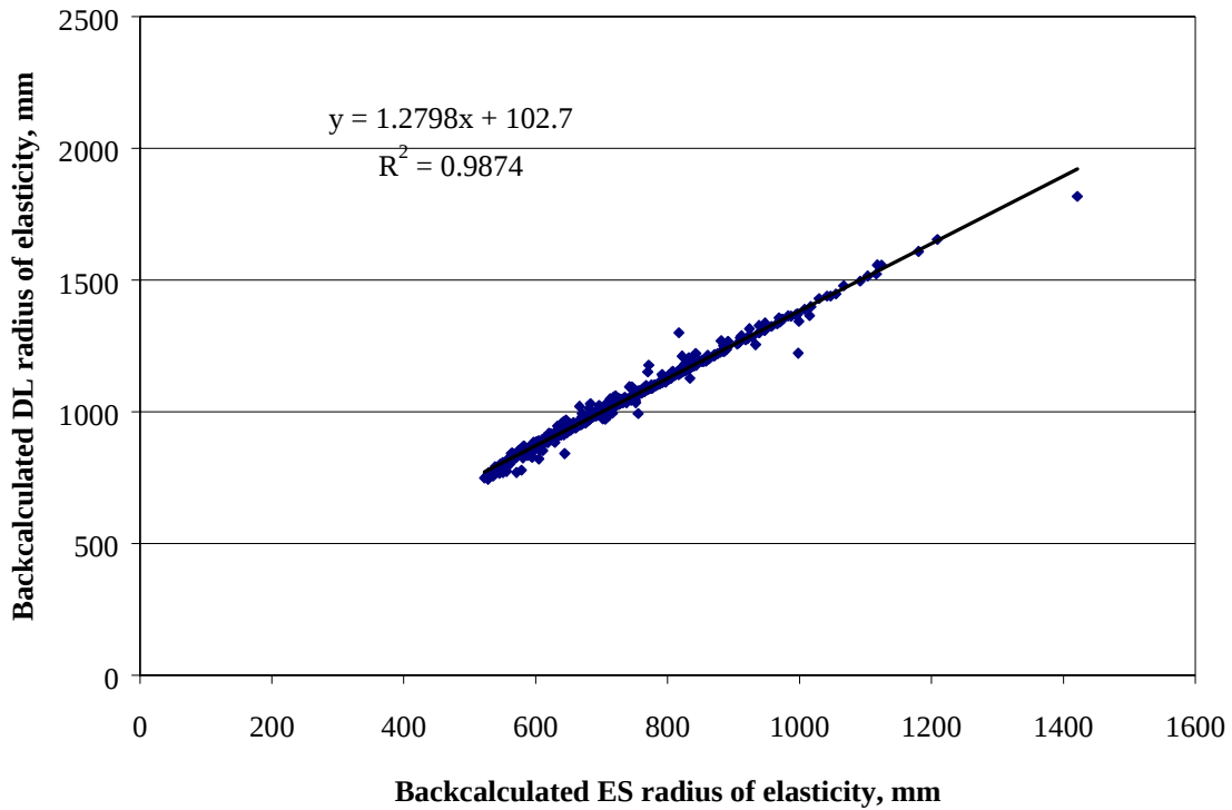
Figure 41. ES radius of relative stiffness versus DL radius of relative stiffness.
