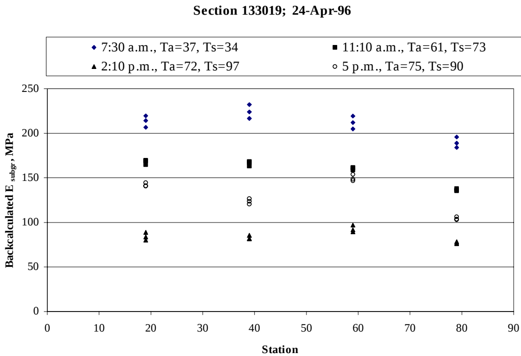
Figure 68. Daily variation in backcalculated subgrade modulus of elasticity, section 133019 (April 1996).
