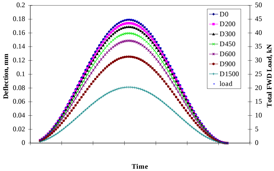
Figure 86. Quasi-static pavement responses to FWD loading.
