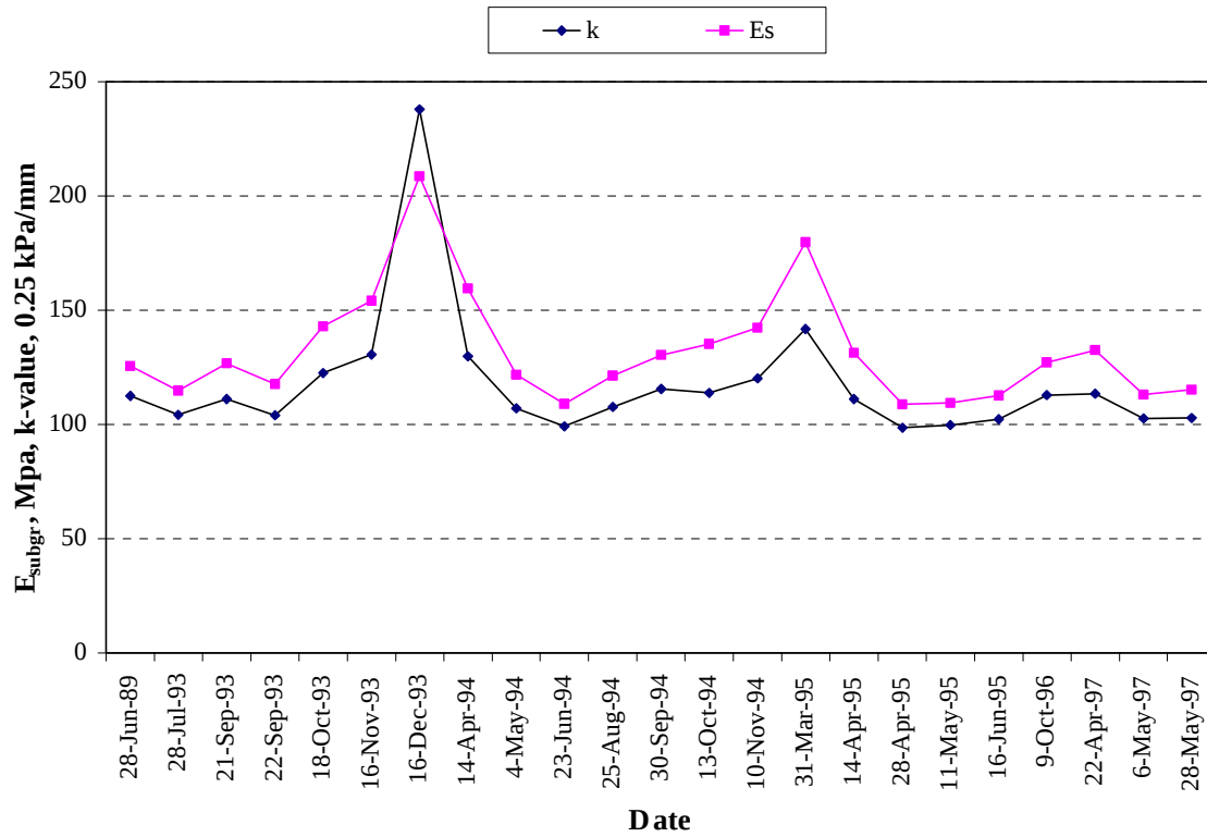
Figure 83. Seasonal variation in backcalculated subgrade moduli, section 274040.
