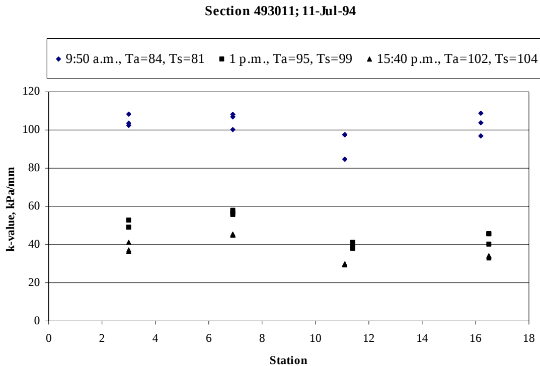
Figure 71. Daily variation in backcalculated k-value, section 493011 (July 1994).
