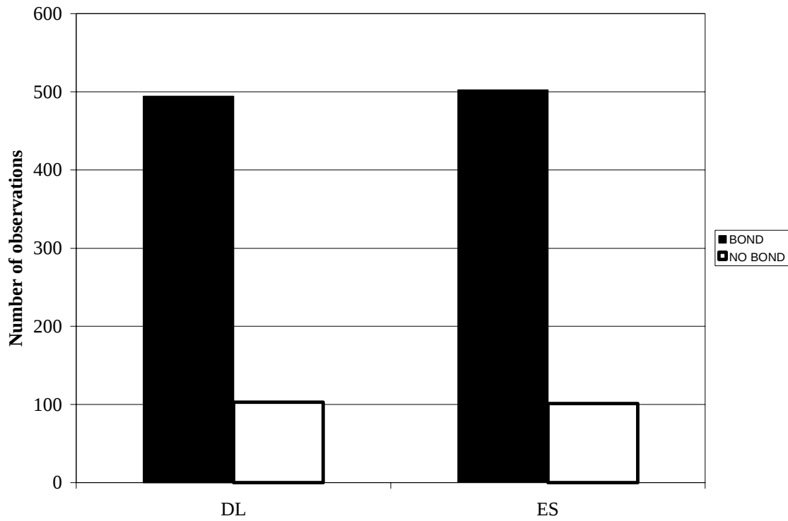
Figure 42. Distribution of bond/no bond interface condition for GPS and SPS LTPP sections.
