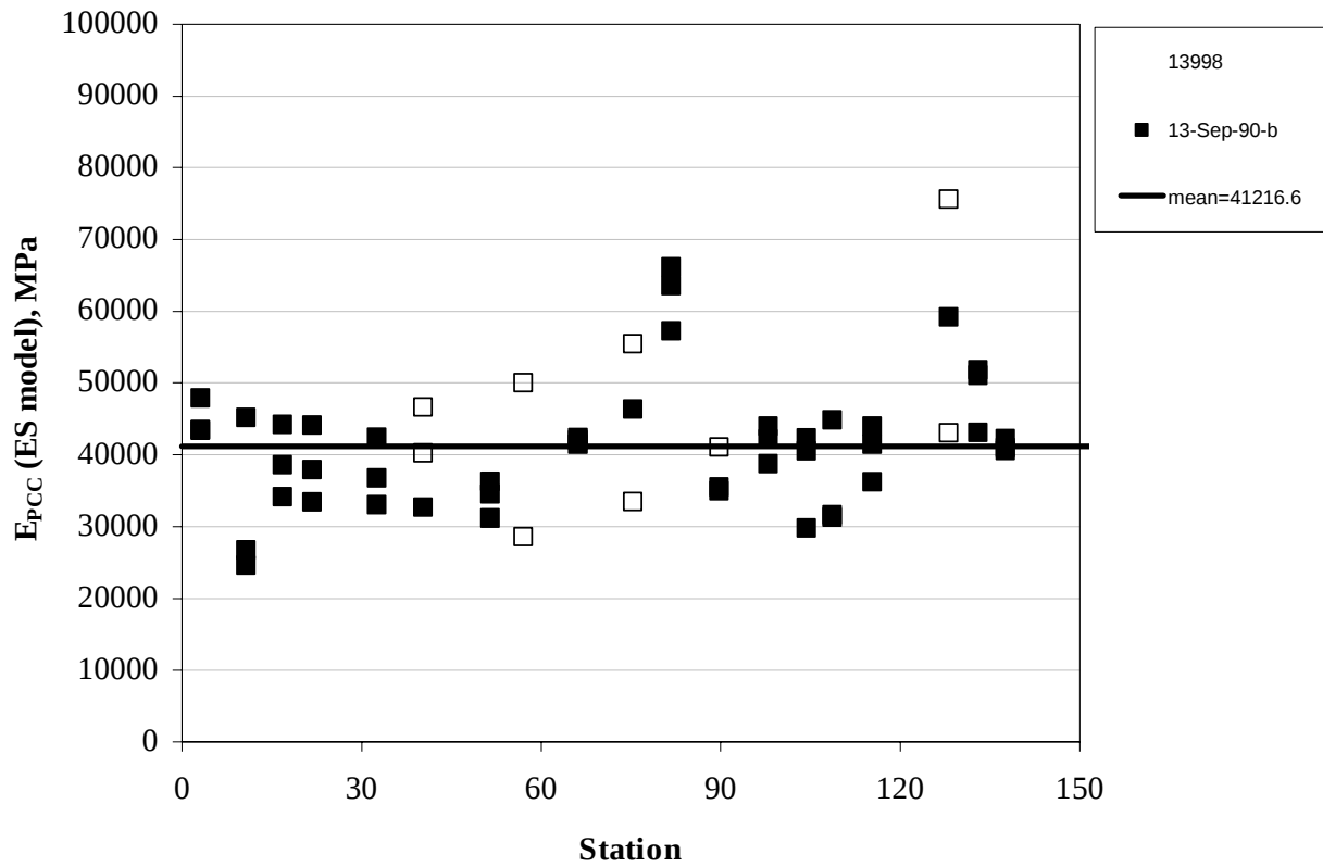
Figure 99. Backcalculated PCC elastic modulus (ES model) for section 013998.
