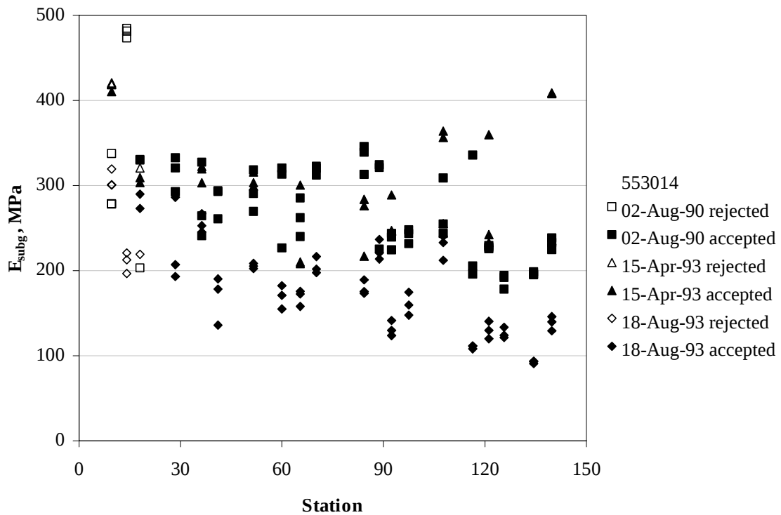
Figure 33. Backcalculated modulus of elasticity of subgrade for section 553014.
