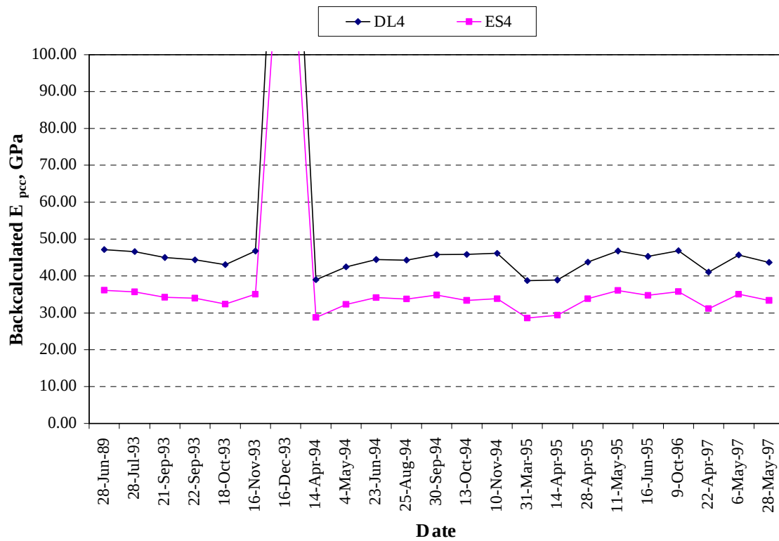
Figure 84. Seasonal variation in backcalculated PCC modulus of elasticity, section 274040.
