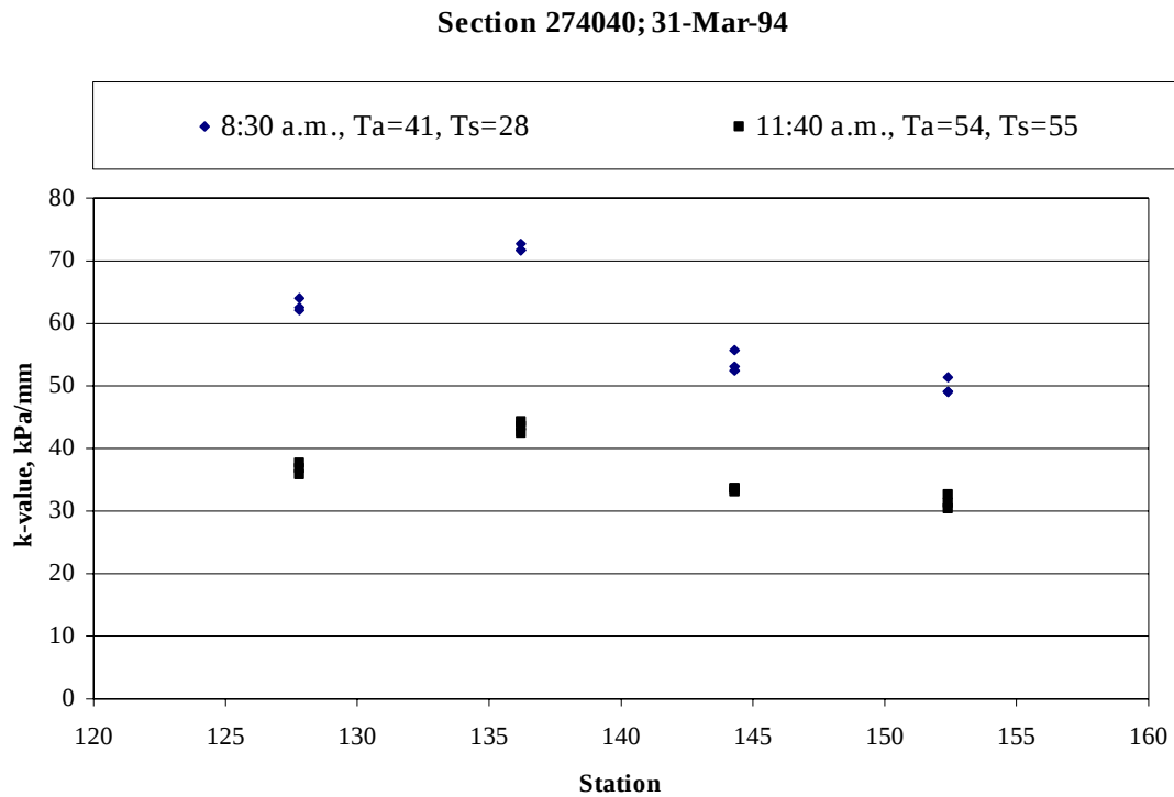
Figure 75. Daily variation in backcalculated k-value, section 274040 (March 1994).
