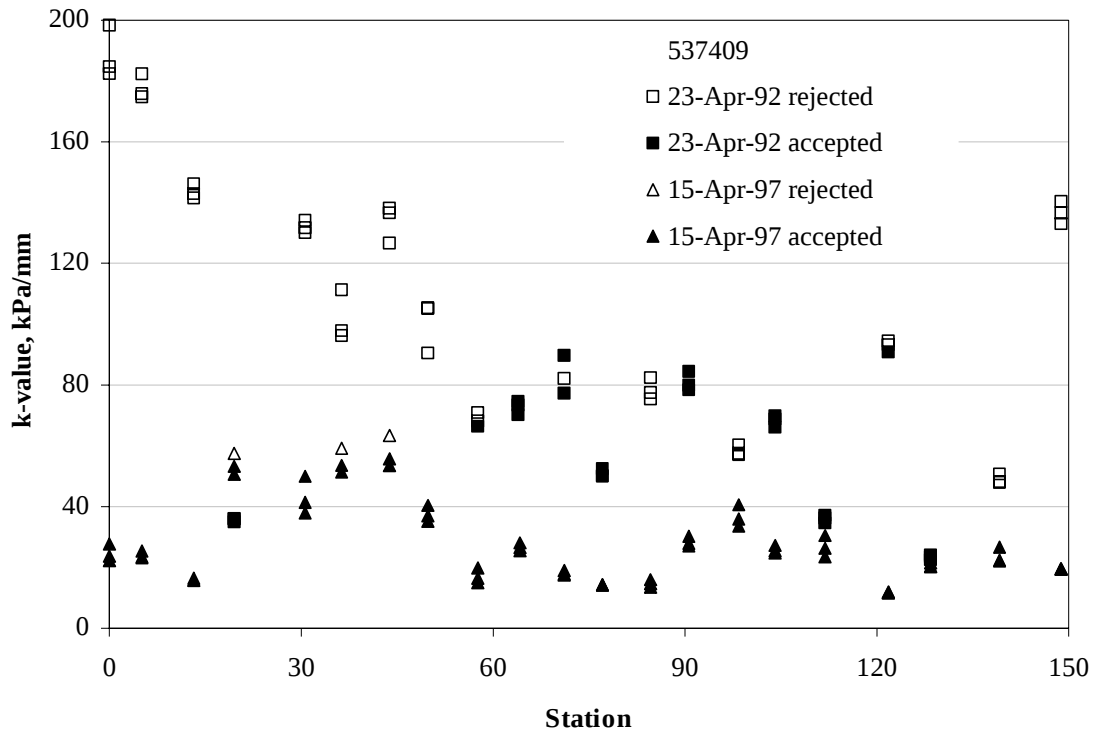
Figure 32. Backcalculated k-values for section 537409.
