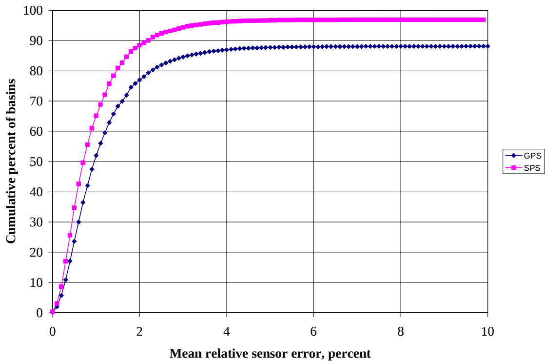
Figure 17. Cumulative chart of mean absolute values of relative errors for LTPP GPS and SPS sections (ES subgrade model).
