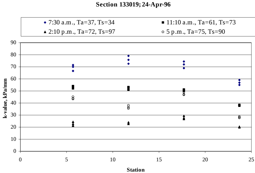
Figure 67. Daily variation in backcalculated k-value, section 133019 (April 1996).
