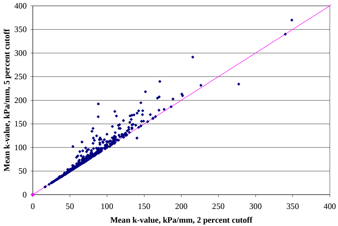
Figure 18. Comparison of mean k-values with 2 and 5 percent cutoff limit for deflection basin acceptance for LTPP GPS section.
