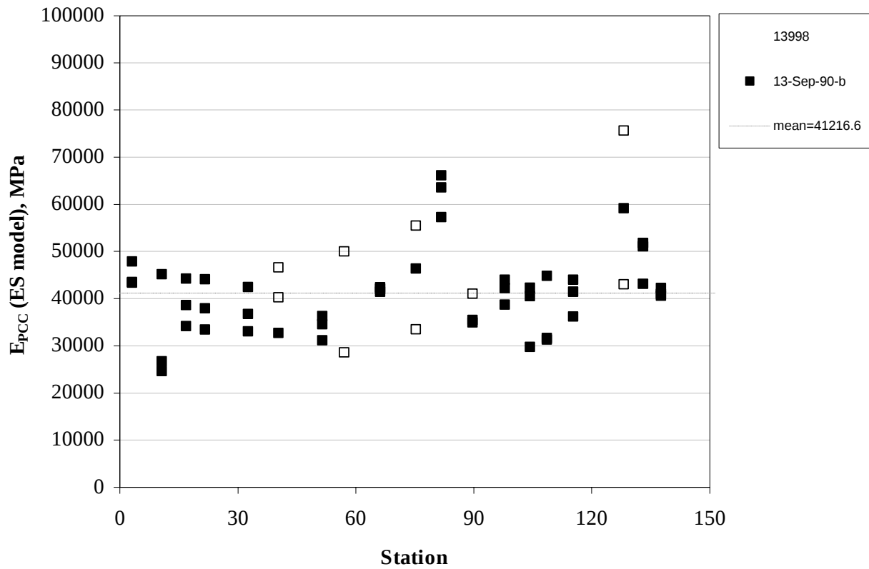
Figure 107. Backcalculated PCC elastic modulus (ES model) for section 015008.
