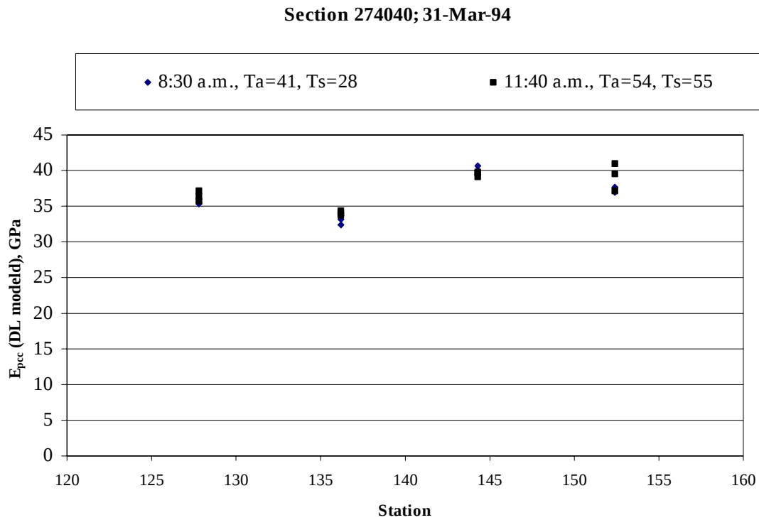
Figure 77. Daily variation in backcalculated PCC modulus of elasticity (DL model), section 274040 (March 1994).
