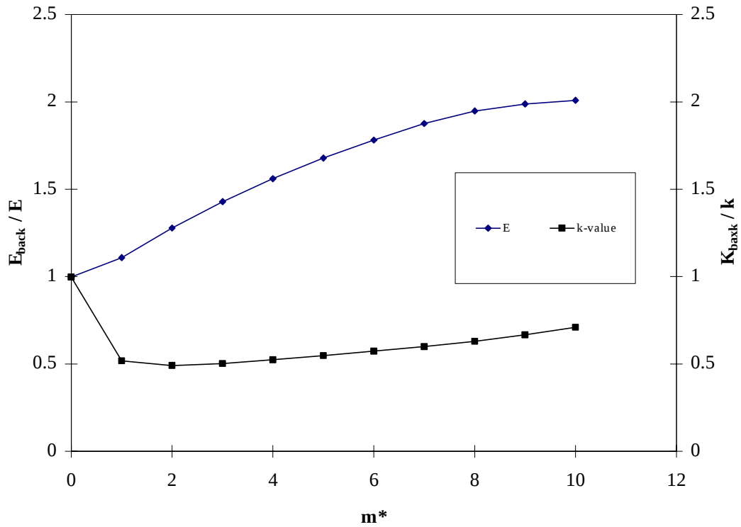
Figure 91. Effect of pavement inertia on the results of backcalculation.
