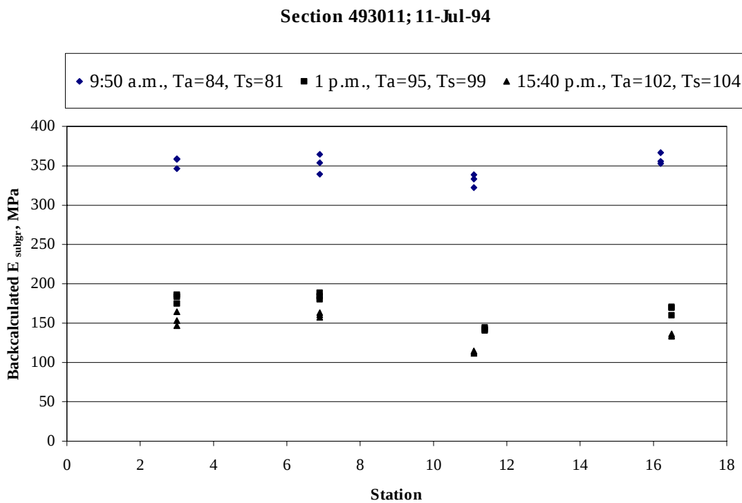
Figure 72. Daily variation in backcalculated subgrade modulus of elasticity, section 493011 (July 1994).
