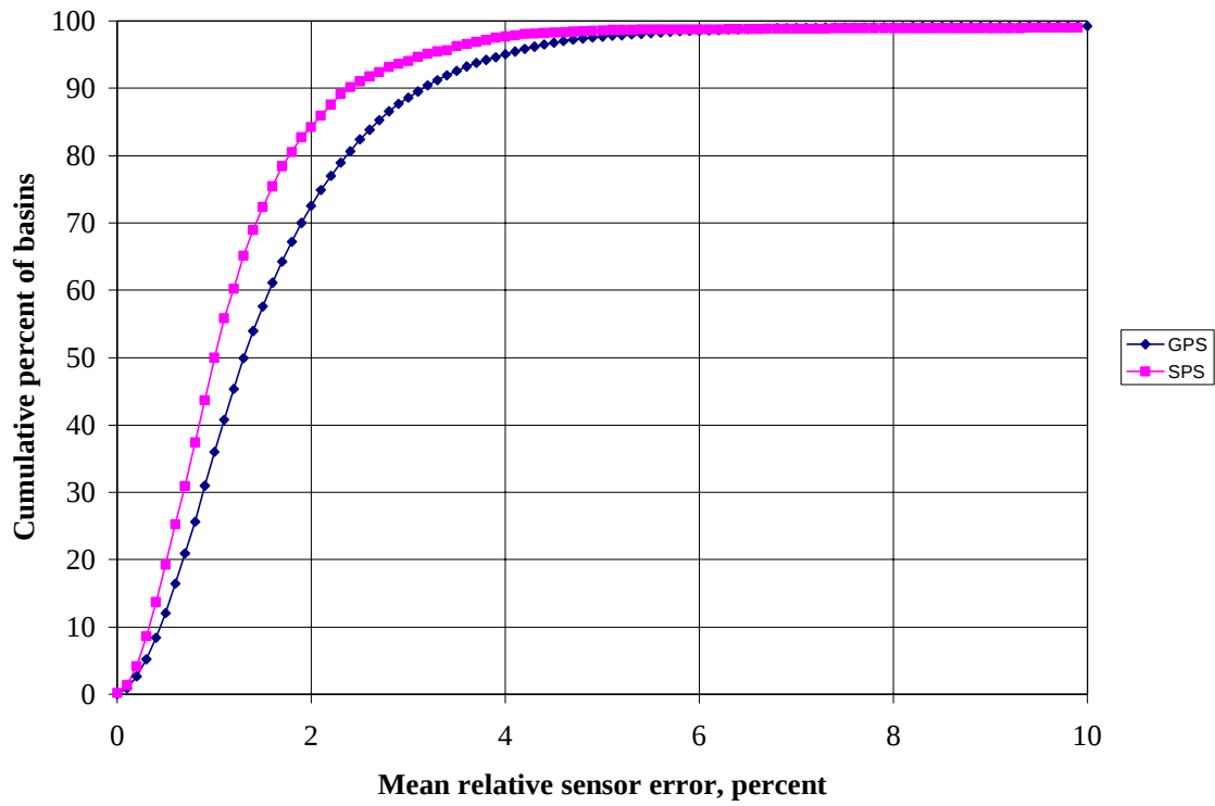
Figure 16. Cumulative chart of mean absolute values of relative errors for LTPP GPS and SPS sections (DL subgrade model).
