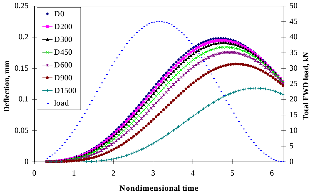
Figure 89. Effect of pavement inertia on FWD sensor deflections, m^*=4 .
