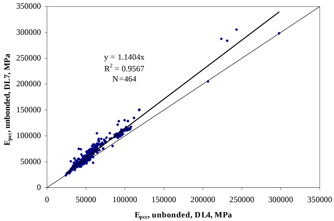
Figure 13. Backcalculated E_{pcc} for LTPP SMP sections, Best Fit 7 versus Best Fit 4 methods.
