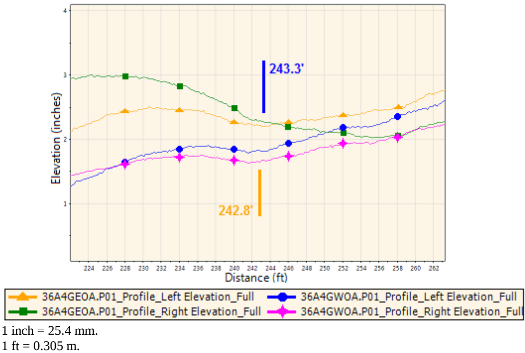
Figure 15. Chart. Example of a GRS-IBS bridge profile in St. Lawrence County, NY, at second interface (eastbound direction).
