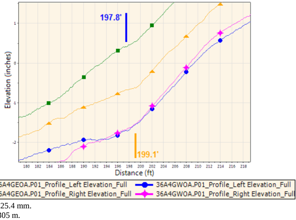
Figure 14. Chart. Example of a GRS-IBS bridge profile in St. Lawrence County, NY, at first interface (eastbound direction).
