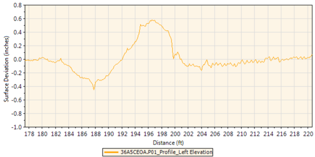
Figure 22. Chart. RSE surface deviations plot using ProVAL software of conventional bridge profile in St. Lawrence County, NY.
