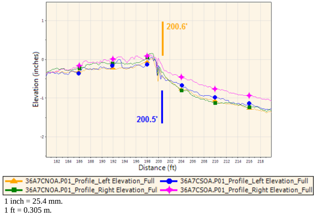
Figure 17. Chart. Example of a conventional bridge profile in St. Lawrence County, NY, at first interface (northbound direction).
