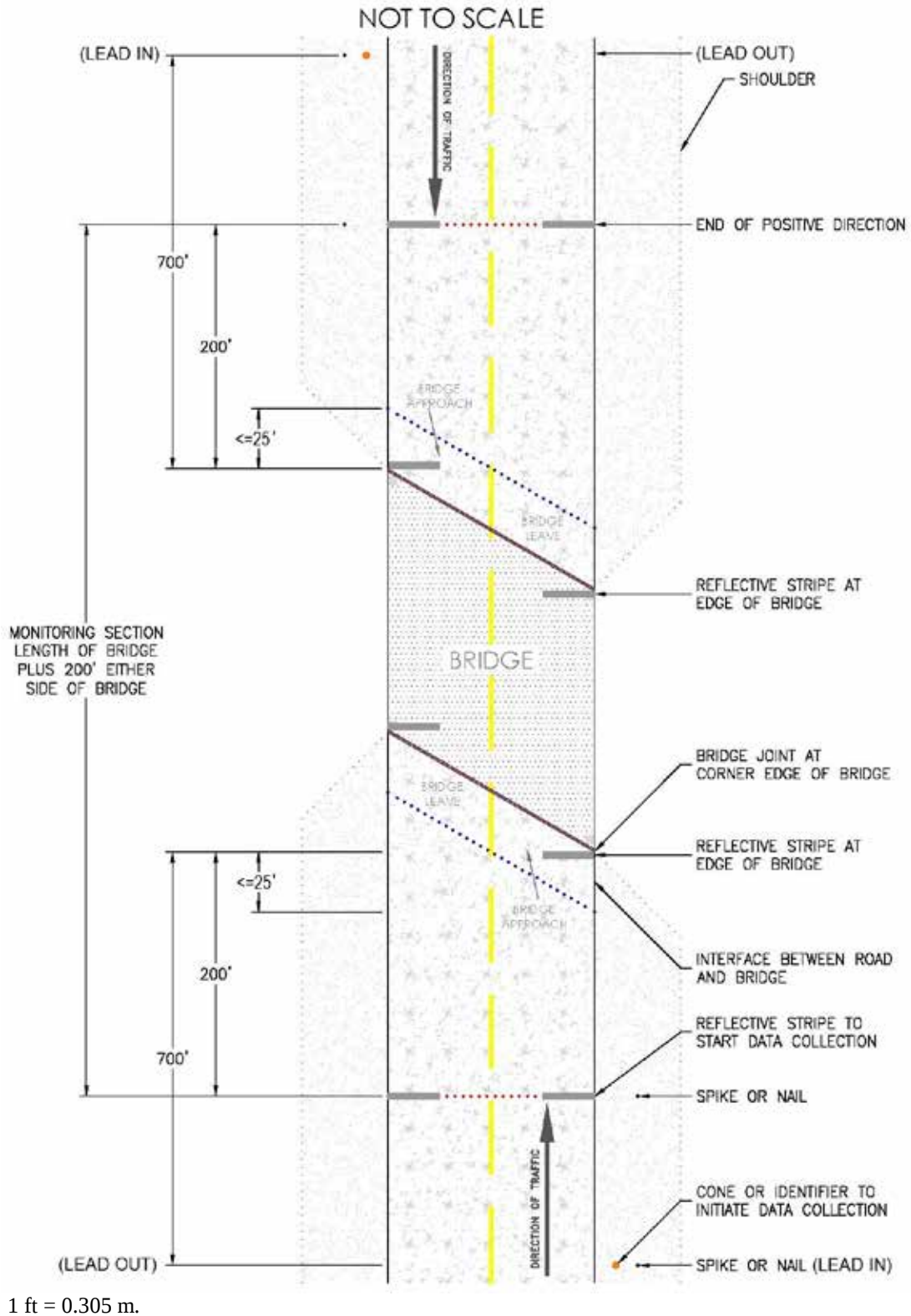
Figure 3. Drawing. Layout of bridge site with skewed joints.
