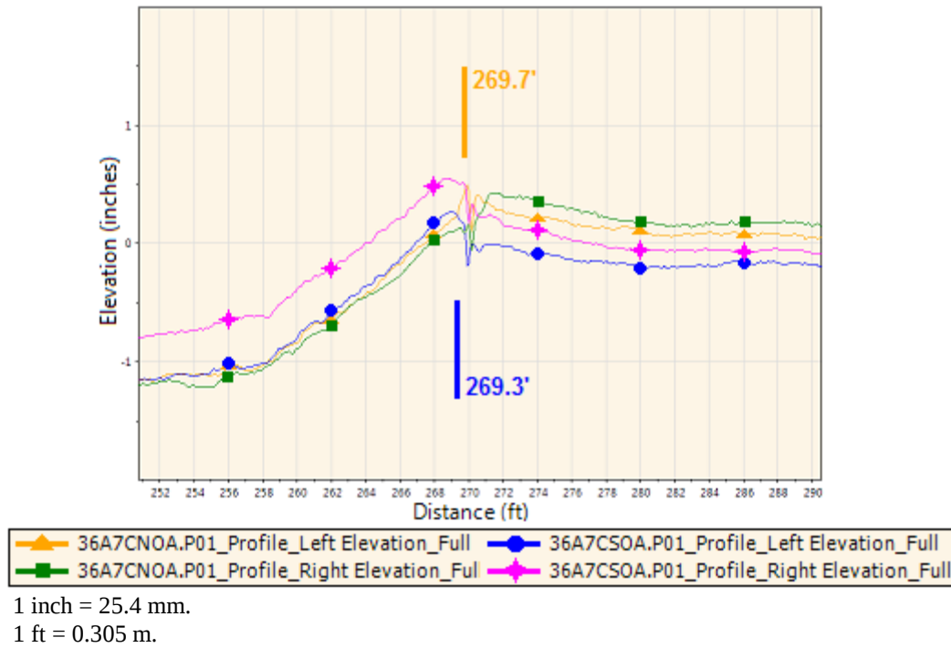
Figure 18. Chart. Example of a conventional bridge profile in St. Lawrence County, NY, at second interface (northbound direction).
