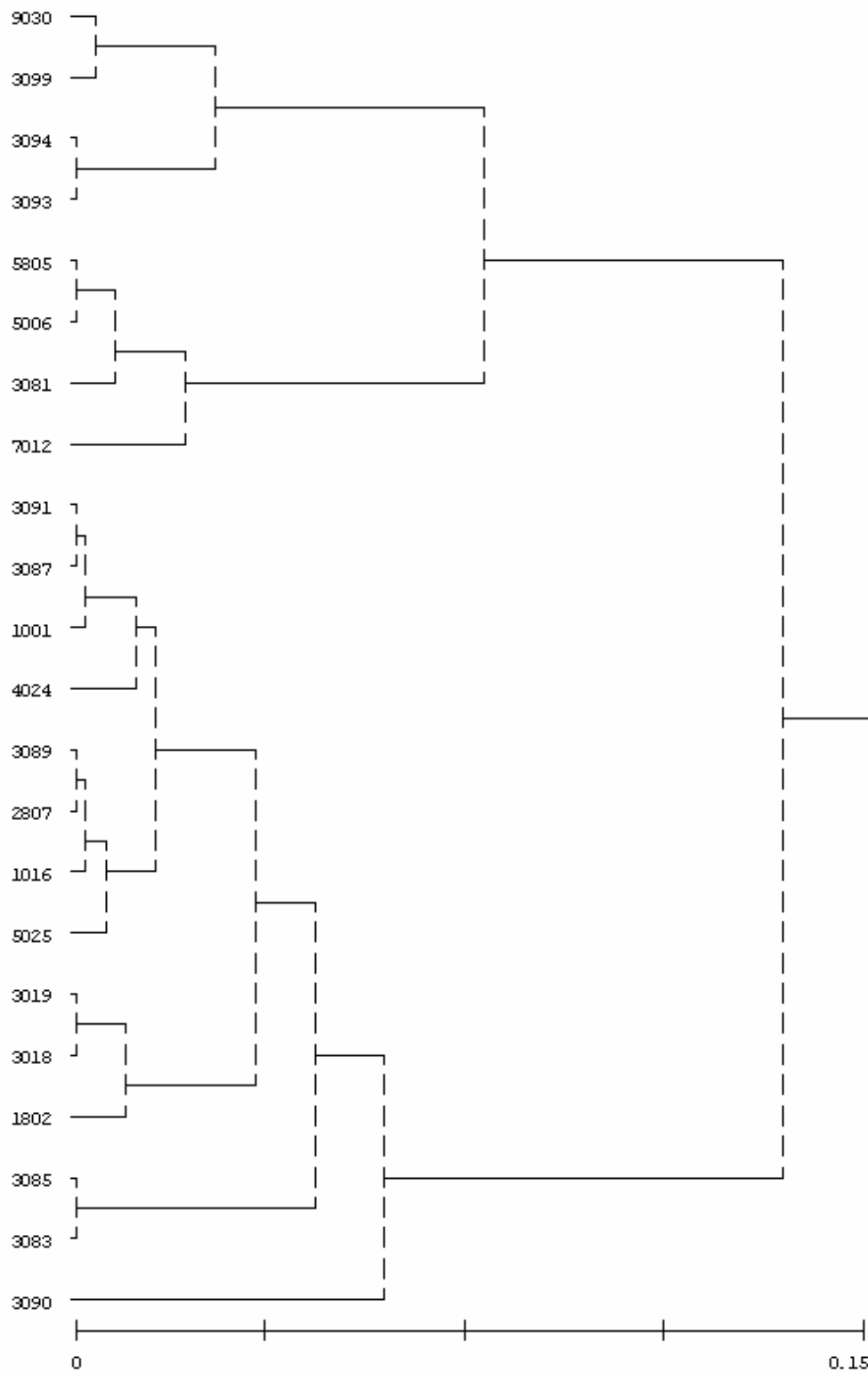
Figure 26. Clusters of LTPP sites by annual tandem-axle load distribution, Mississippi.
