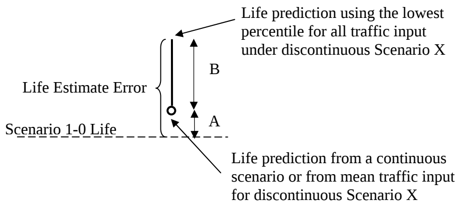
Figure 17. Components of the percentage difference between pavement life predictions for scenario X and those for scenario 1-0.
