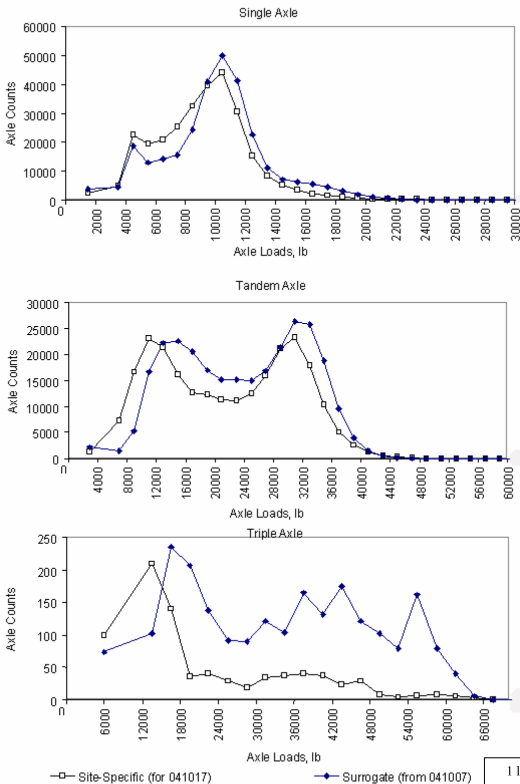
Figure 38. Comparison of site-specific and surrogate base annual spectra for 041017.
