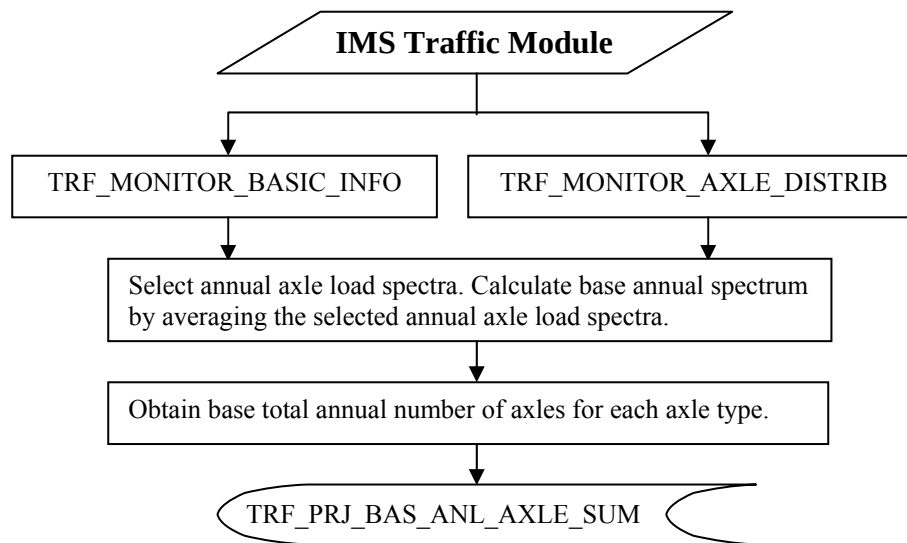
Figure 28. Flowchart for computation of the base annual axle load summary.
