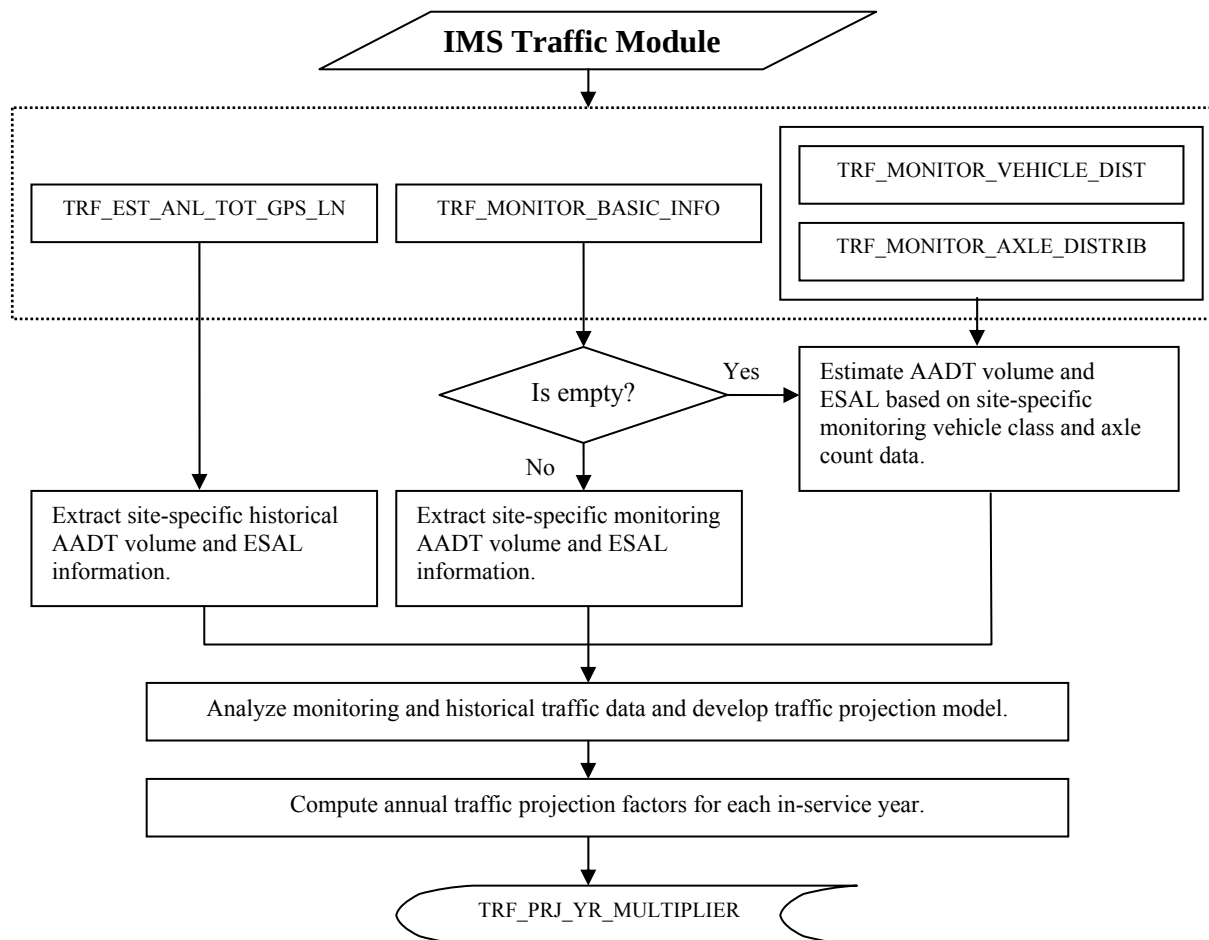
Figure 29. Flowchart for computation of the annual projection factors.
