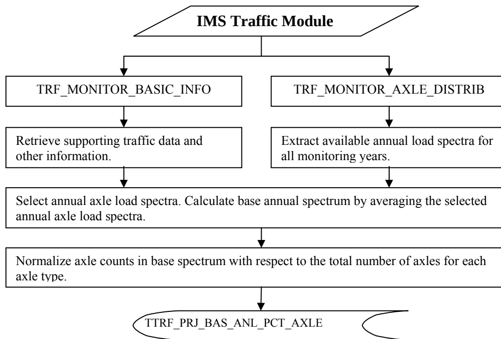
Figure 27. Flowchart for computation of the normalized base annual load spectra.
