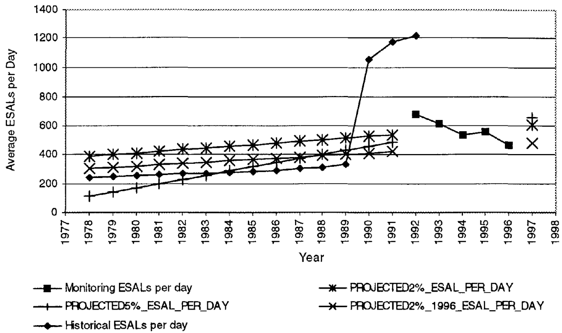
Figure 21. Comparison of projected, historical, and monitoring ESALs for Site 05-3059.
