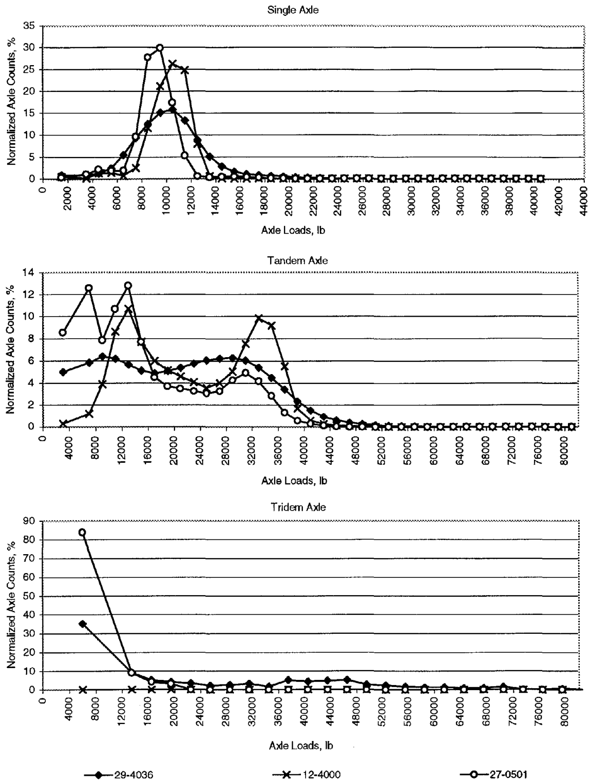
Figure 115. Normalized load spectra for Class 9 vehicles.
