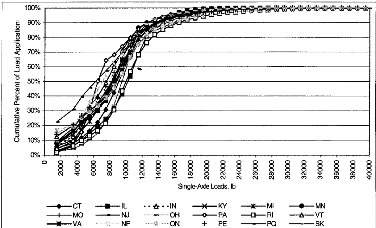
Figure 10. Cumulative distribution of single-axle loads for the NAR and NCR States/Provinces.
