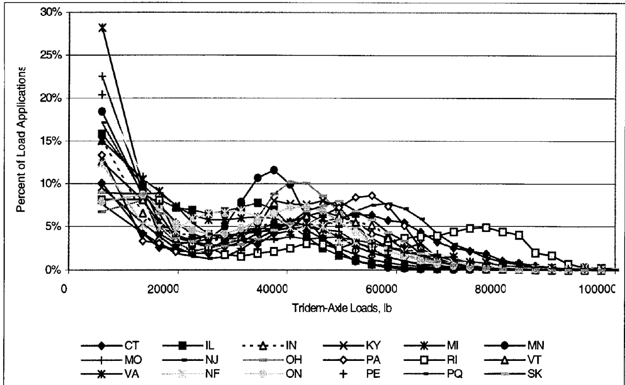
Figure 9. Distribution of tridem-axle loads for the NAR and NCR States/Provinces.
