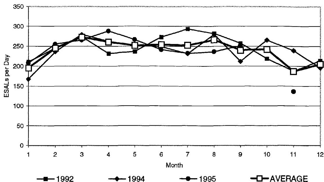
Figure 24. Comparison of monthly ESALs per day variation for Site 12-4000.
