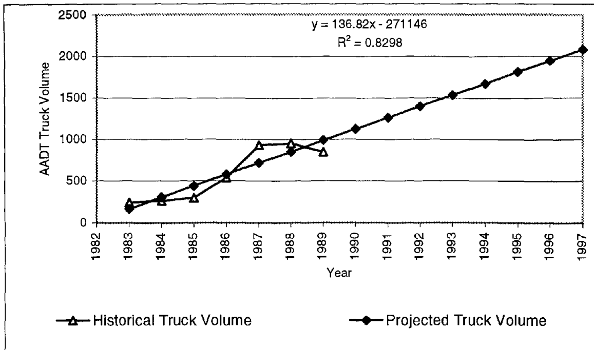
Figure 82. Historical and projected truck AADT volumes for Site 29-4036 for Category 4.
