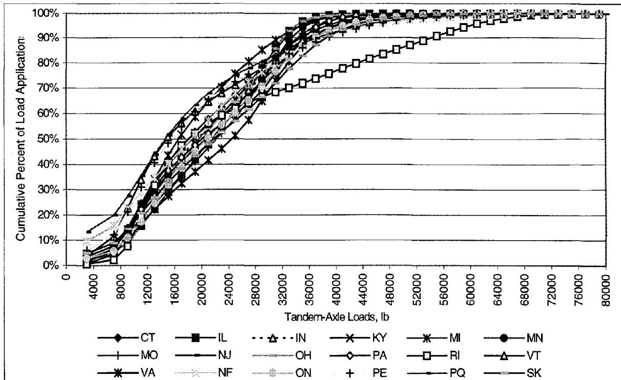
Figure 11. Cumulative distribution of tandem-axle loads for the NAR and NCR States/Provinces.
