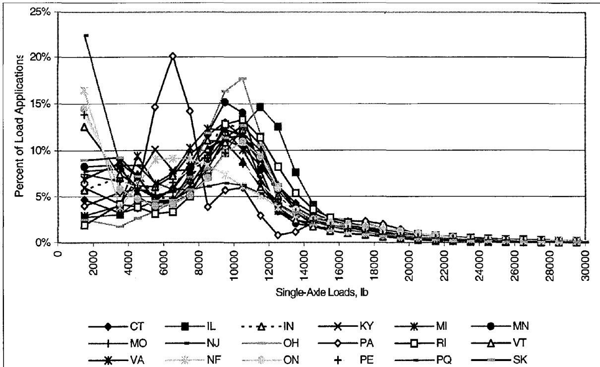
Figure 7. Distribution of single-axle loads for the NAR and NCR States/Provinces.
