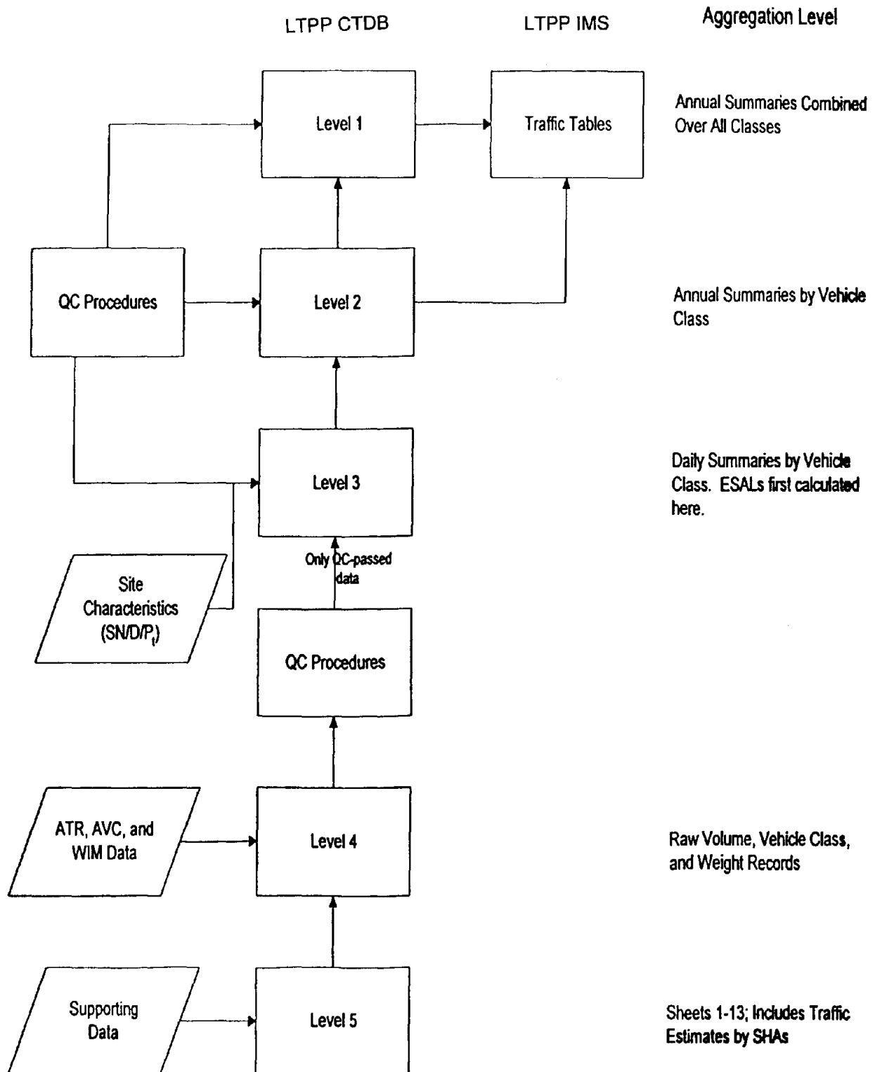
Figure 2. LTPP traffic data levels.
