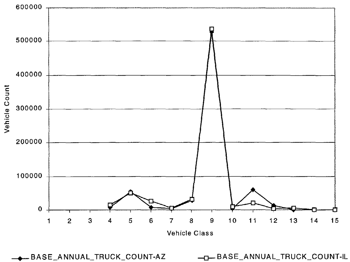
Figure 80. Comparison of truck distribution curves for Arizona and Illinois rural Interstates.
