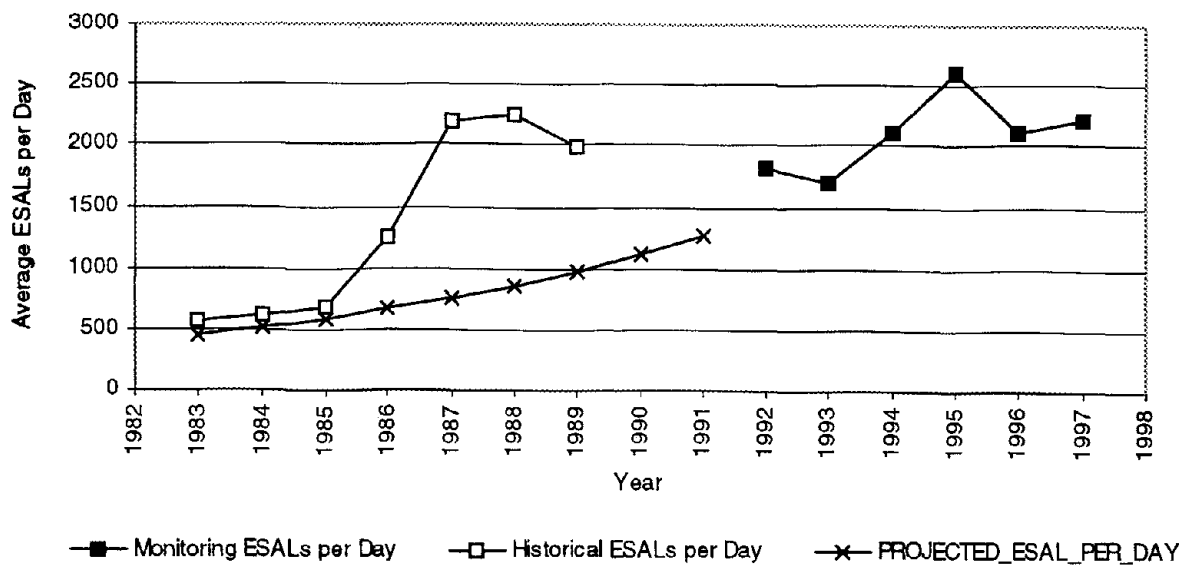
Figure 40. Comparison of ESAL volumes for Site 29-4036.
