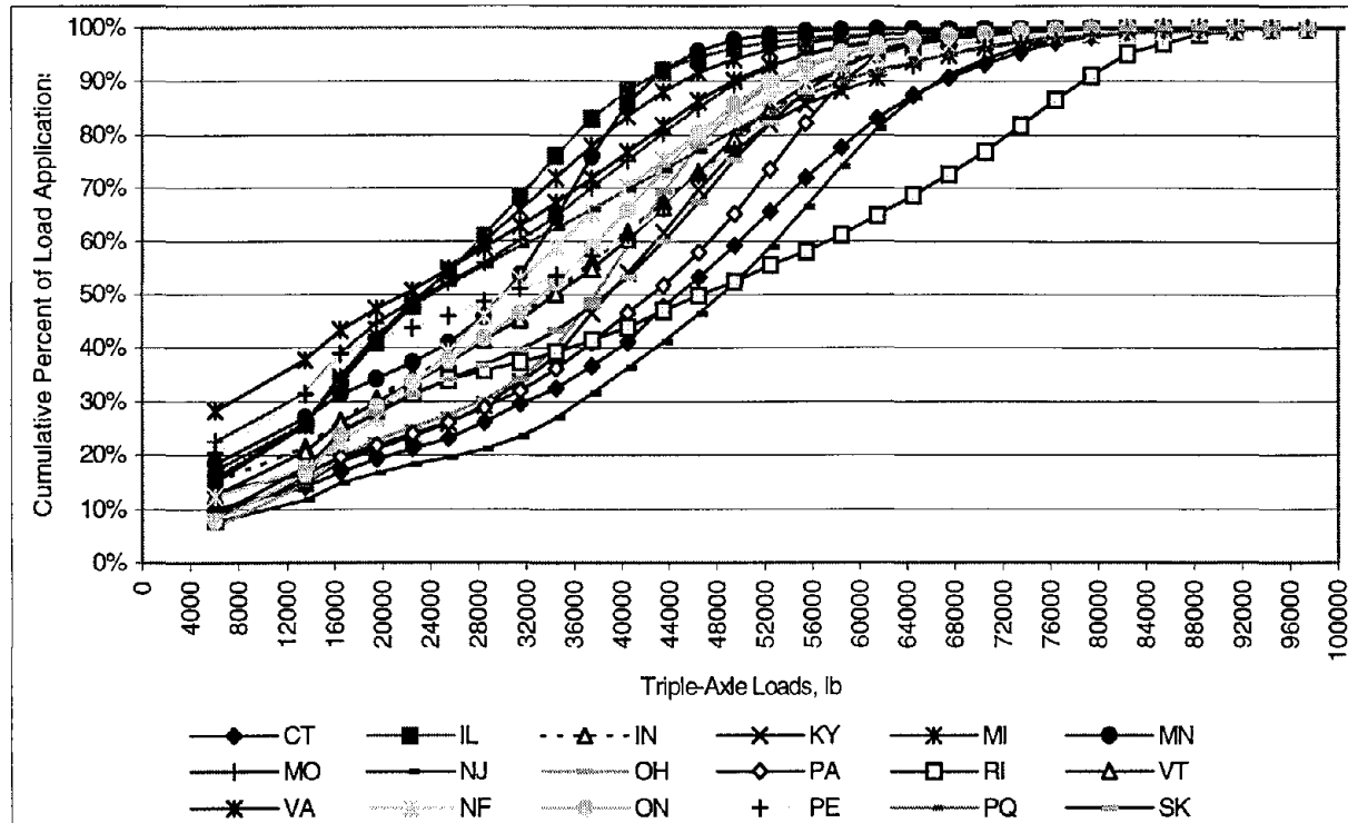
Figure 12. Cumulative distribution of tridem-axle loads for the NAR and NCR States/Provinces.
