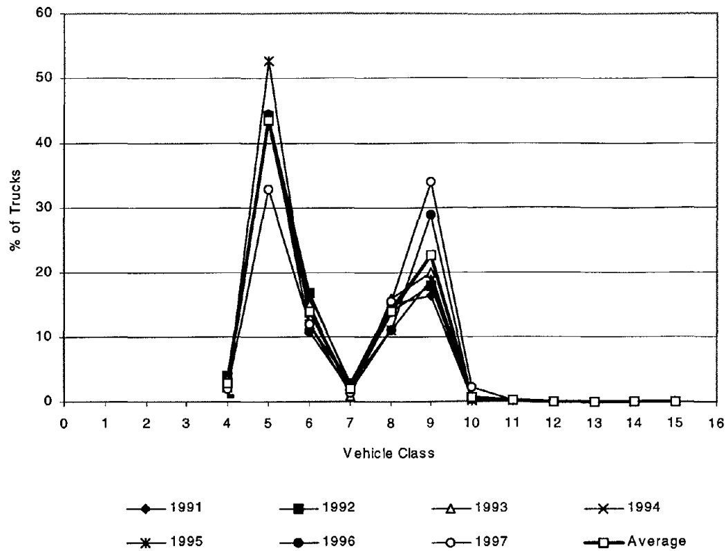
Figure 29. Truck distribution by class for Site 12-4000.
