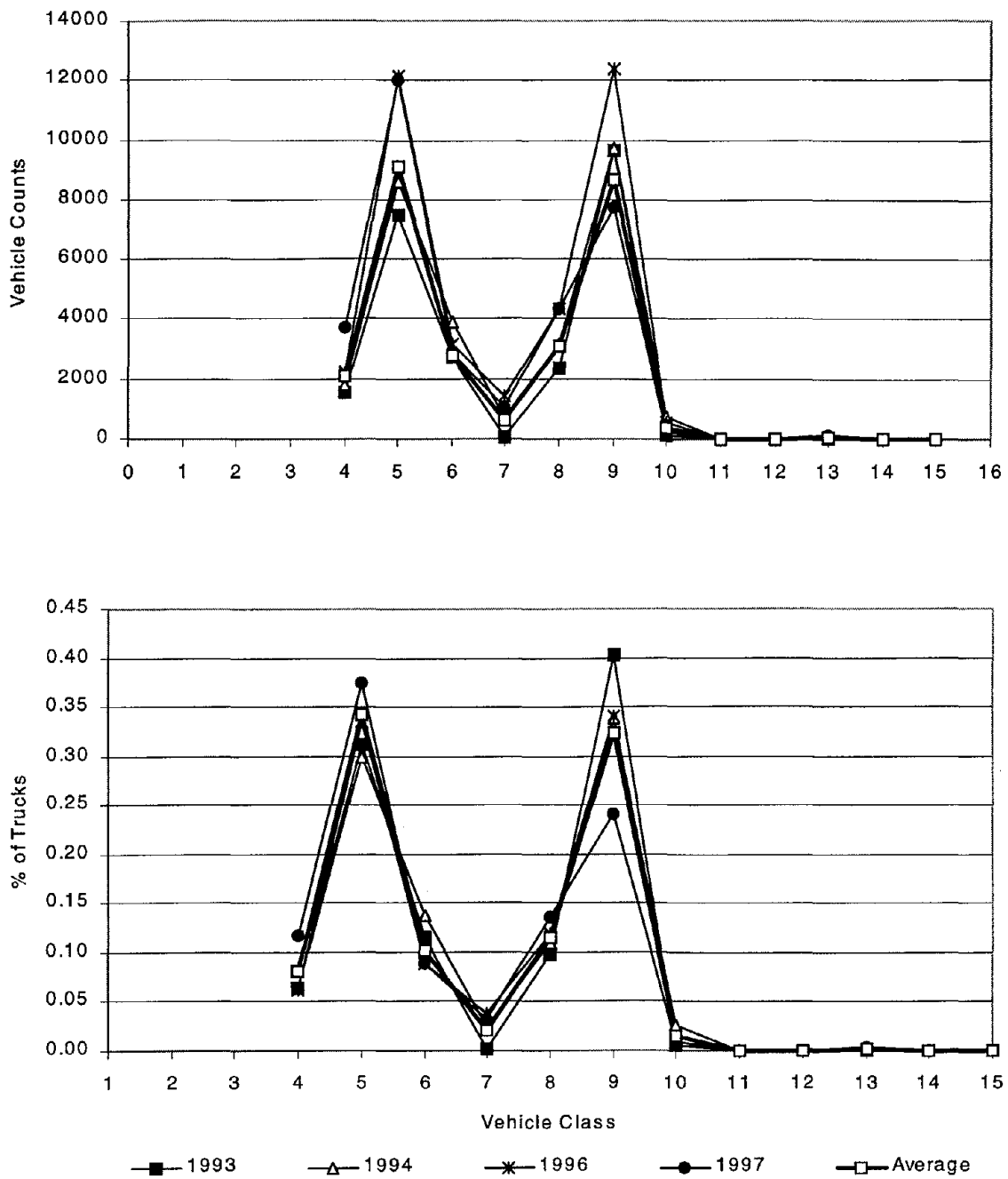
Figure 69. Truck distribution by class for Site 55-3012.
