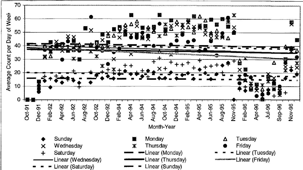
Figure 5. Axle load distributions by day of the week for Class 9 vehicles for Site 12-4000 – tandem-axle loads, 0-142.4 kN (0-31,999 lb), 1991 to 1996.
