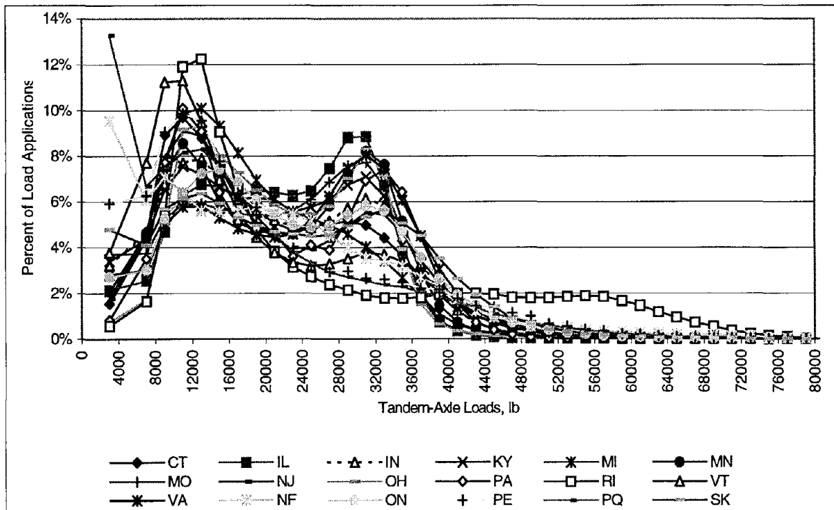
Figure 8. Distribution of tandem-axle loads for the NAR and NCR States/Provinces.
