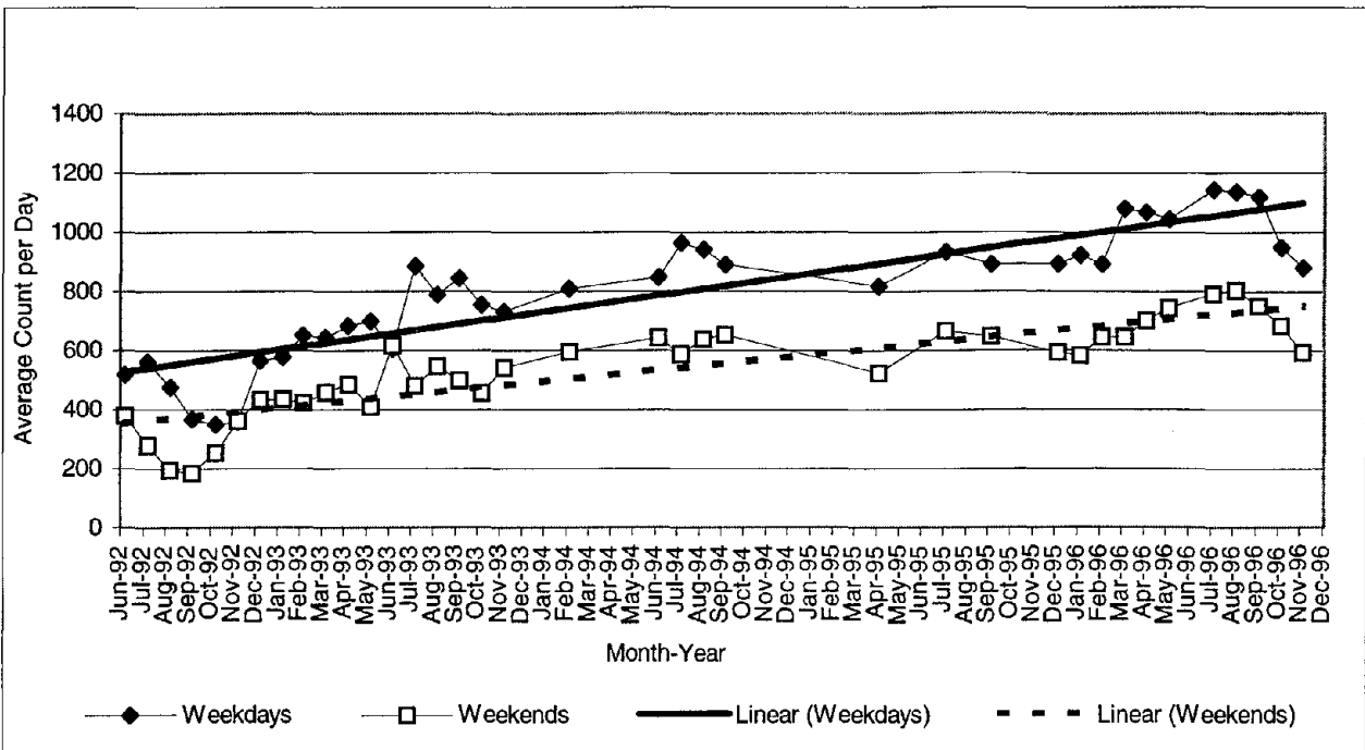
Figure 6. Weekday/weekend axle load counts for Class 9 vehicles for Site 29-4036 – single-axle loads, 0-75.6 kN (0-16,999 lb), 1992 to 1996.
