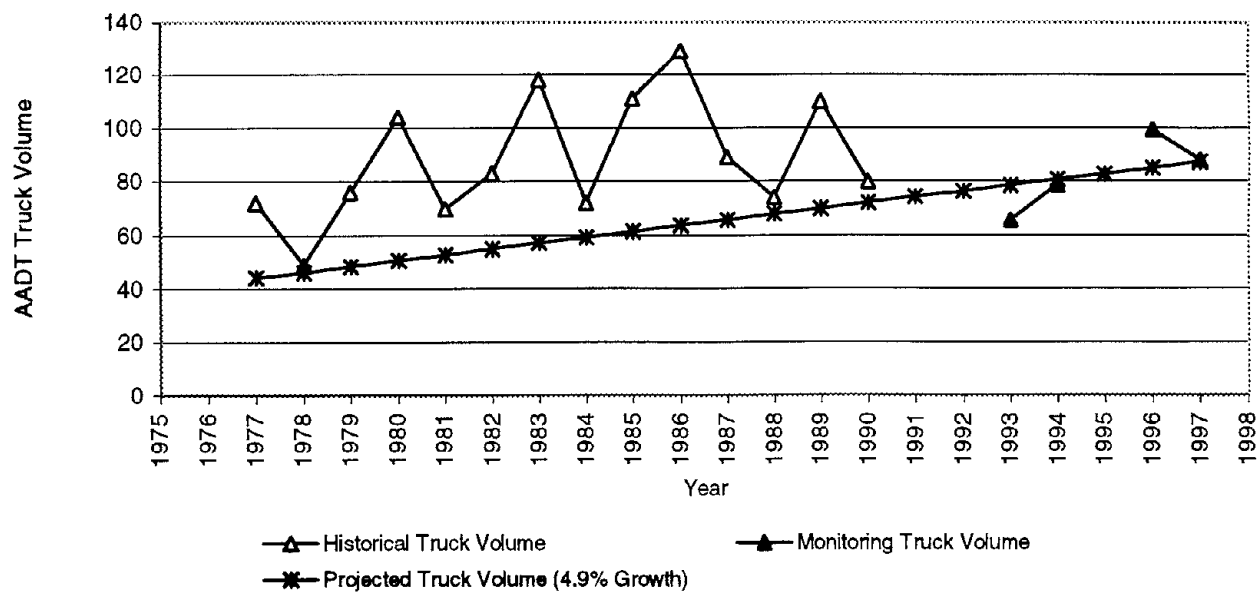
Figure 68. Comparison of truck AADT volumes for Site 55-3012.
