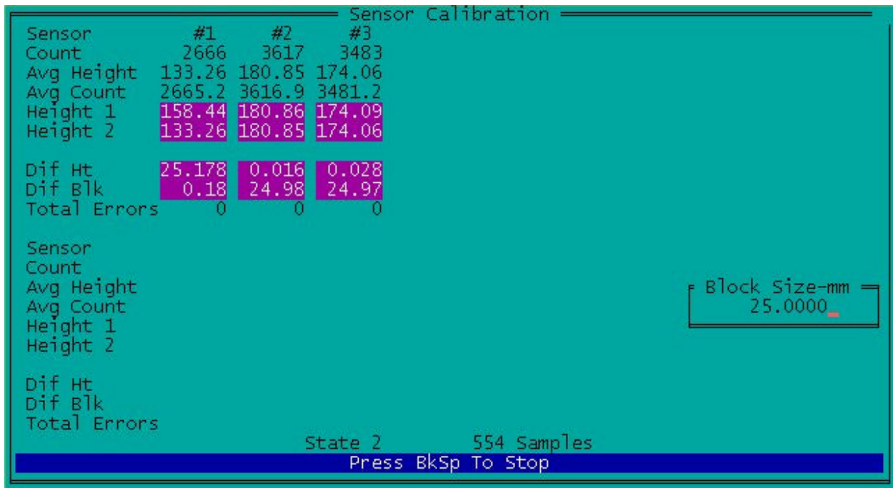
Figure 2.5.4.11. Readings taken with 25 mm block below sensor #1.
