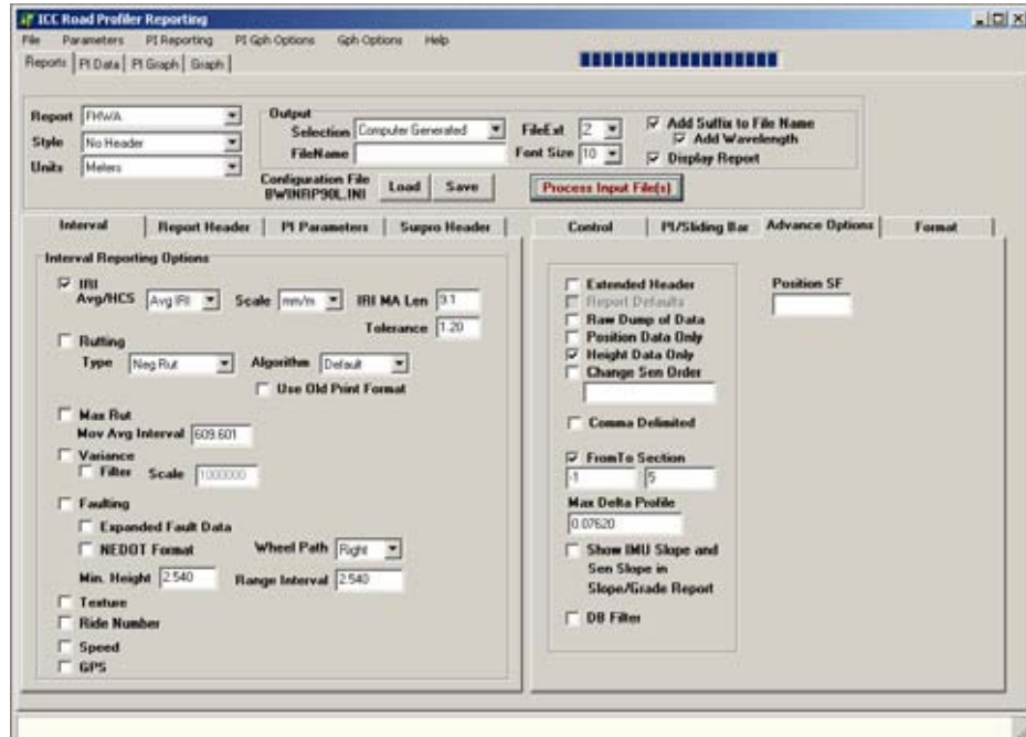
Figure 88. Screen shot. Parameters set in the advanced options tab.
