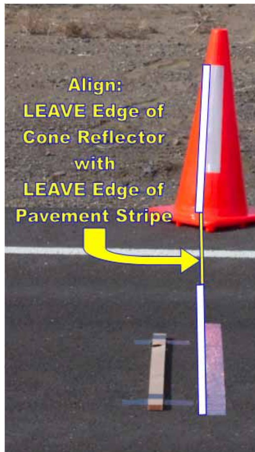
Figure 84. Photo. Placement of vertical photocell target in relation to section starting location.
