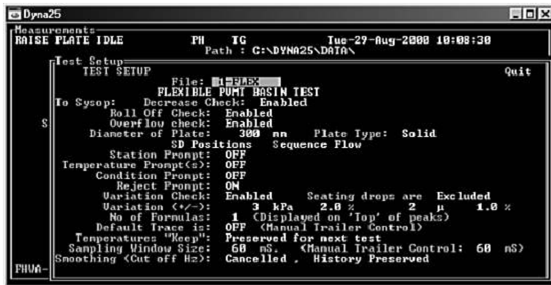
Figure G-1.14 Test Setup - Flexible Pavement Basin Test
