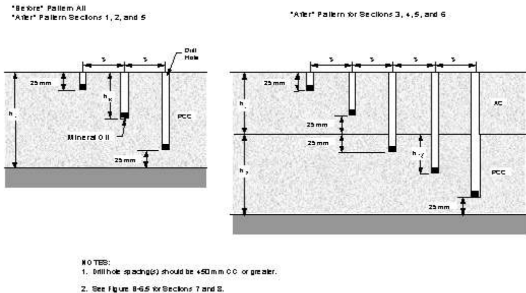
Figure B-6.4 Typical Drilling Pattern for Temperature Gradient Data “Before” and “After”
