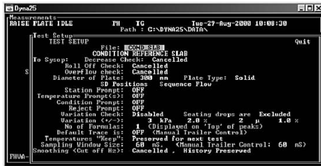
Figure G-1.20 Test Setup - Condition Reference Slab
