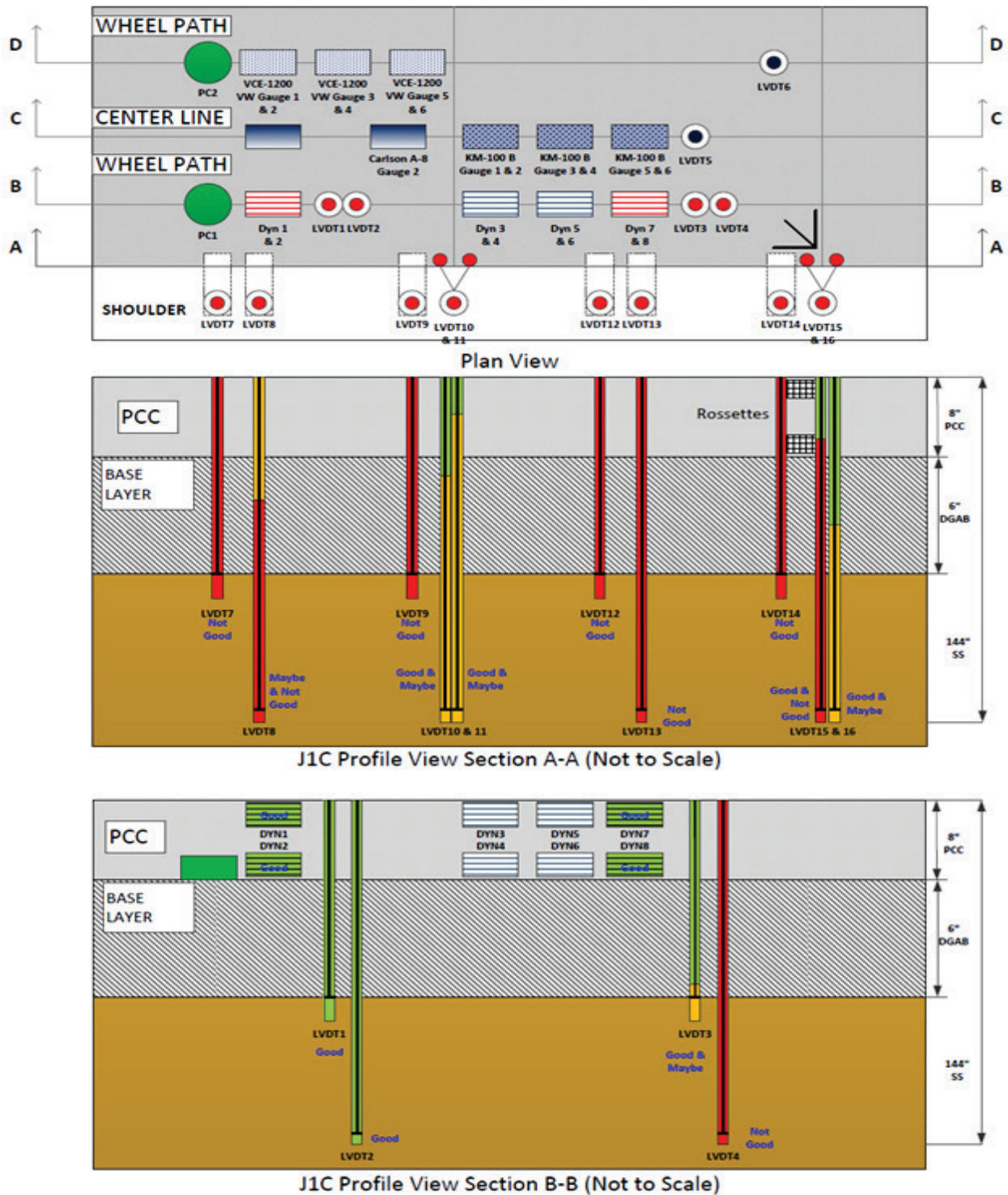
Figure 52. Illustration. QC results by sensor type for test section 390201 test J1C.
