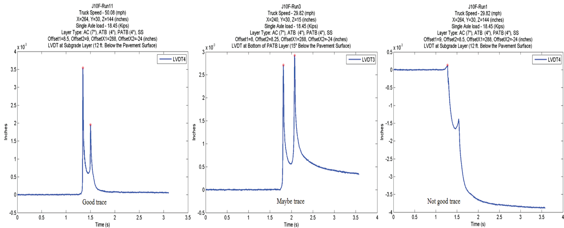
Figure 12. Graph. Ohio SPS-1 LVDT trace categorization.
