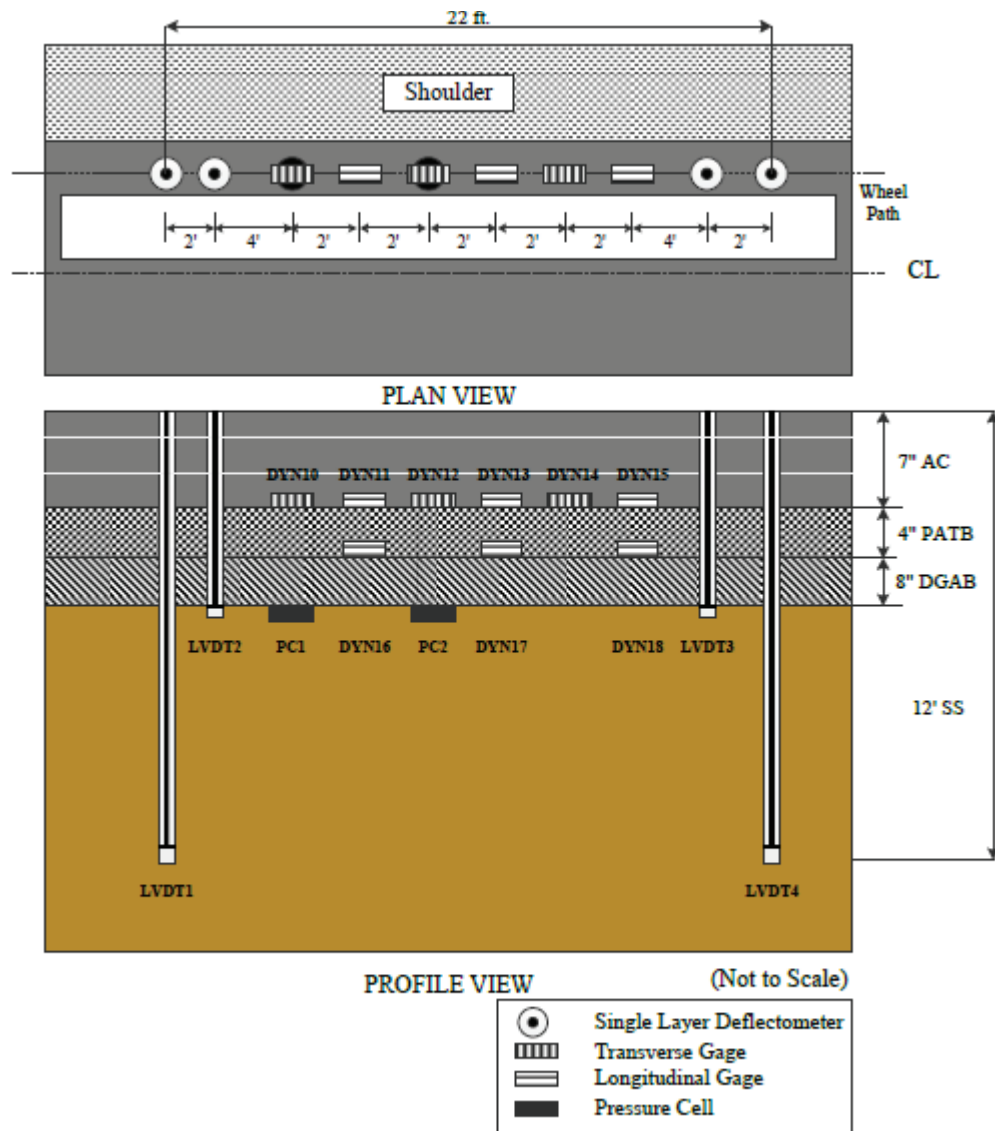
Figure 25. Illustration. Ohio SPS-1 test section 390108 sensor layout.
