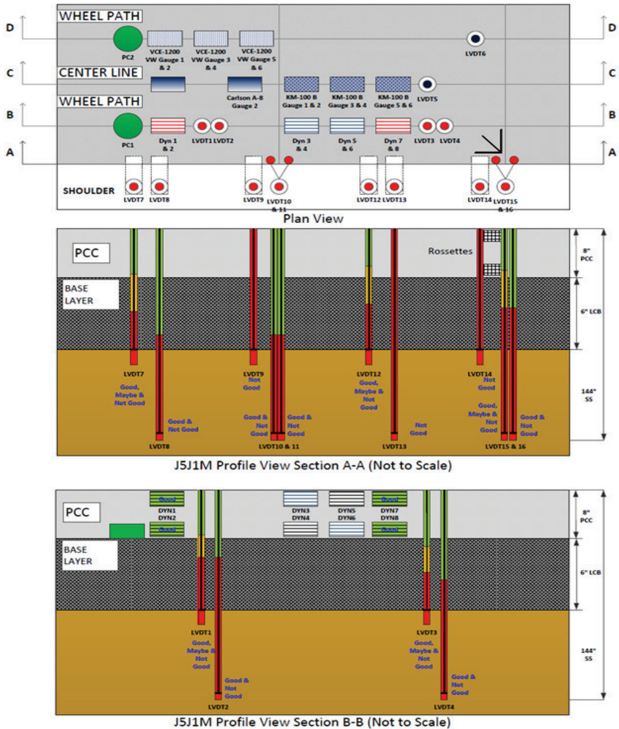
Figure 56. Illustration. QC results by sensor type for test section 390205 test J5J1M.
