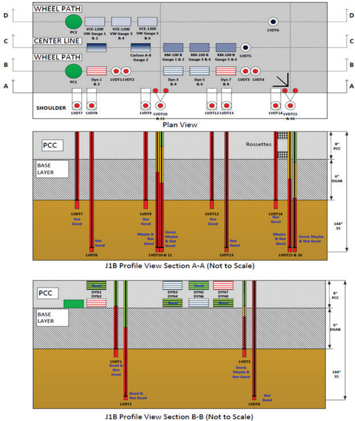
Figure 51. Illustration. QC results by sensor type for test section 390201 test J1B.
