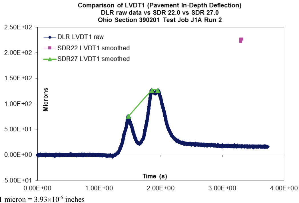
Figure 23. Graph. LVDT1 traces for Ohio test section 390201 test J1A run 2 on August 12, 1996.
