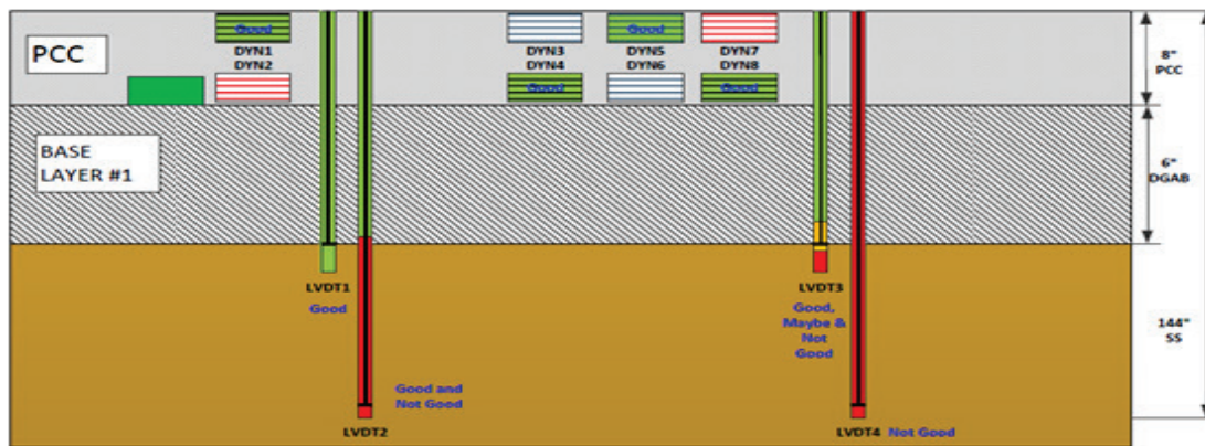
Figure 50. Illustration. QC results by sensor type for test section 390201 test J1A.
