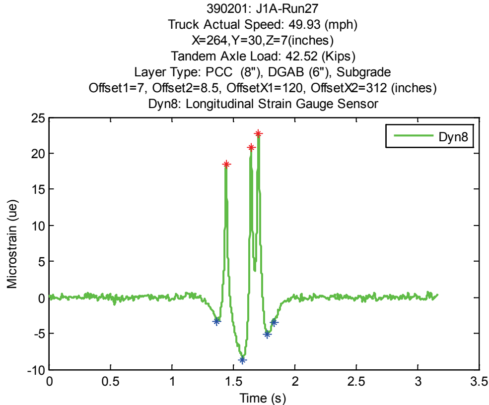
Figure 10. Graph. Extracted trace peaks and valleys from an Ohio SPS-2 test run.
