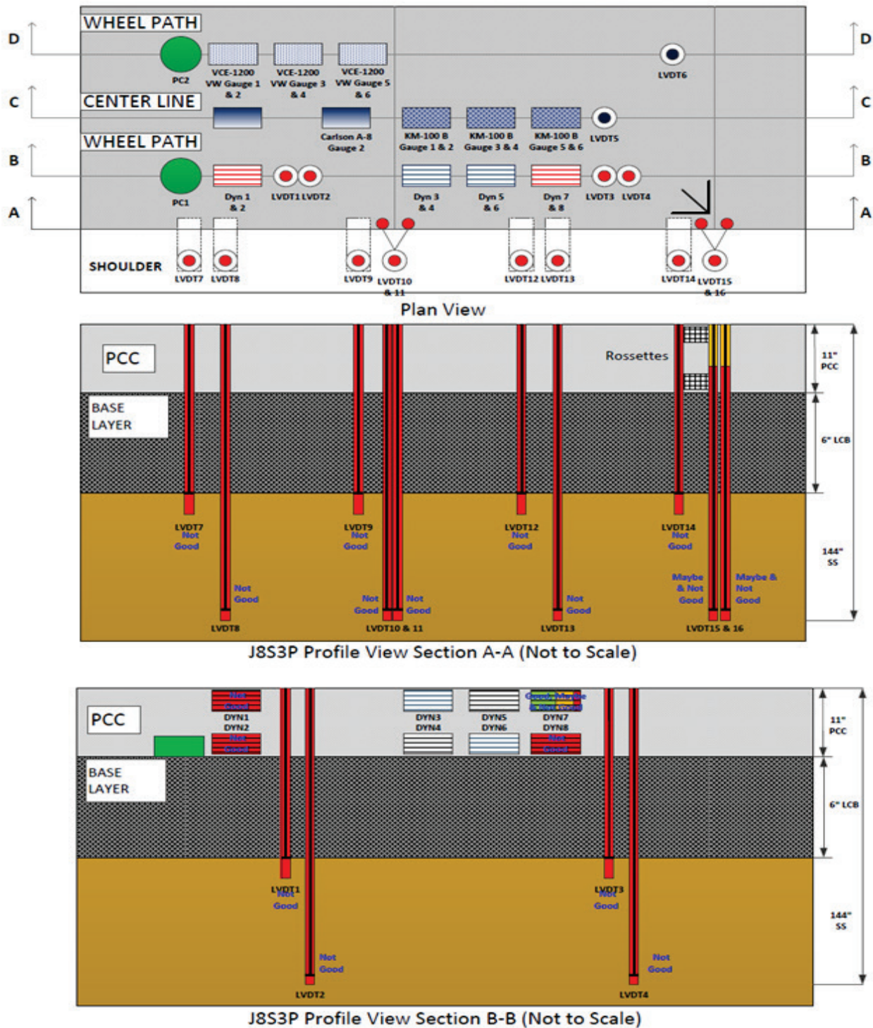
Figure 66. Illustration. QC results by sensor type for test section 390208 test J8S3P.
