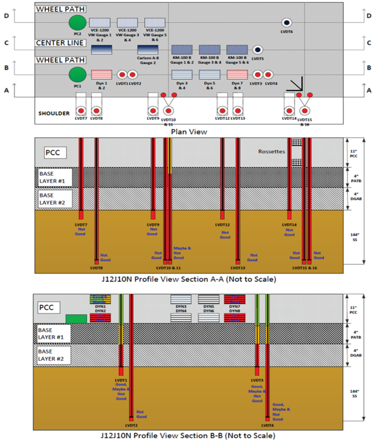
Figure 71. Illustration. QC results by sensor type for test section 390212 test J12J10N.
