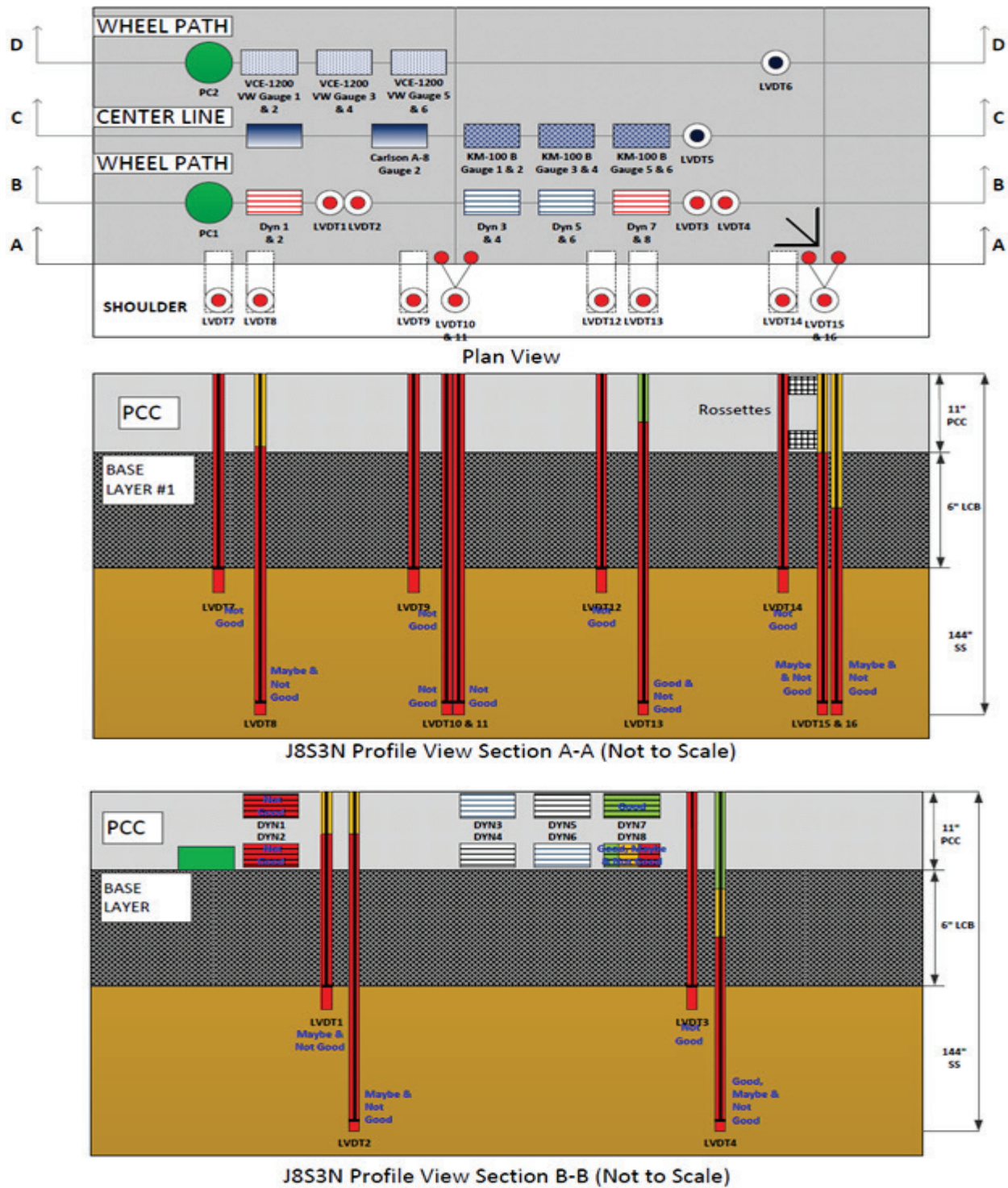
Figure 64. Illustration. QC results by sensor type for test section 390208 test J8S3N.
