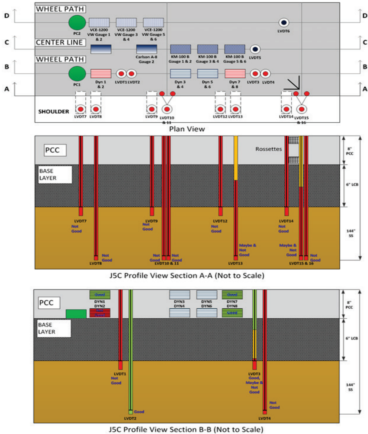
Figure 55. Illustration. QC results by sensor type for test section 390205 test J5C.
