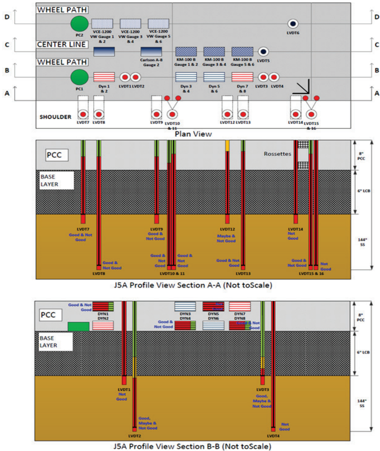
Figure 53. Illustration. QC results by sensor type for test section 390205 test J5A.
