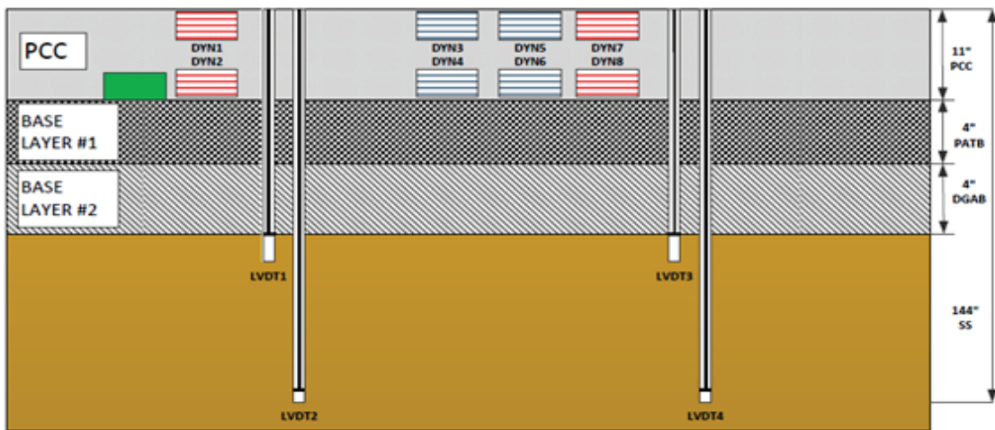
Figure 3. Illustration. Ohio SPS-2 test section 390212 sensor layout.
