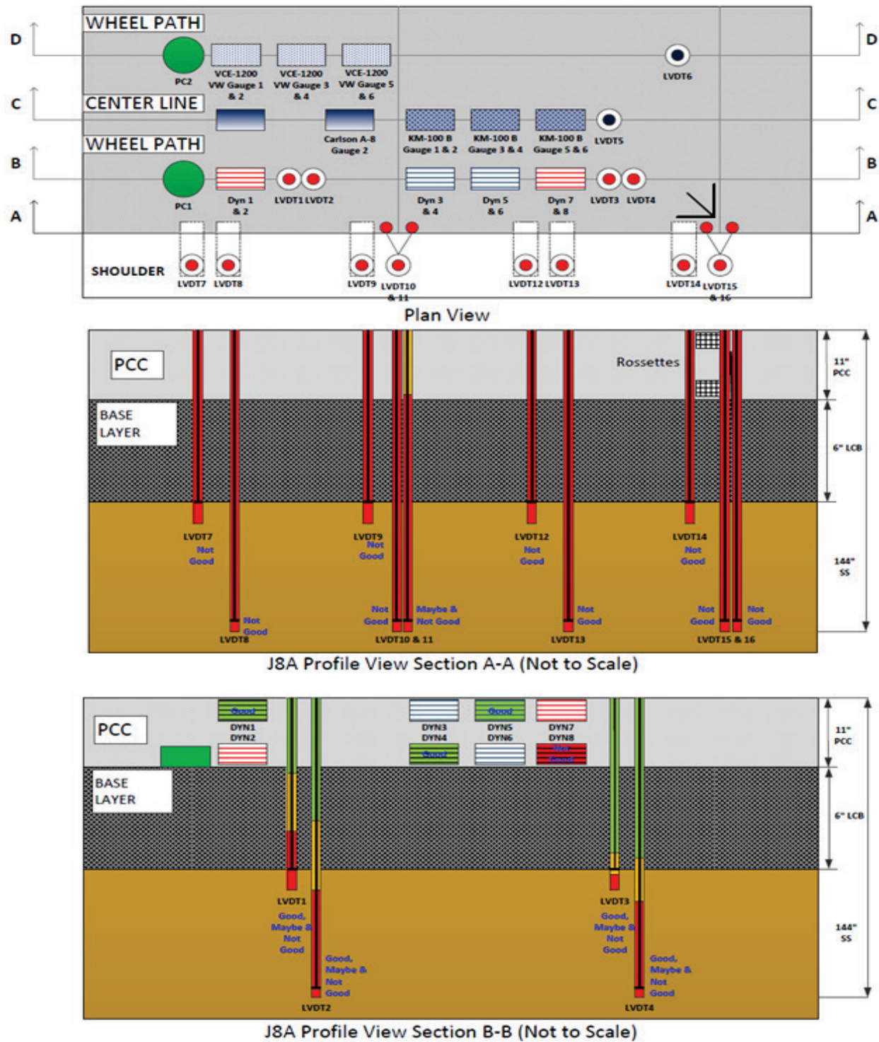
Figure 60. Illustration. QC results by sensor type for test section 390208 test J8A.
