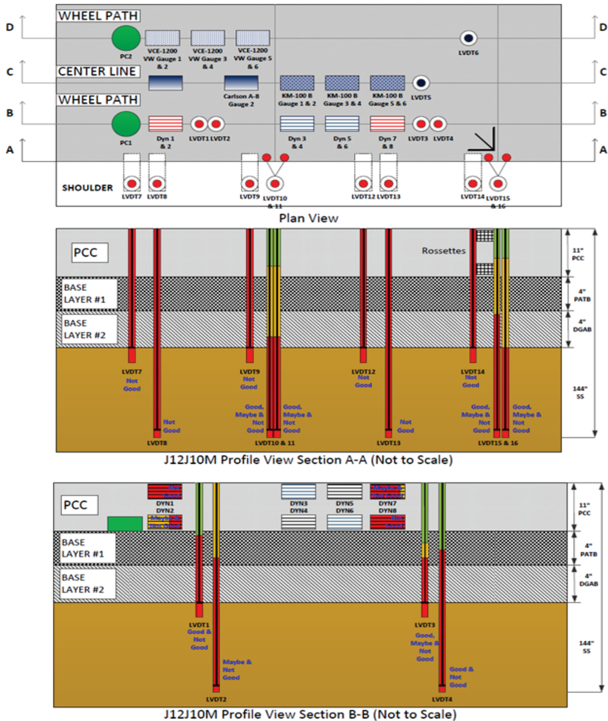
Figure 70. Illustration. QC results by sensor type for test section 390212 test J12J10M.
