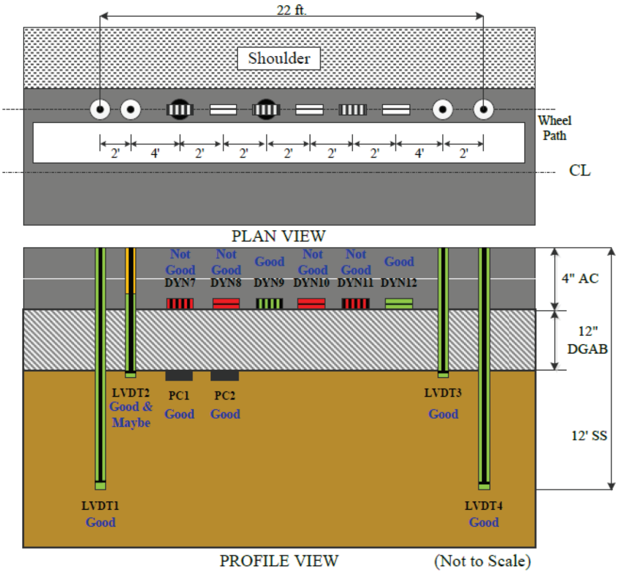
Figure 31. Illustration. QC results by sensor type for test section 390102 test J2F.
