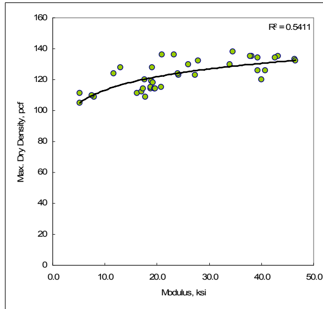
Figure 15. Maximum dry density versus subgrade modulus of coarse-grained soils (1 ksi = 6.89 MPa; 1 pcf = 1 kg/m 3 )
