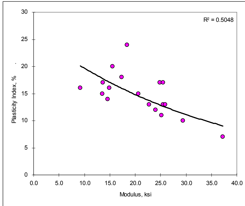
Figure 17. Plasticity index versus subgrade modulus for fine-grained soils (1 ksi = 6.89 MPa)
