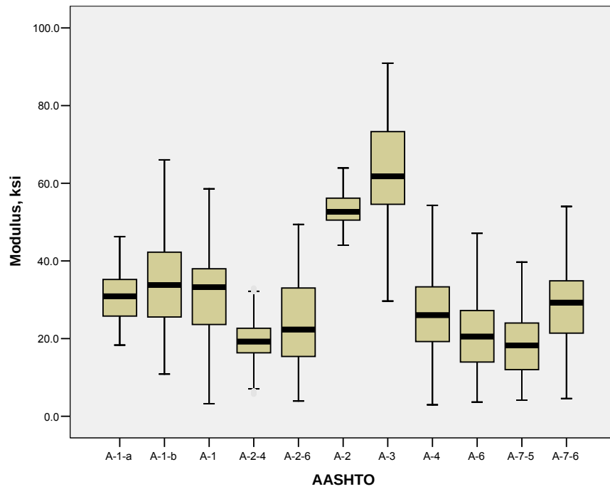
Figure 8. Box Plot of Calculated Subgrade Modulus by Soil Types (1 ksi = 6.89 MPa)
