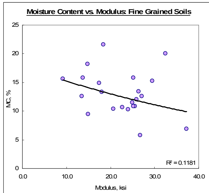
Figure 13. MC (Moisture Content) versus subgrade modulus for fine-grained soils (1 ksi = 6.89 MPa)
