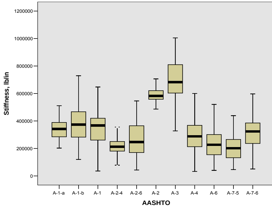
Figure 7. Box Plot of Calculated Subgrade Stiffness by Soil Types (100,000 lb/in = 17.5 MN/m)
