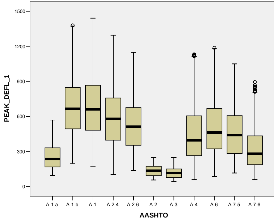
Figure 6. Box Plot of Deflection D1 (PEAK_DEFL_1) Data by Soil Type (deflection in \mu\text{m} )
