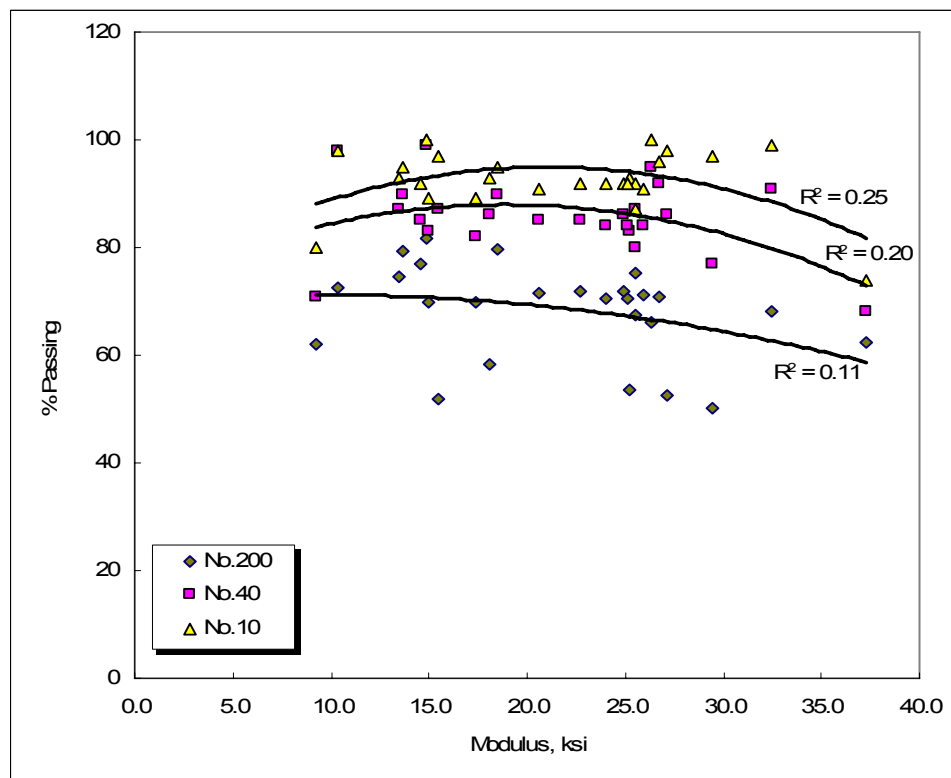
Figure 20. Grain size distribution versus subgrade modulus for fine-grained soils (1 ksi = 6.89 MPa)
