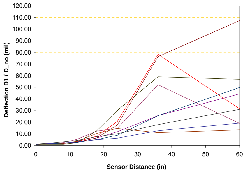
Figure 2. Type II Normalized Deflection Basin (1 in = 2.54 cm, 1 mil = 25.4 \mu\text{m} )
