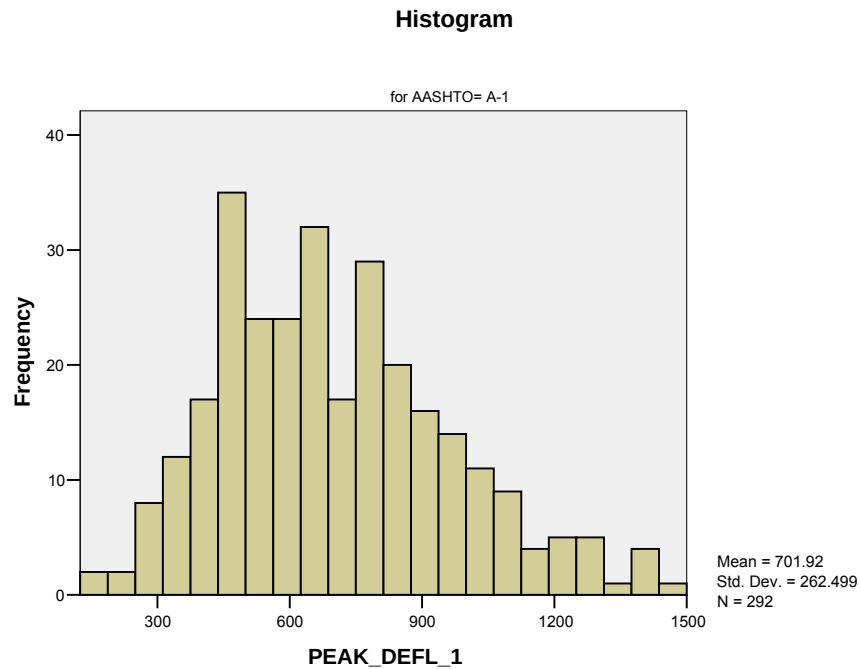
Figure 3. Histogram for deflection (PEAK_DEFL_1) data for A-1 soils (deflection in \mu\text{m} )
