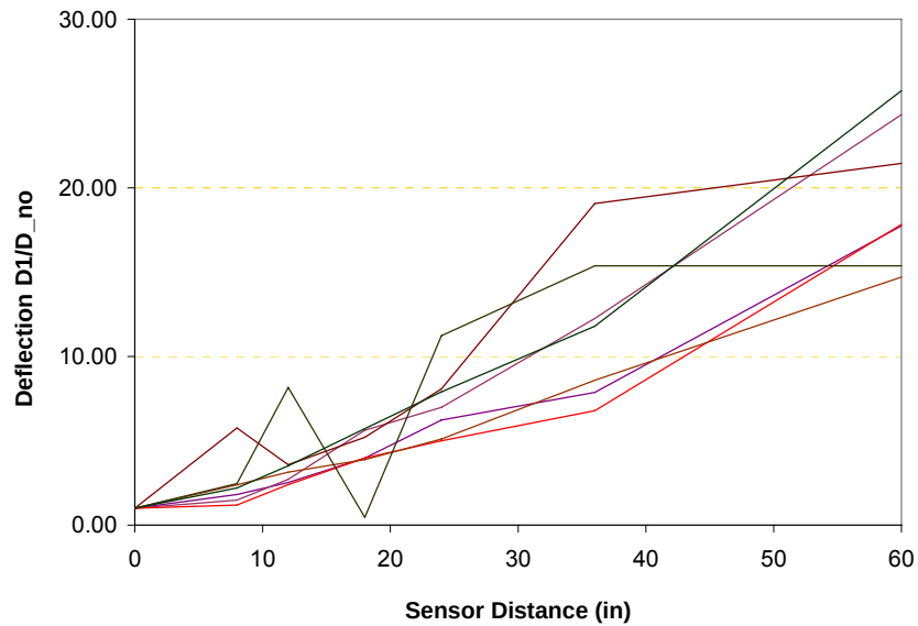
Figure 1. Type I Normalized Deflection Basin (1 in = 2.54 cm, 1 mil = 25.4 \mu\text{m} )
