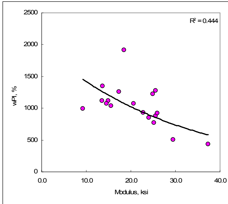
Figure 18. wPI (weighted plasticity index) versus subgrade modulus of fine-grained soils (1 ksi = 6.89 MPa)
