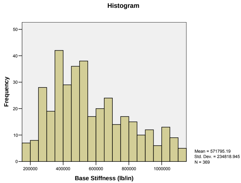
Figure 10. Histogram of base stiffness.
