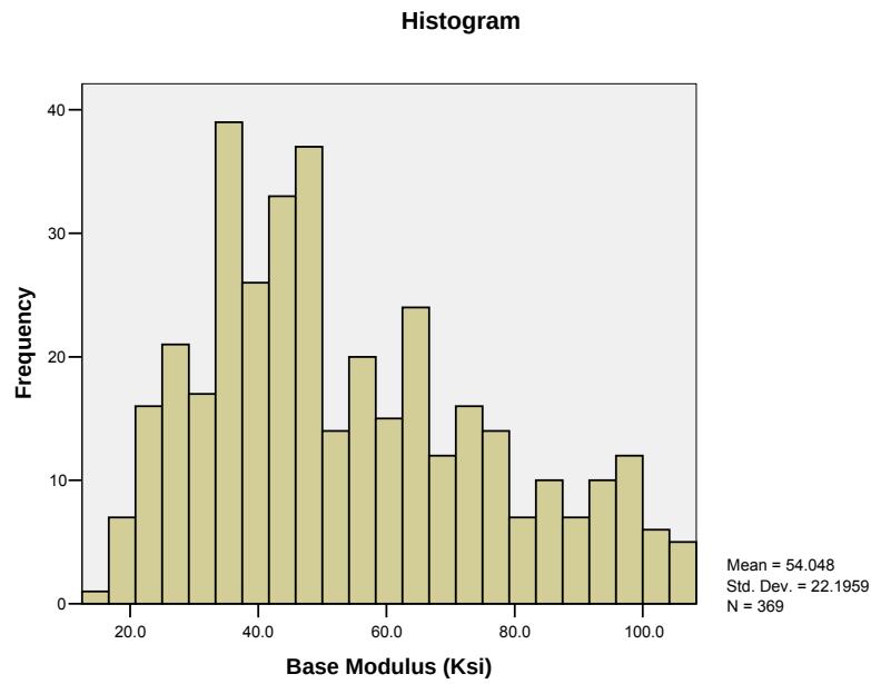
Figure 11. Histogram of base modulus.
