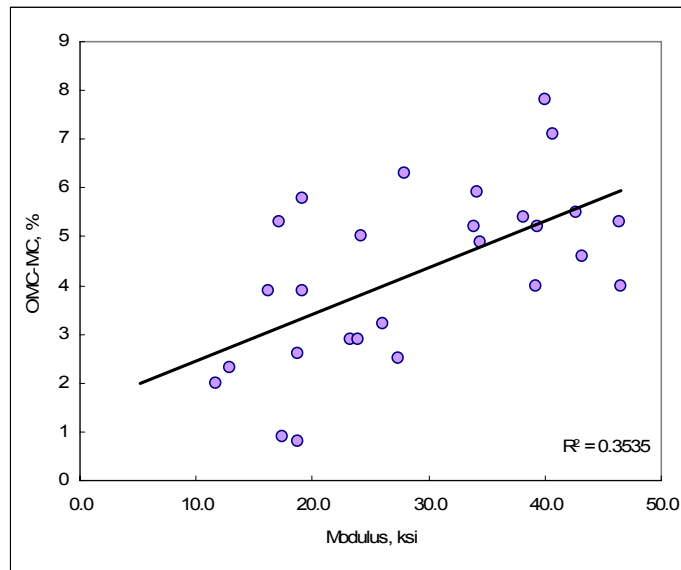
Figure 14. OMC-MC (Optimum Moisture Content – Natural Moisture Content) versus subgrade modulus for coarse-grained soils (1 ksi = 6.89 MPa)
