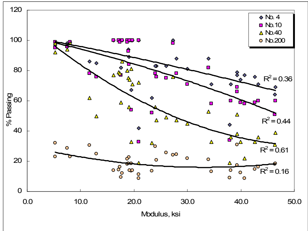
Figure 19. Grain size distribution versus subgrade modulus for coarse-grained soils (1 ksi = 6.89 MPa)
