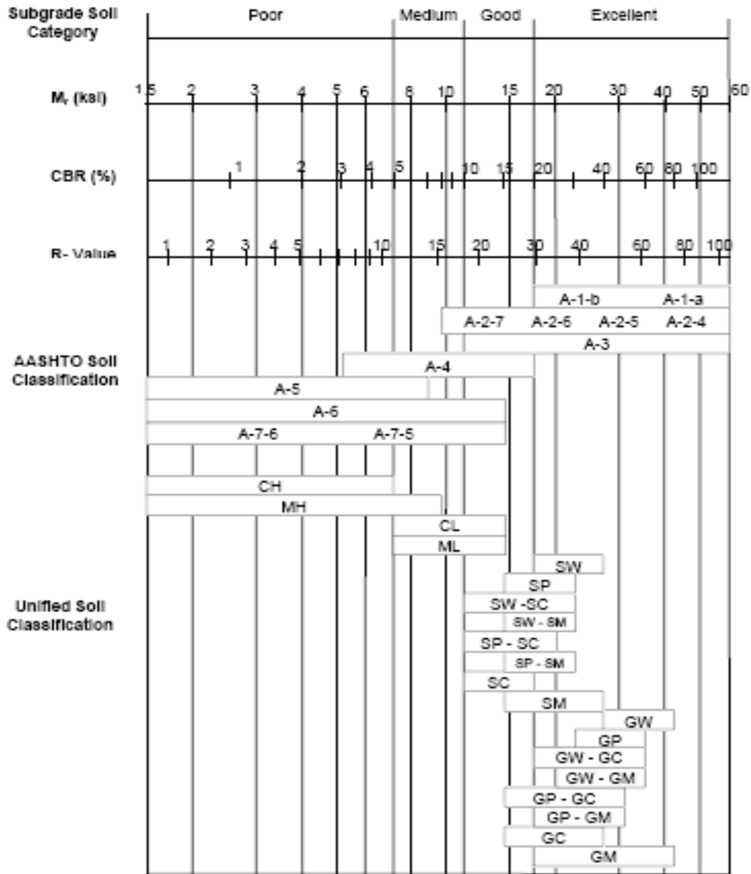
Figure 9. Typical Subgrade Modulus Correlations to Classification Categories (1 ksi = 6.89 MPa) [from ERES Consultants Division, 2004]
