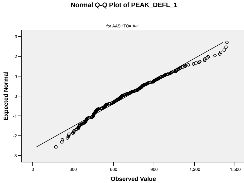
Figure 4. Q-Q plot of deflection data for A-1 soils (observed value of deflection in \mu\text{m} )
