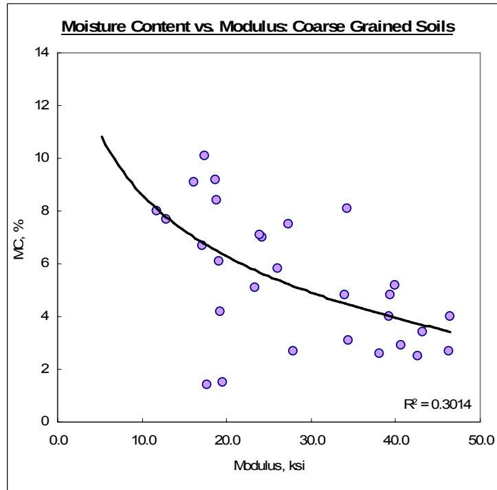
Figure 12. MC (Moisture Content) versus subgrade modulus for coarse-grained soils (1 ksi = 6.89 MPa)
