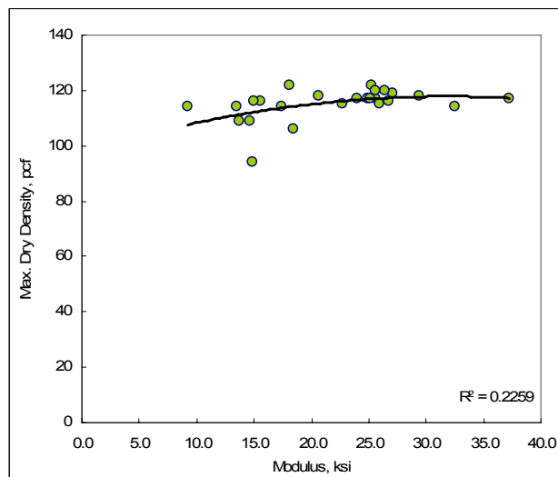
Figure 16. Maximum dry density versus subgrade modulus of fine-grained soils (1 ksi = 6.89 MPa; 1 pcf = 1 kg/m 3 )
