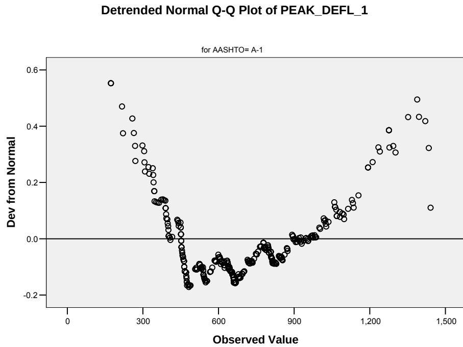
Figure 5. Detrended Q-Q plot of deflection data for A-1 soils (observed value of deflection in \mu\text{m} )
