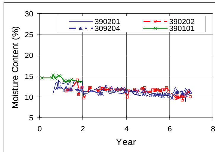
Figure 8. Moisture Variations in OH AC Section (390101) and JCP Sections (390201, 390202 and 390204) on GB
