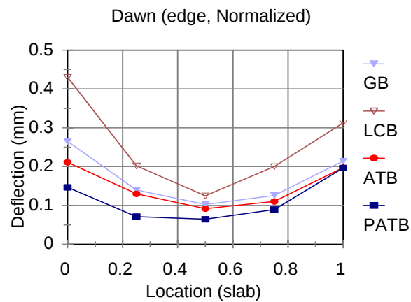
Figure 24. Edge of Slab Deflection, Dawn (1 mm = 39.37 mil)
