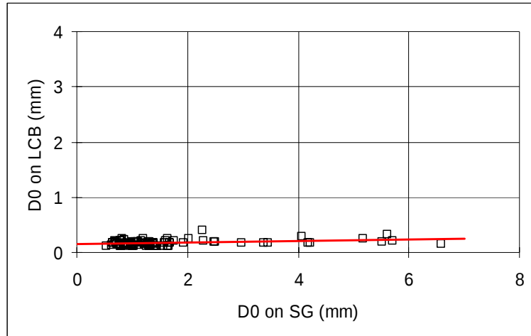
Figure 18. Lean Concrete Base Deflection Comparison (1 mm = 39.37 mil)
