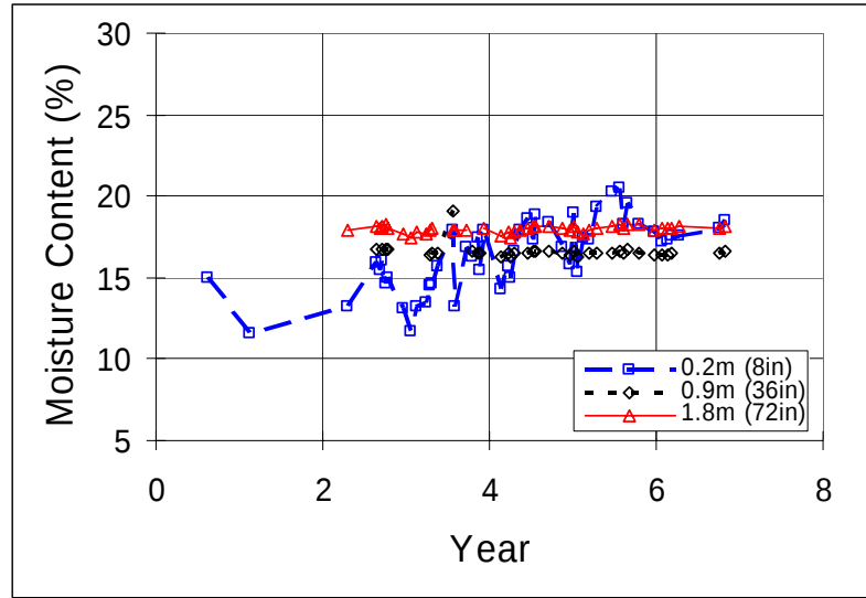
Figure 7. Annual Moisture Cycles at Different Depths in Ohio Section 390208 with LCB
