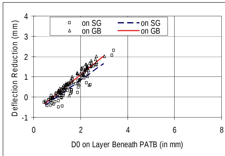
Figure 20. PATB Deflection Reduction (1 mm = 39.37 mil)
