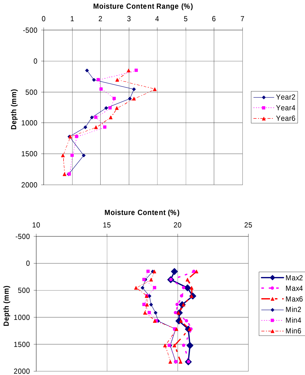
Figure 3. Range of Moisture Content Variation and Max/Min Moisture Content as a Function of Depth (Ohio Section 390104 ATB) (100 mm = 3.94 in)
