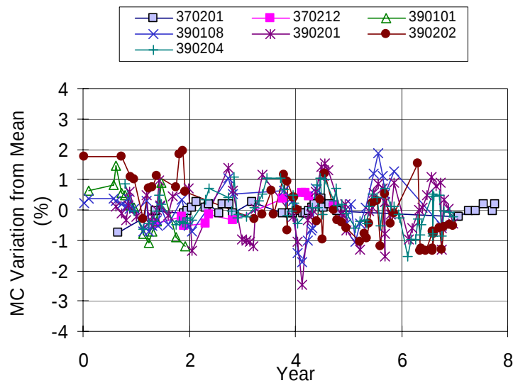
Figure 11. Moisture Deviations from the Mean on NC and OH GB Sections
