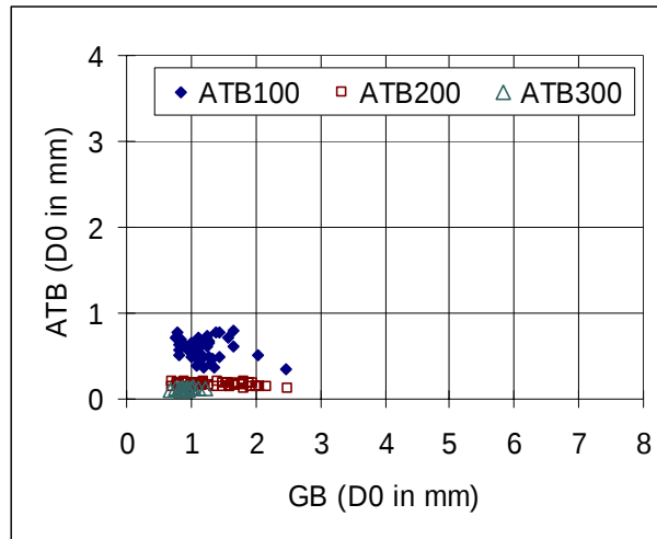
Figure 21. ATB Deflection Comparison (1 mm = 39.37 mil)
