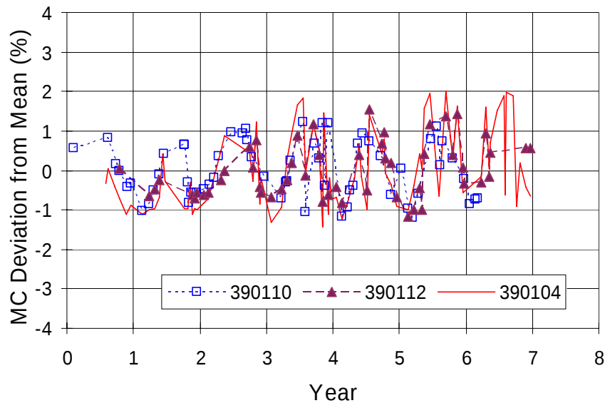
Figure 13. Moisture Deviations from the Mean on OH Sections with PATB (390110 and 390112) and ATB (390104)
