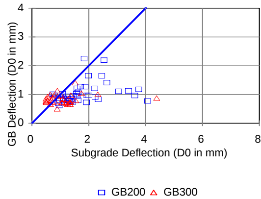
Figure 16. Thick Granular Base Deflection Comparison (1 mm = 39.37 mil)
