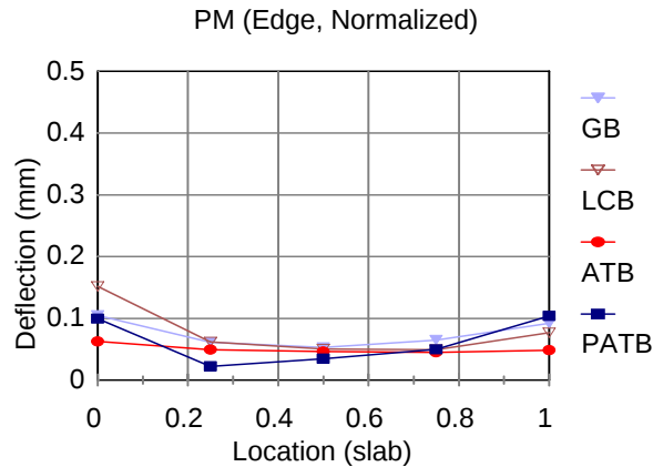
Figure 25. Edge of Slab Deflection, Mid Afternoon (1 mm = 39.37 mil)
