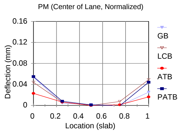
Figure 23. Center of Lane Deflection, Mid Afternoon (1 mm = 39.37 mil)
