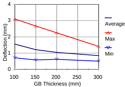
Figure 17. Average Deflection of GB with Different Thicknesses (1 mm = 39.37 mil)
