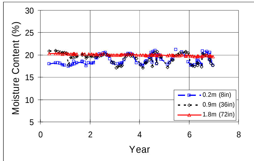
Figure 6. Annual Moisture Cycles at Different Depths in Ohio Section 390205 with LCB
