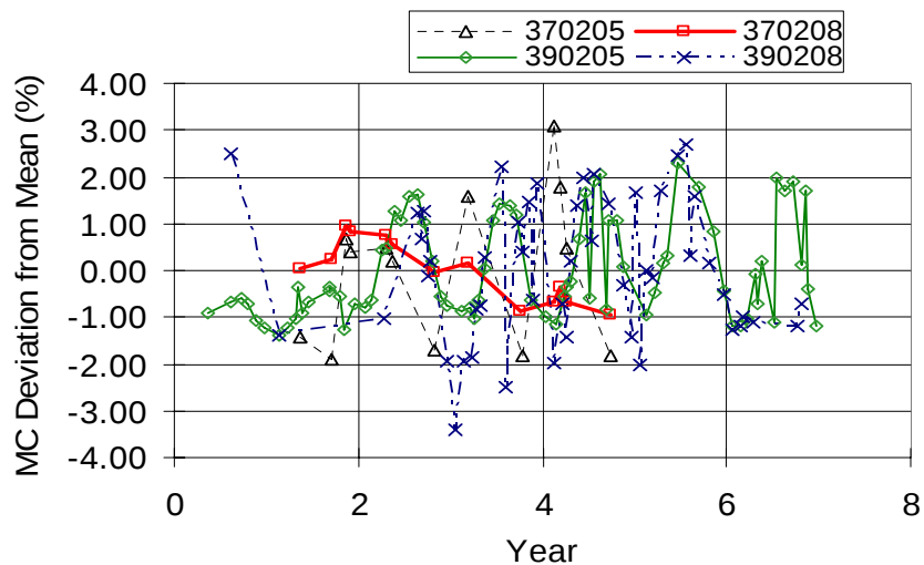
Figure 12. Moisture Deviations from the Mean on NC and OH LCB Sections
