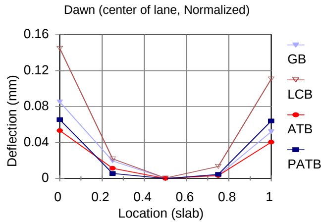
Figure 22. Center of Lane Deflection, Dawn (1 mm = 39.37 mil)
