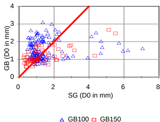
Figure 15. Thin Granular Base Deflection Comparison (1 mm = 39.37 mil)
