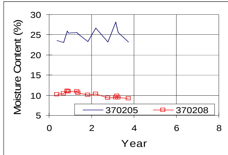
Figure 10. Moisture Variations in NC Sections 370205 and 370208 with LCB
