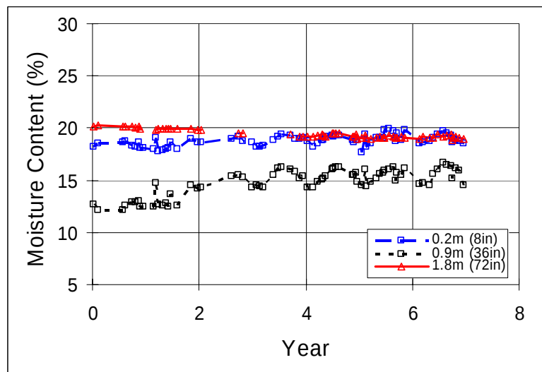
Figure 9. Moisture Variations in OH Section 390108 with PATB and GB
