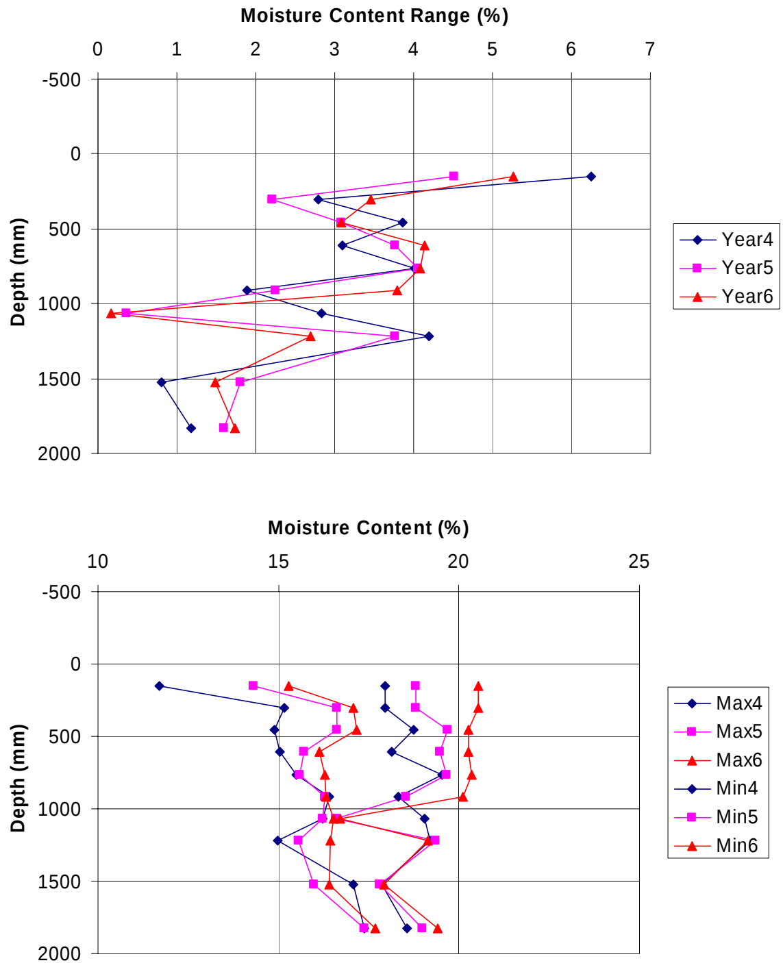
Figure 4. Range of Moisture Content Variation and Max/Min Moisture Content as a Function of Depth (Ohio Section 390208 LCB) (100 mm = 3.94 in)
