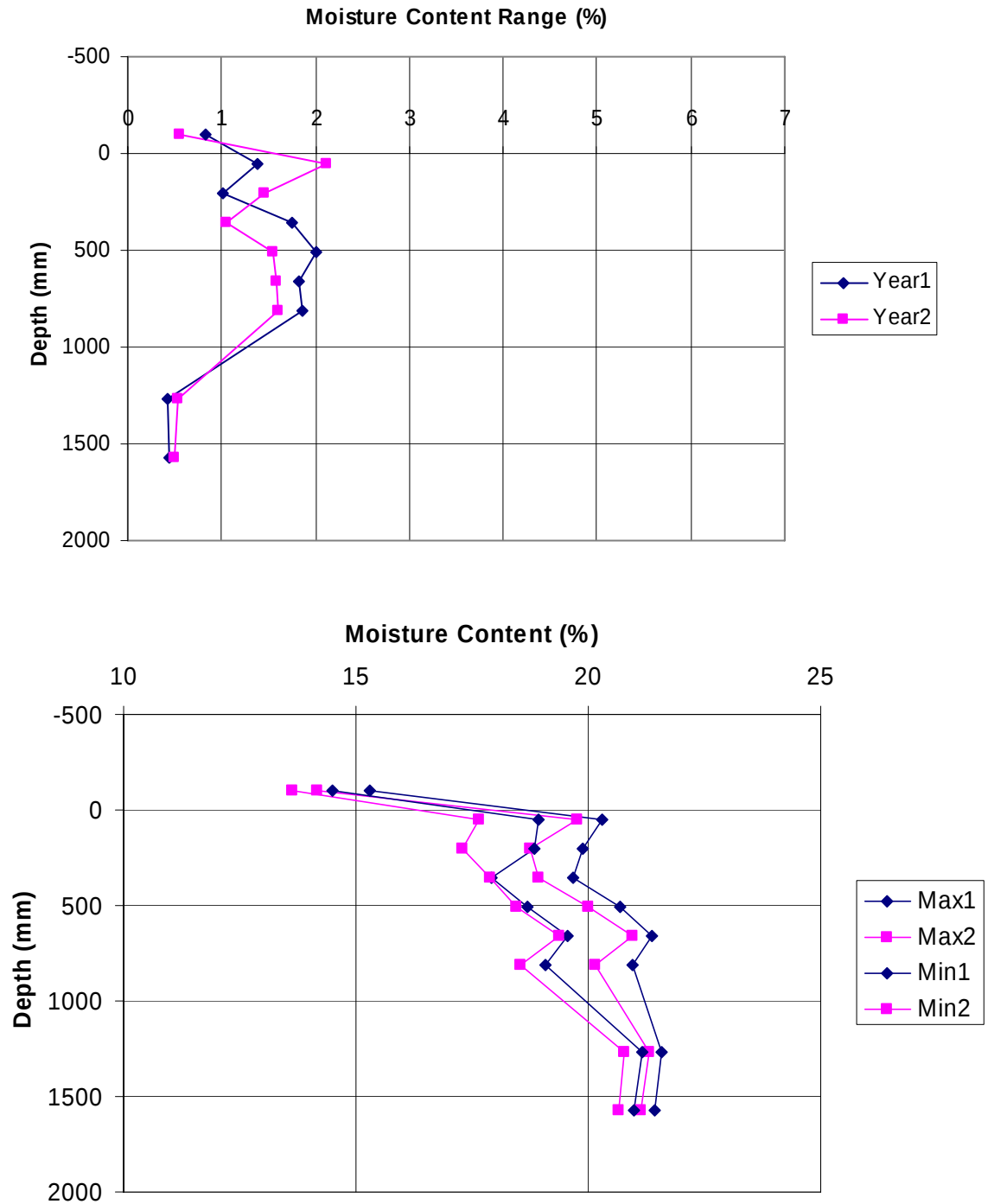
Figure 2. Range of Moisture Content Variation and Max/Min Moisture Content as a Function of Depth (Ohio Section 390101 GB) (100 mm = 3.94 in)
