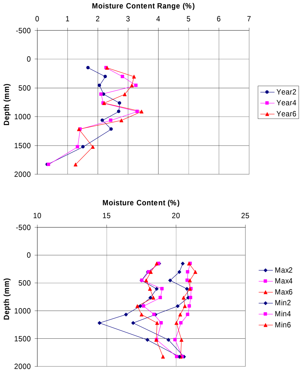
Figure 5. Range of Moisture Content Variation and Max/Min Moisture Content as a Function of Depth (Ohio Section 390110 PATB) (100 mm = 3.94 in)
