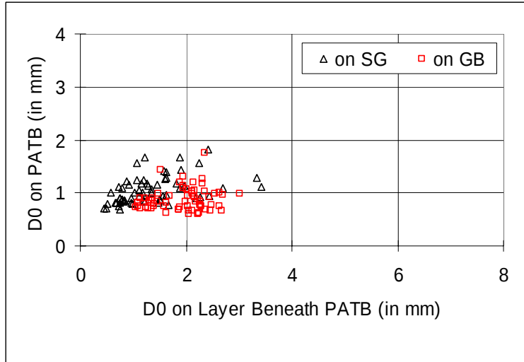
Figure 19. PATB Deflection Comparison (1 mm = 39.37 mil)
