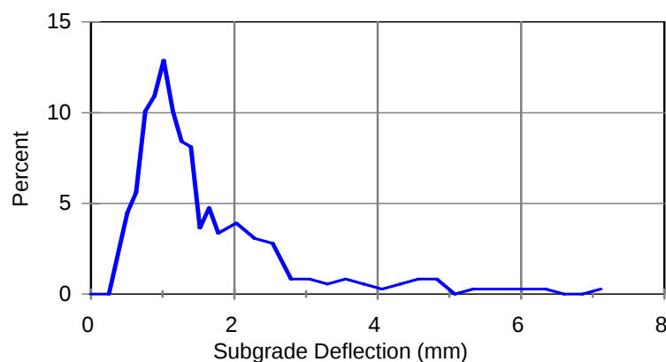
Figure 14. Subgrade Deflection Distribution for Ohio sections. (1 mm = 39.37 mil)
