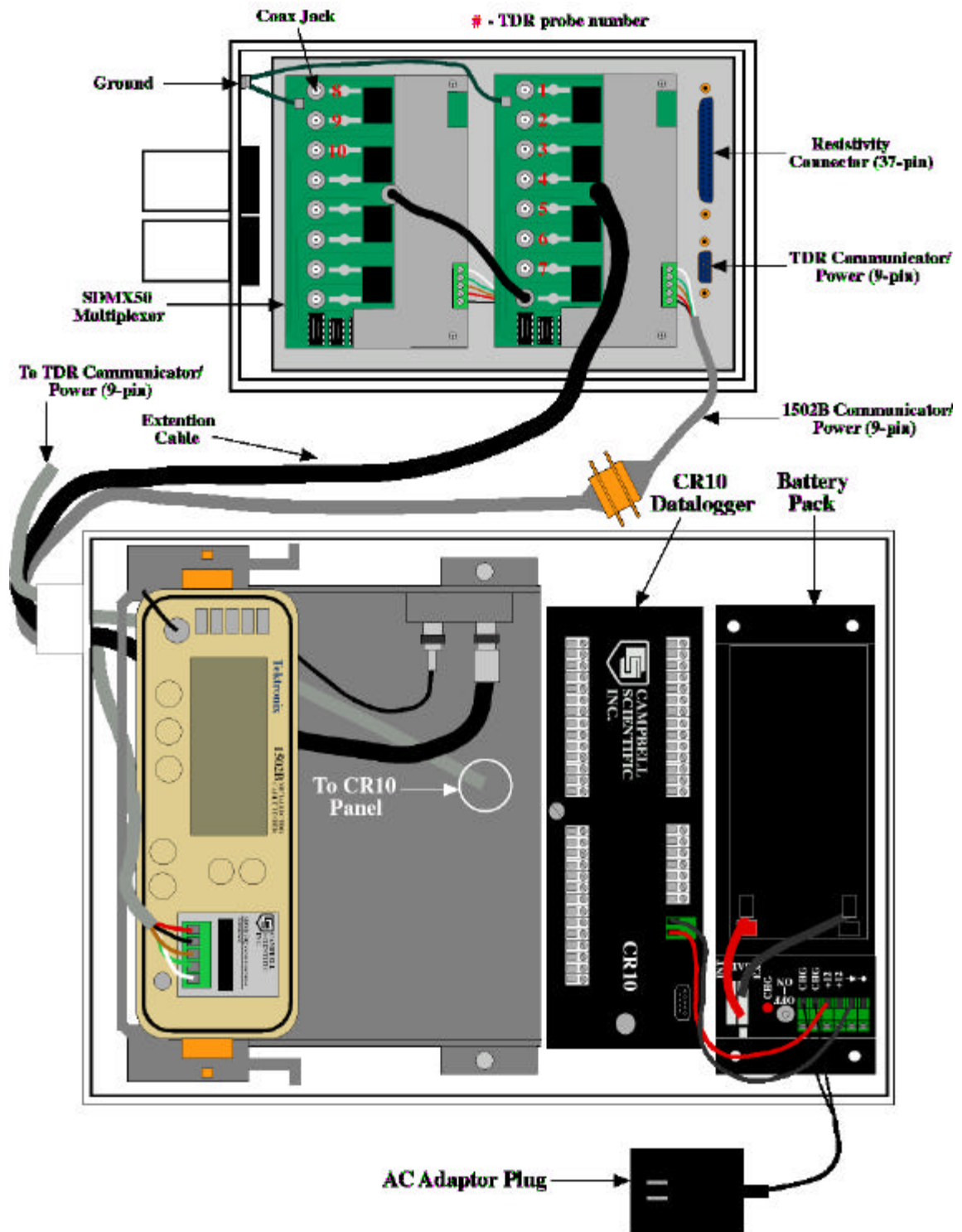
Figure 4.3 Mobile System
