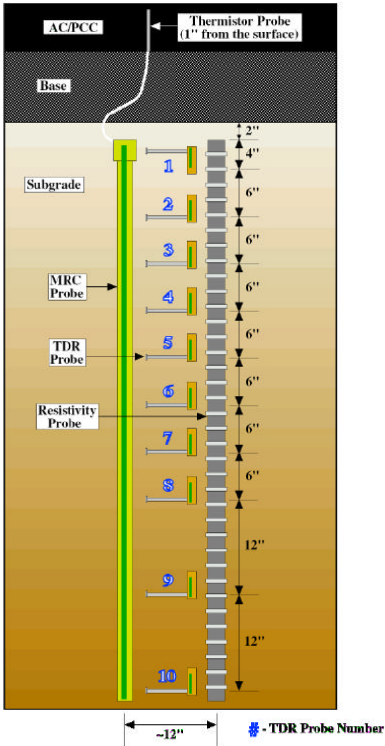
Figure 3.11 Environmental Instrumentation Layout
