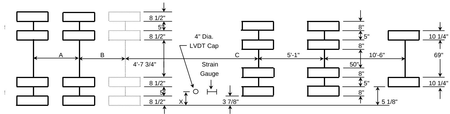
Tire Coverage of Pavement Sensors
