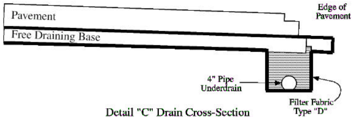
Figure 8.1 Drain Types
