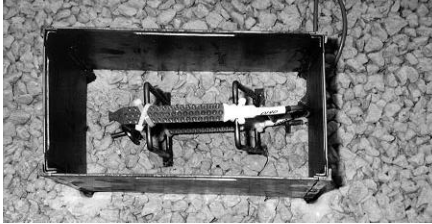
Figure 12.13 Micro Measurement EGP-5-120 Gauge Setup
