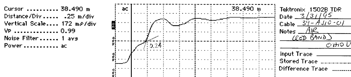
Figure 3.9 TDR Probe in Air Calibration
