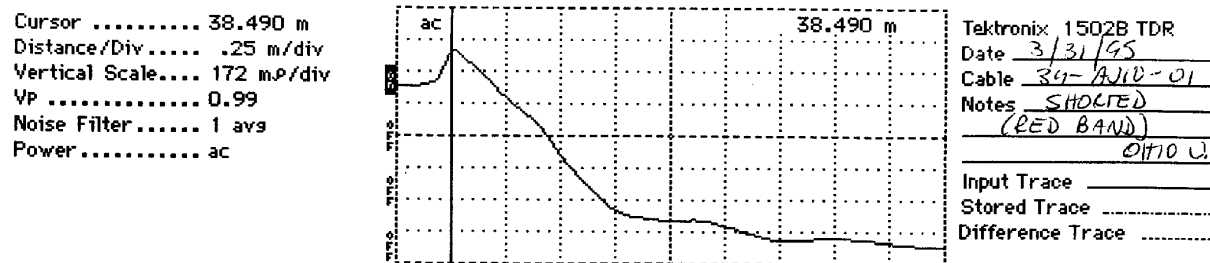
Figure 3.8 Shorted TDR Probe Calibration Sheet
