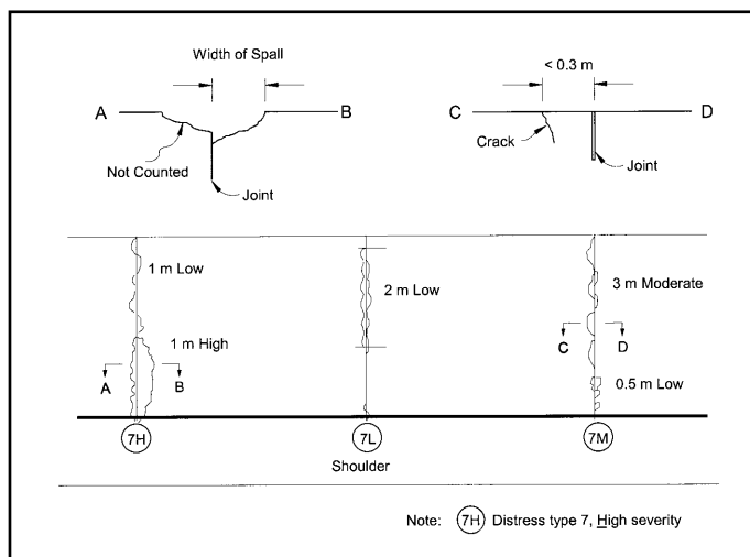
FIGURE 66 Distress Type JCP 7—Spalling of Transverse Joints
