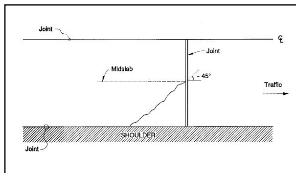
FIGURE 48 Distress Type JCP 1—Corner Breaks
