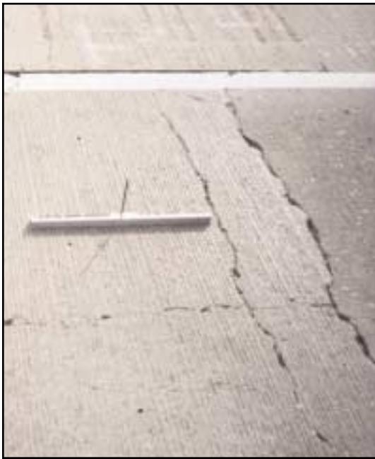
FIGURE 125 Distress Type CRCP 12—Low Severity Punchouts
