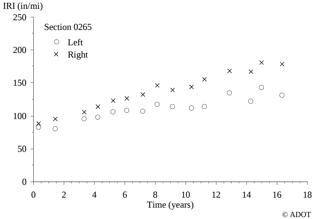
Figure 43. Graph. IRI Progression for Section 0265.
