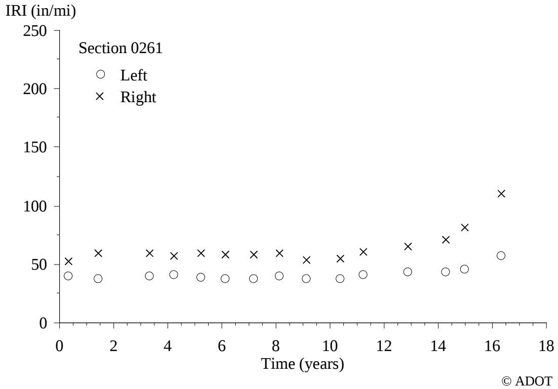
Figure 39. Graph. IRI Progression for Section 0261.
