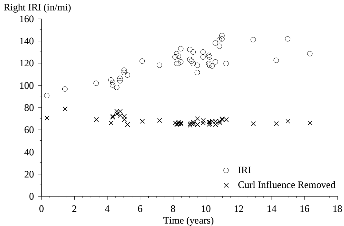
Figure 13. Graph. Right IRI Progression for Section 0215.
