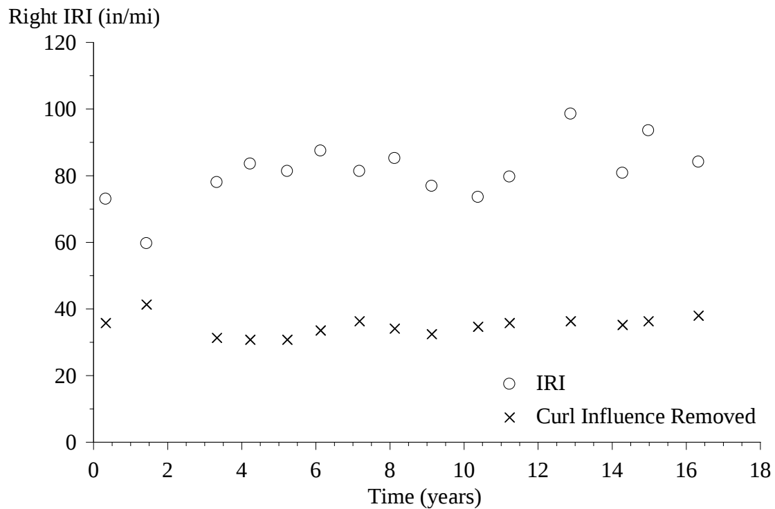
Figure 19. Graph. Right IRI Progression for Section 0221.
