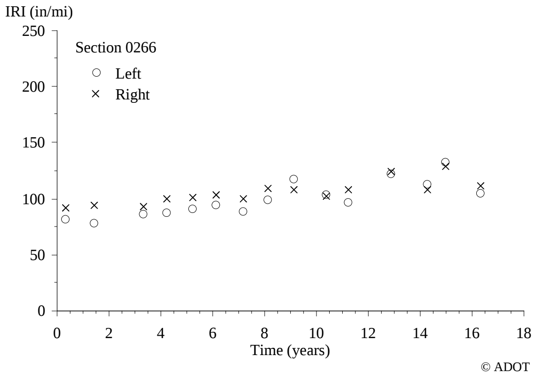
Figure 44. Graph. IRI Progression for Section 0266.
