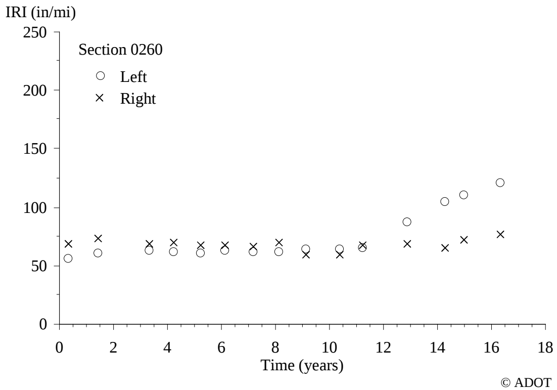
Figure 38. Graph. IRI Progression for Section 0260.
