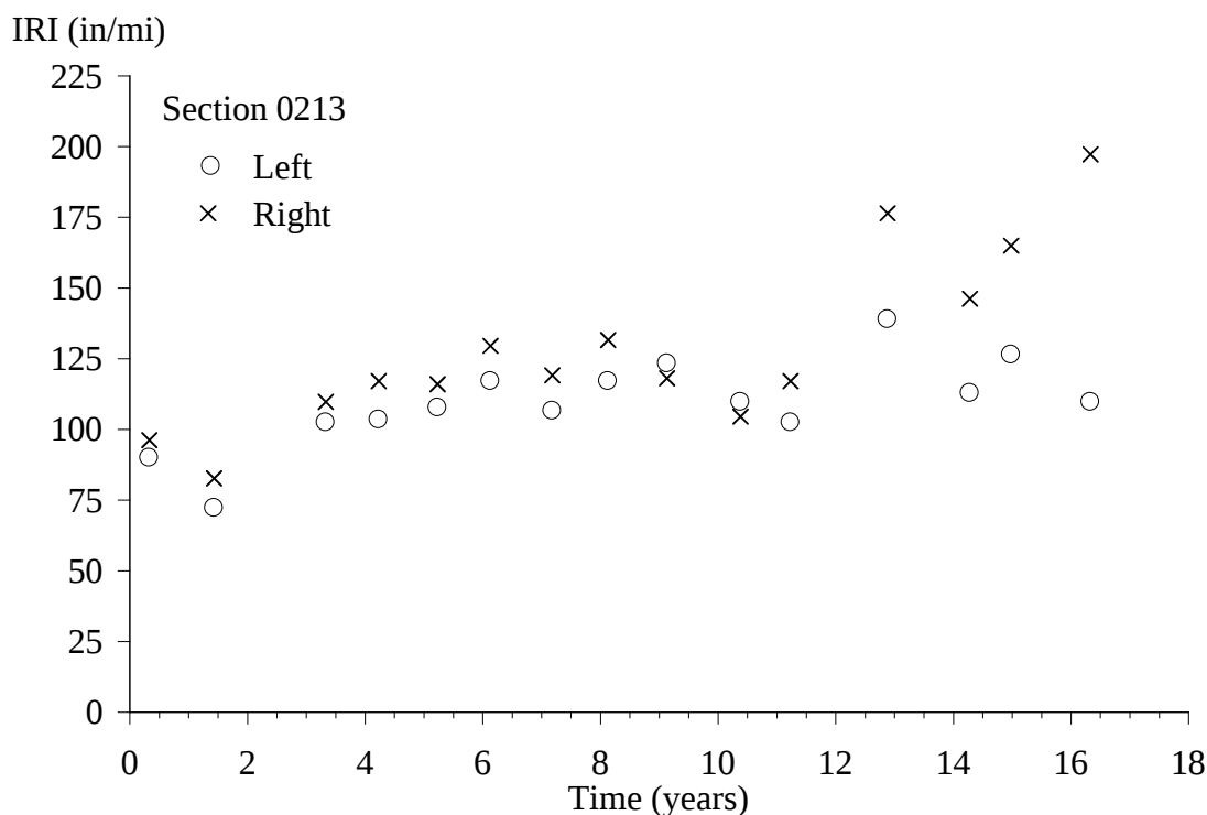
Figure 1. Graph. IRI Progression for Section 0213.
