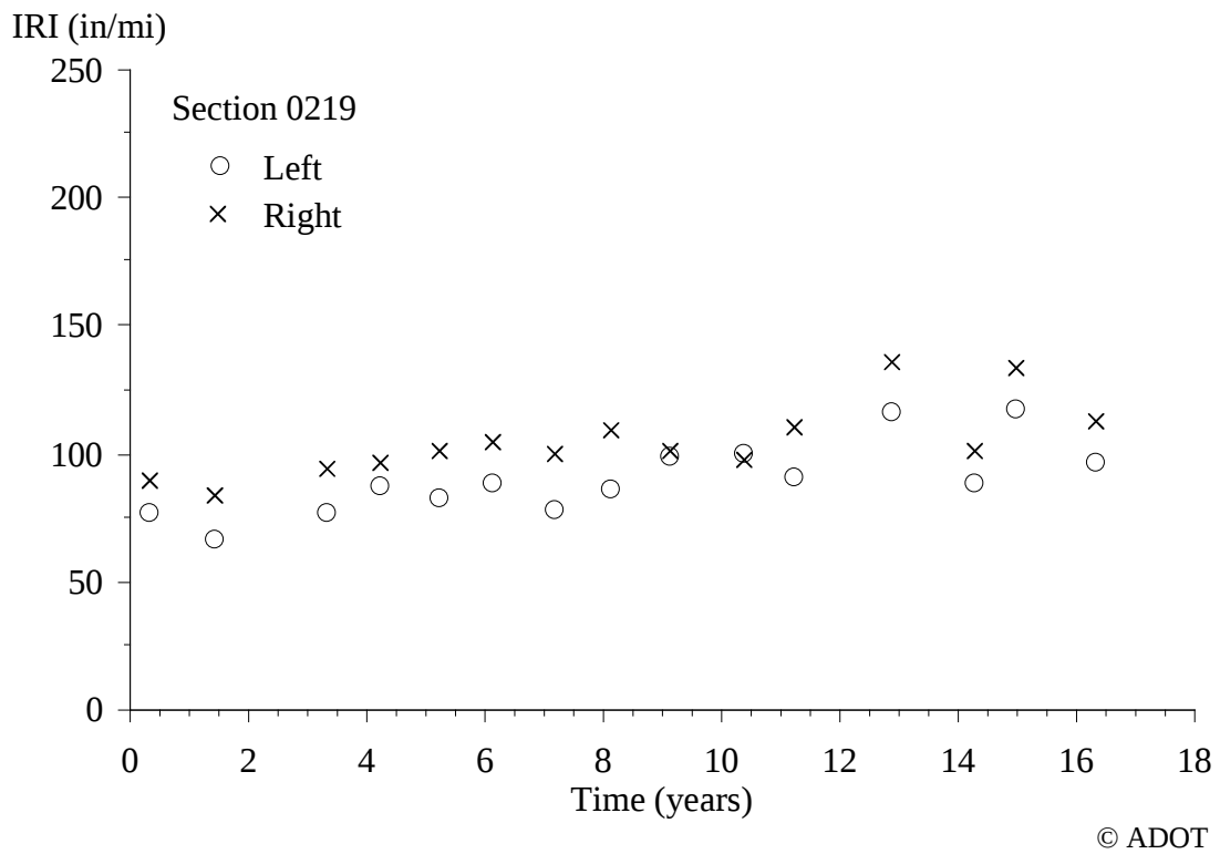
Figure 32. Graph. IRI Progression for Section 0219.
