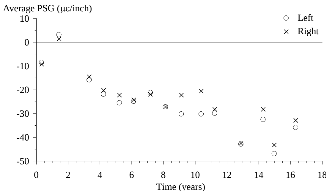
Figure 5. Graph. Average PSG versus Time for Section 0223.
