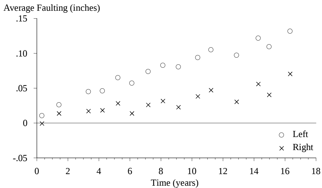
Figure 23. Graph. Faulting for Section 0265.
