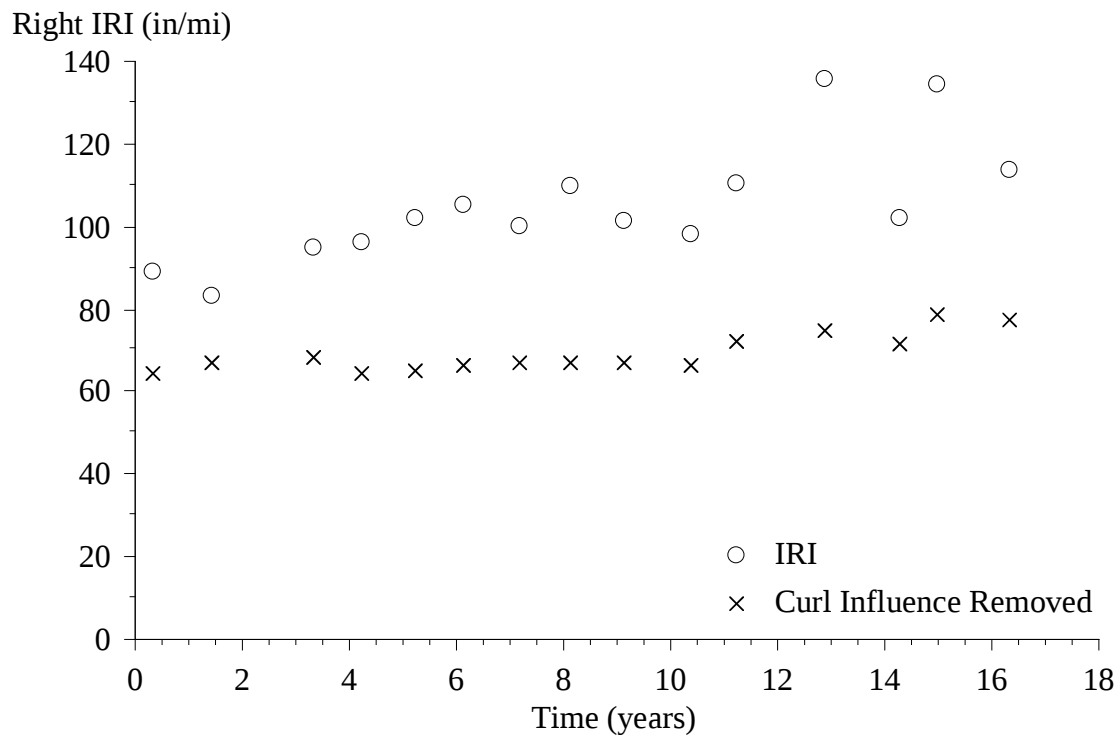
Figure 17. Graph. Right IRI Progression for Section 0219.
