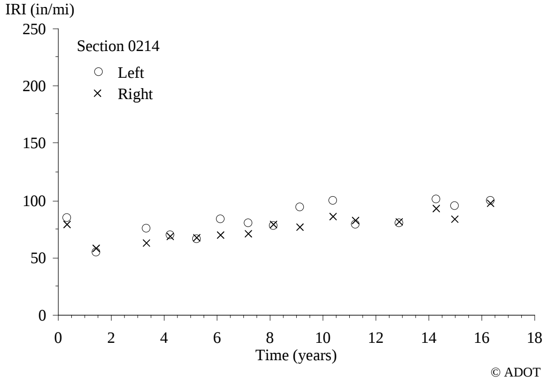
Figure 27. Graph. IRI Progression for Section 0214.
