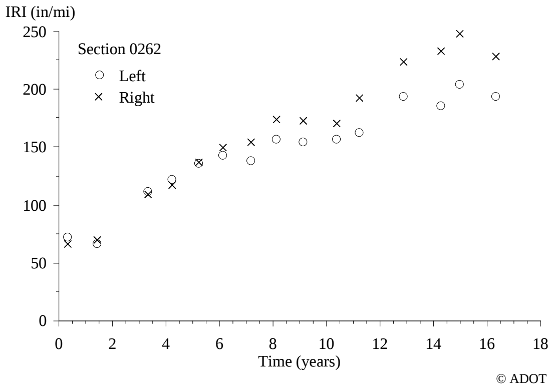
Figure 40. Graph. IRI Progression for Section 0262.
