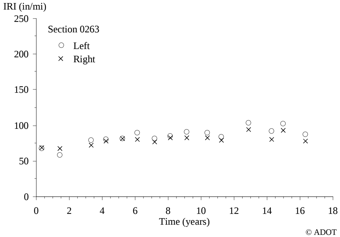
Figure 41. Graph. IRI Progression for Section 0263.
