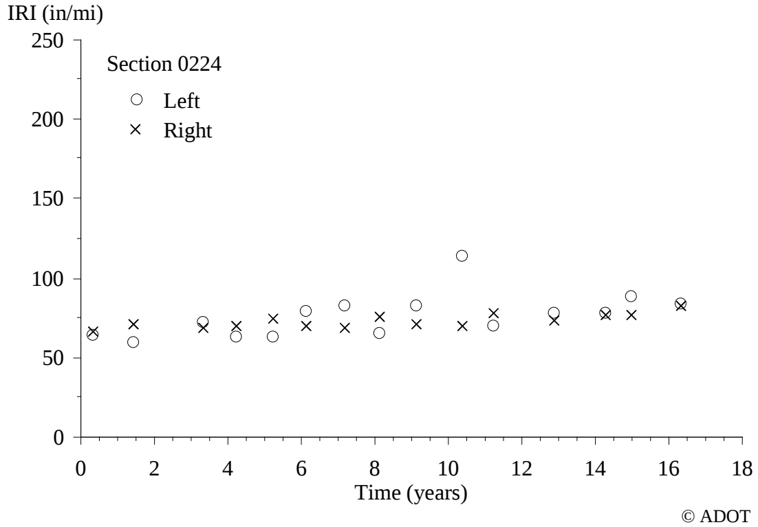
Figure 37. Graph. IRI Progression for Section 0224.
