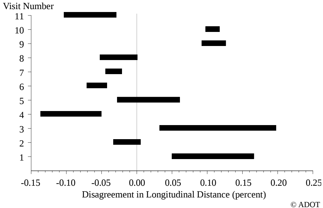
Figure 24. Graph. Consistency in Longitudinal Distance Measurement.
