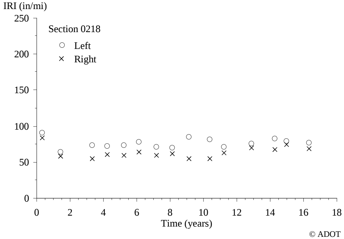
Figure 31. Graph. IRI Progression for Section 0218.
