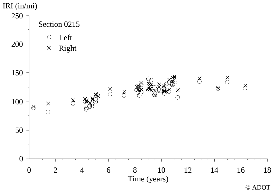
Figure 28. Graph. IRI Progression for Section 0215.
