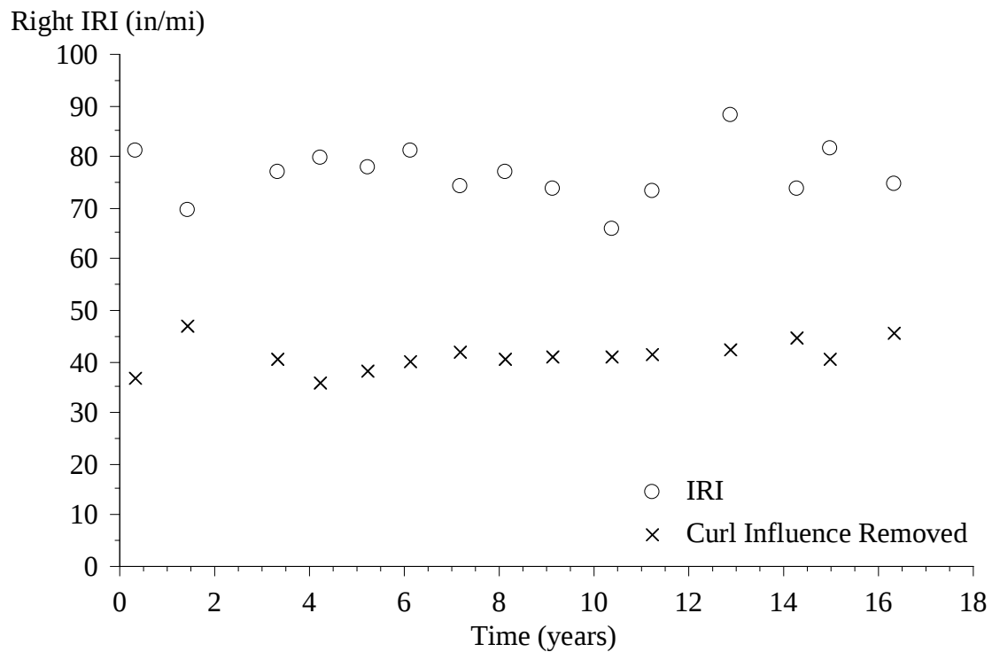
Figure 15. Graph. Right IRI Progression for Section 0217.
