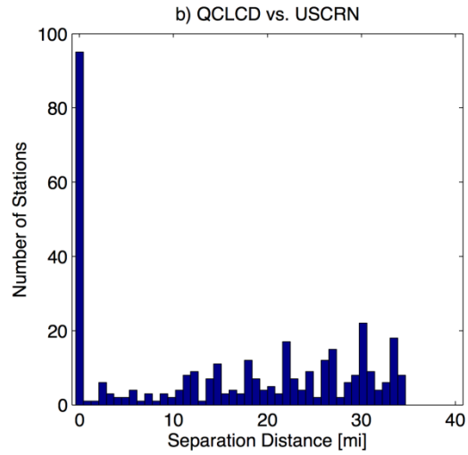
Figure 63. Histogram. Histogram of separation distances (in mi) relative to QCLCD for USCRN stations.
