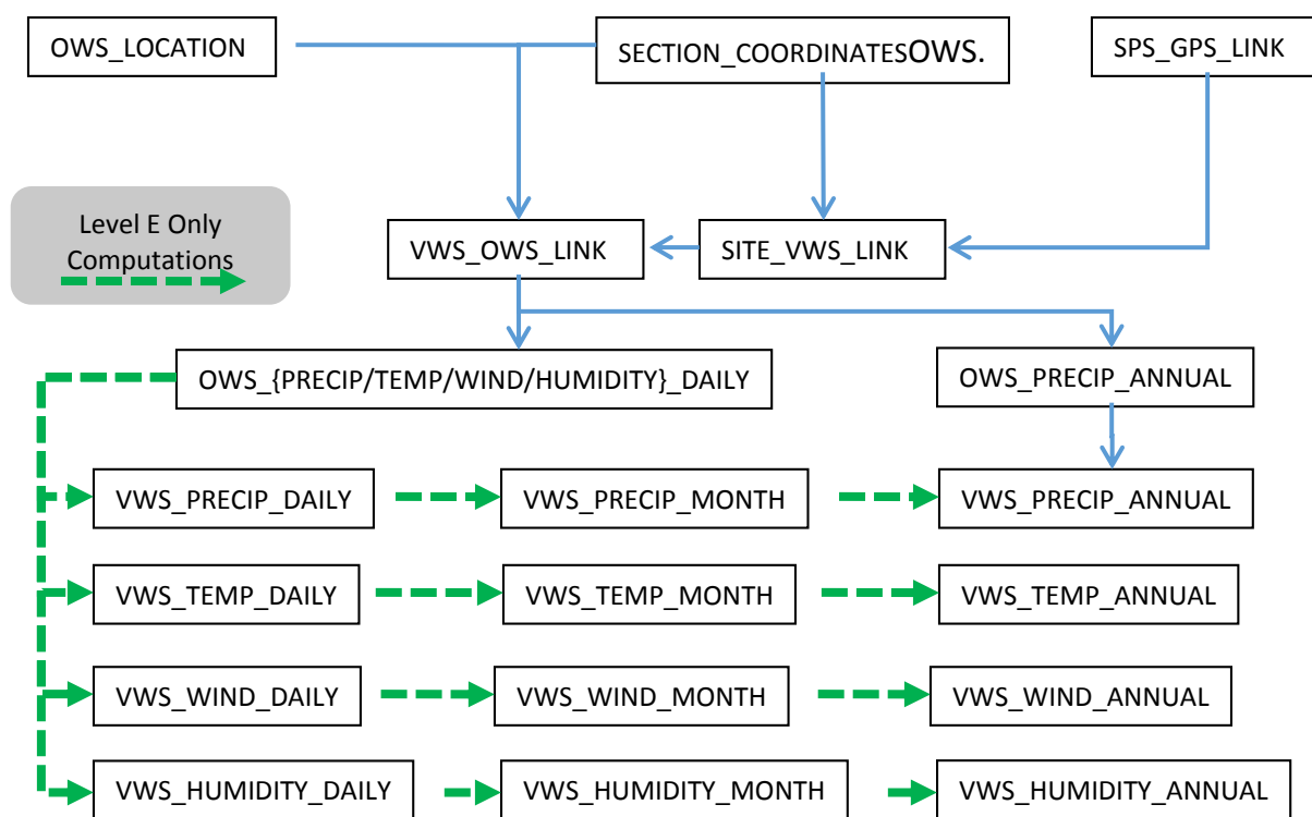
Figure 6. Schematic. Computational and relational structure of the CLM_VWS tables.
