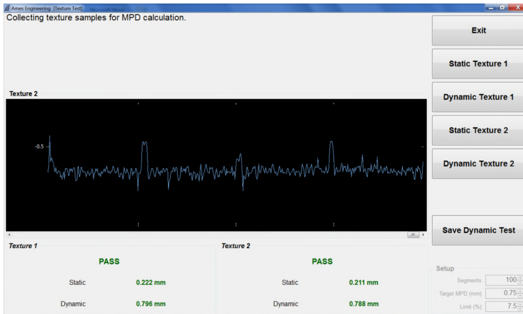
Figure 119. Results from a completed texture calibration check.
