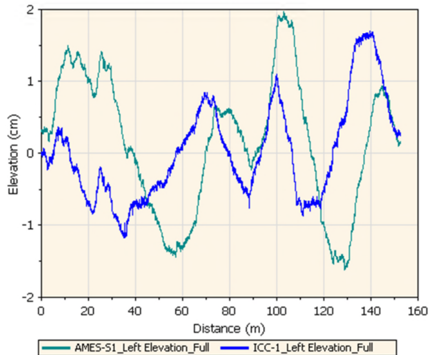
Figure 130. ICC and Ames profile data collected at Section 1.
