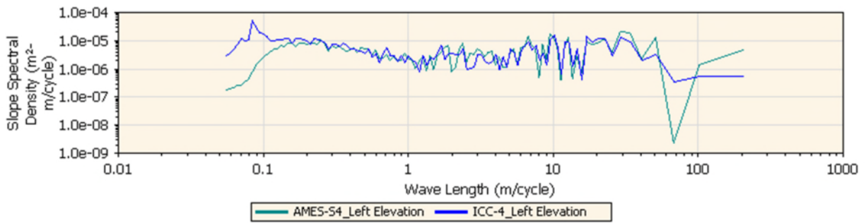
Figure 133. PSD plot of profile data collected by ICC and Ames devices at section 4.
