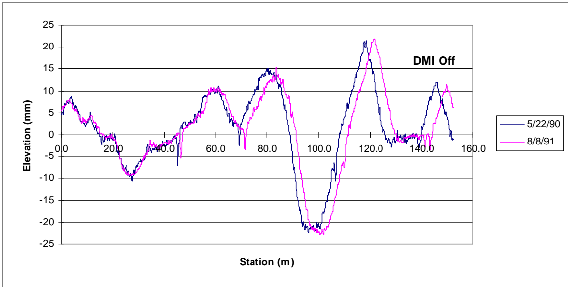
Figure 126. Data collected with a correctly calibrated and a miscalibrated DMI.
