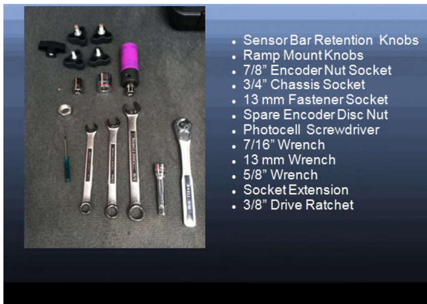
Figure 39. Contents of the toolbox.
