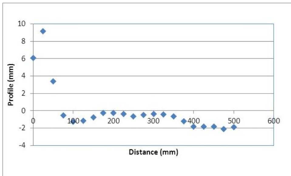
Figure 123. Example plot of data from photocell initiation test with two points on the target.
