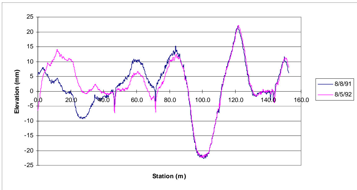
Figure 129. Differences in profile due to maintenance within section.
