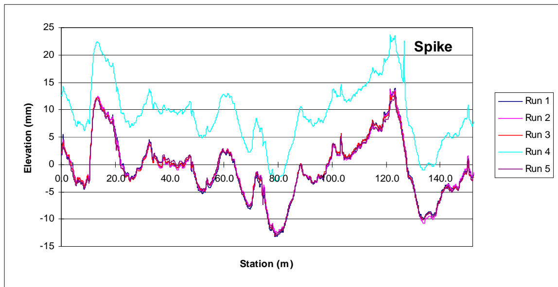
Figure 125. Spike in profile data (profile data for run 4 has been offset for clarity).
