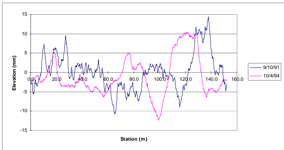
Figure 128. Differences in profile due to rehabilitation of section.
