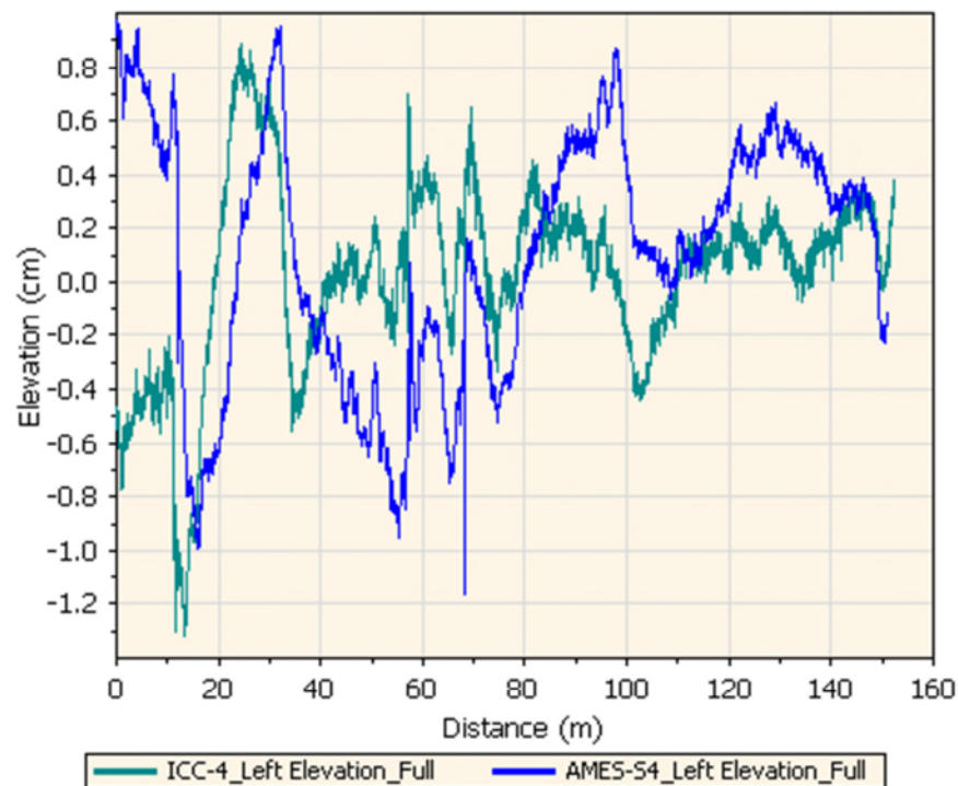
Figure 132. ICC and Ames profile data collected at Section 4.
