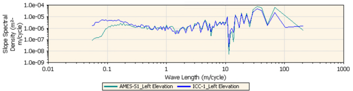
Figure 131. PSD plot of profile data collected by ICC and Ames devices at section 1.
