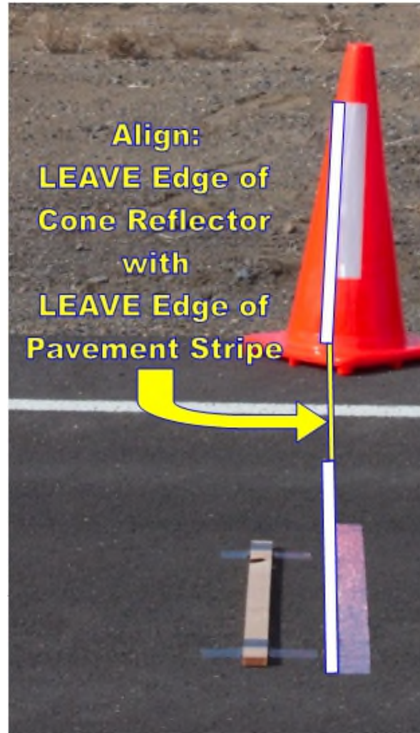
Figure 121. Placement of vertical photocell target in relation to section starting location.
