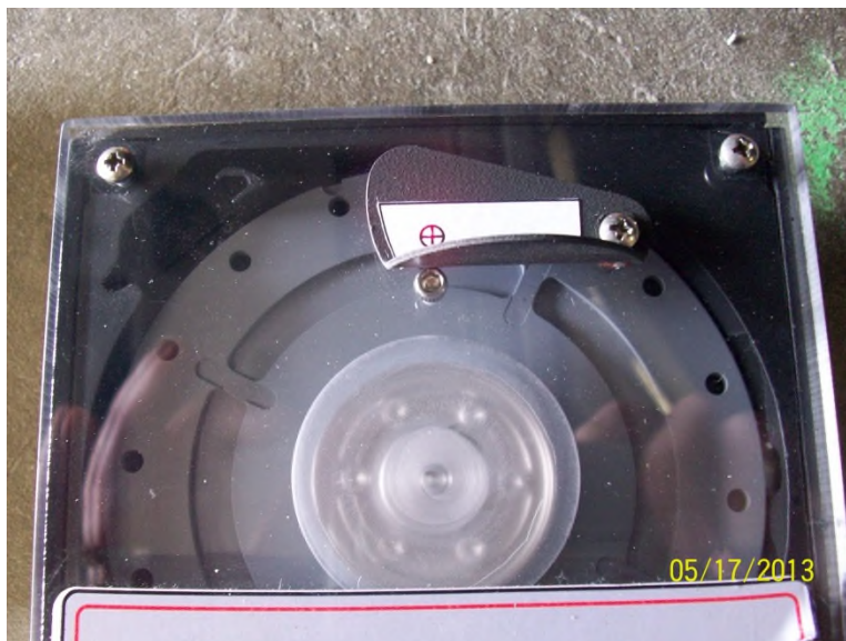
Figure 115. Target on texture reference test device.
