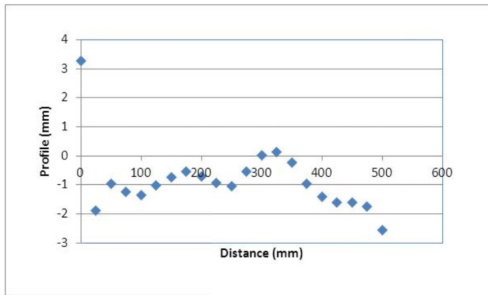
Figure 122. Example plot of data from photocell initiation test with one point on the target.
