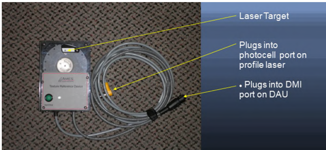
Figure 114. Texture reference test device.
