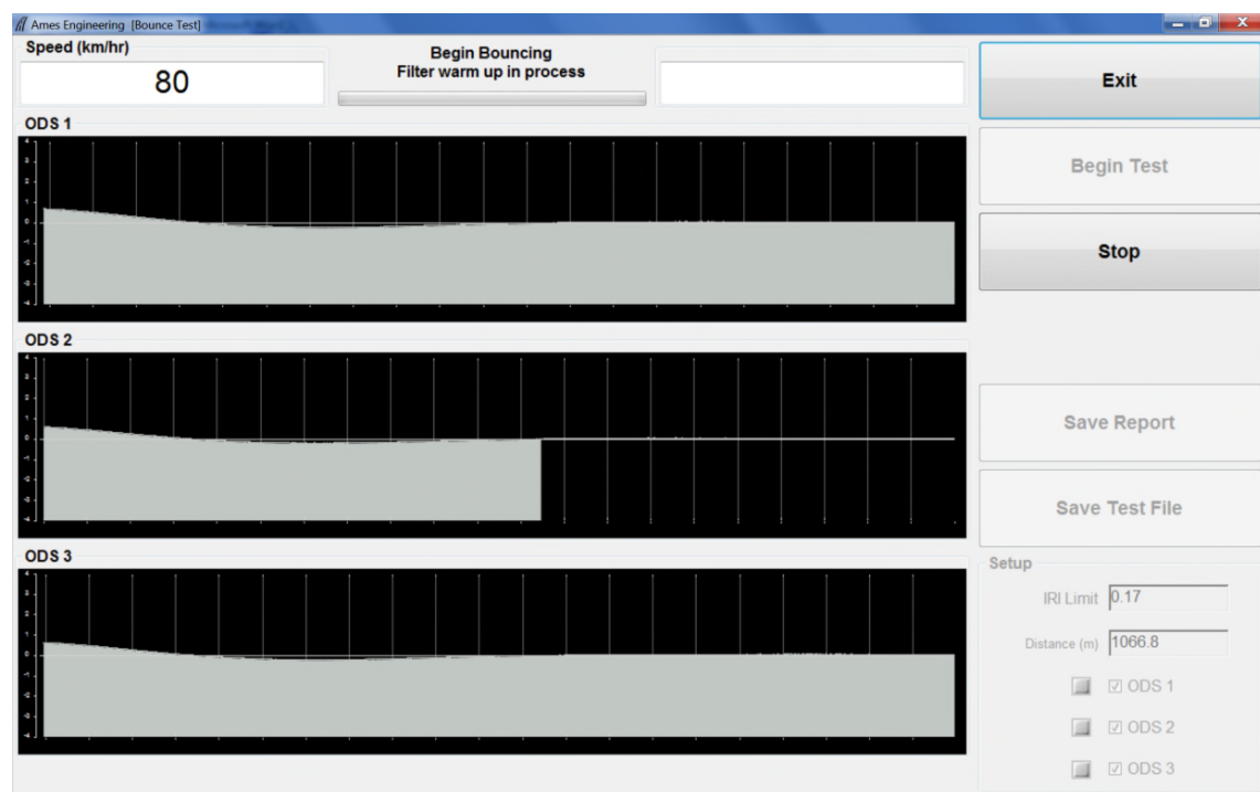
Figure 80. Filter warm-up in progress during bounce test.
