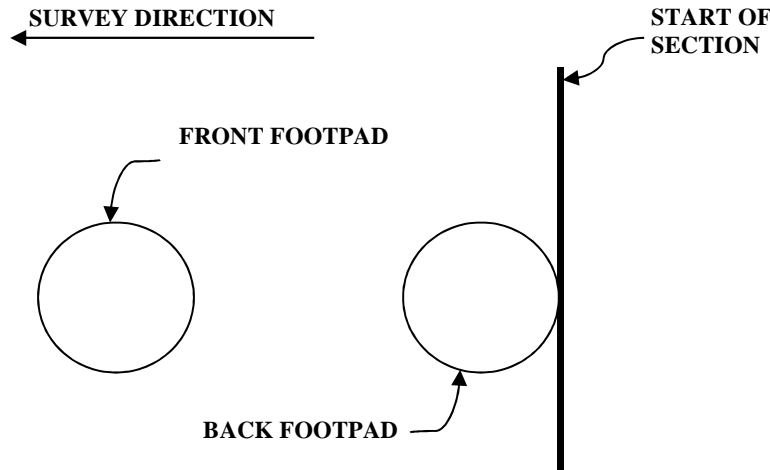
Figure 137. Location of back footpad of Dipstick® at start of the section.
