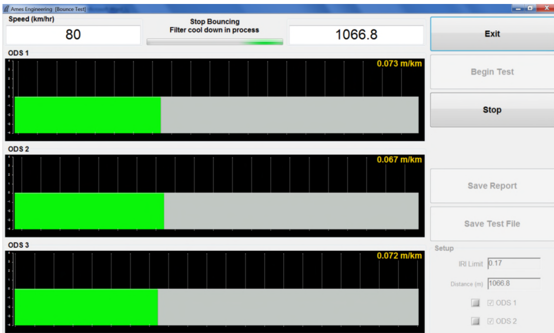
Figure 81. Filter cool-down process after bounce test is terminated.
