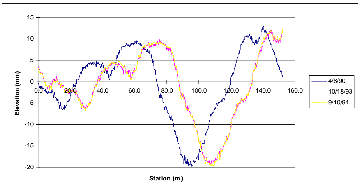
Figure 127. Example of early profile start.
