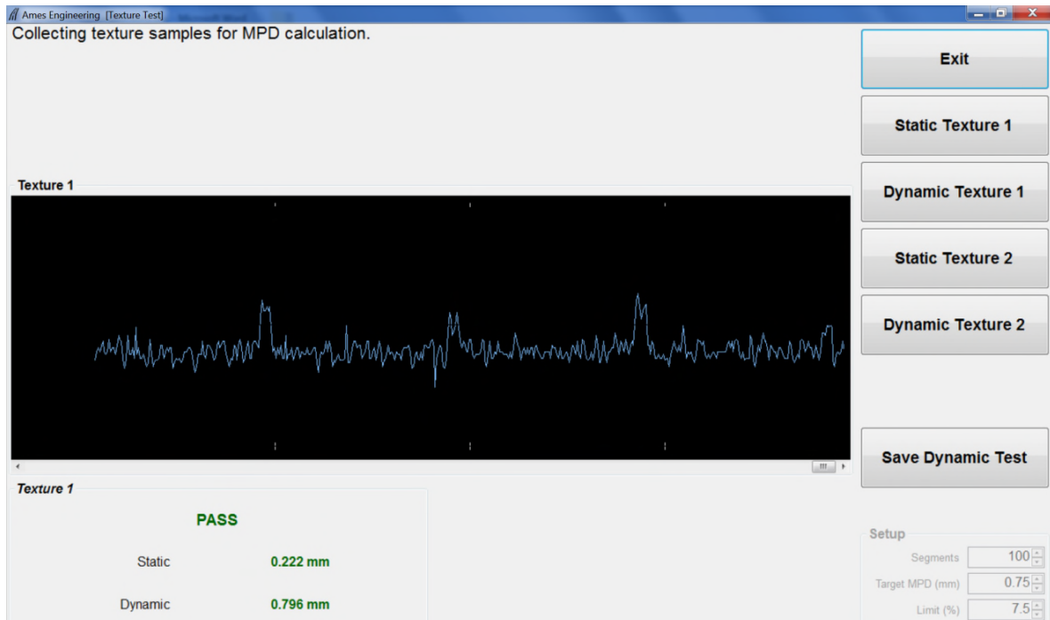
Figure 118. Texture reference test screen after dynamic test on left sensor.
