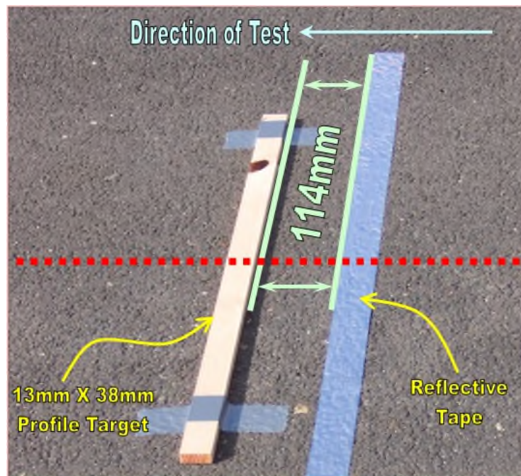
Figure 120. Section starting stripe and bump target placed on the pavement.
