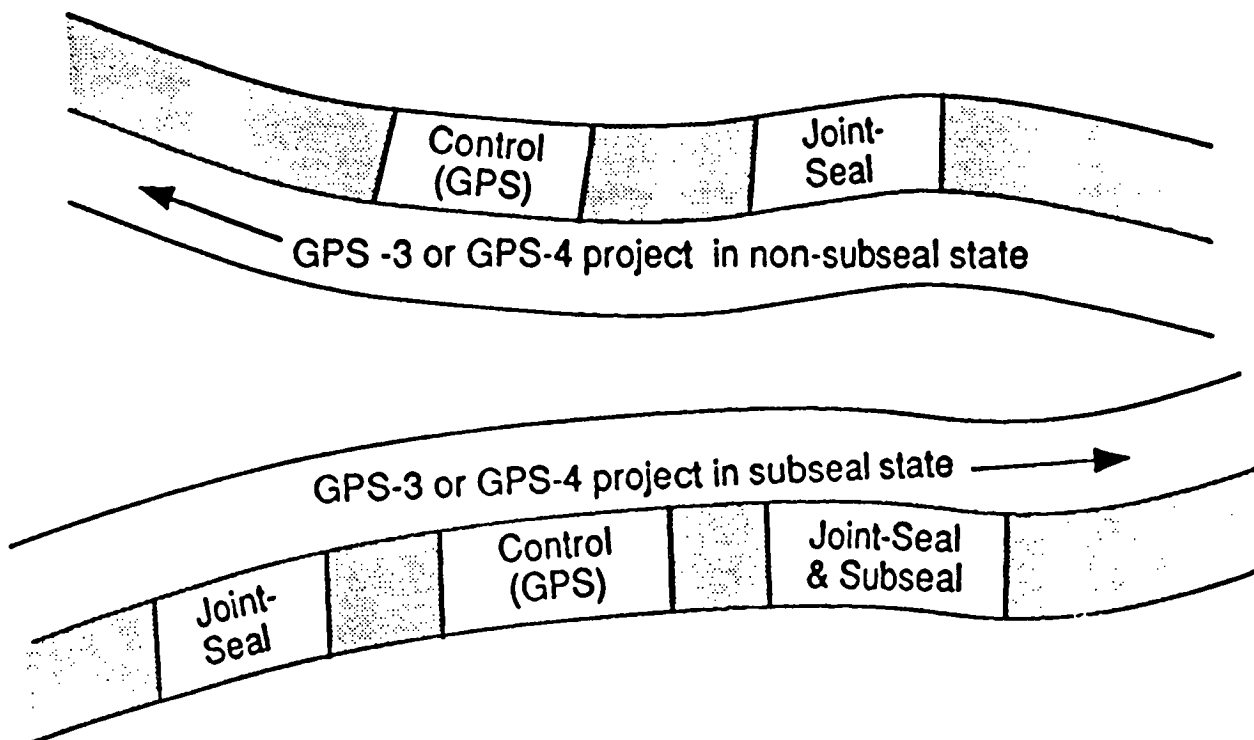
Figure 3.2. Test Section Layout for SPS-3 and SPS-4: Studies of Preventive Maintenance Effectiveness
