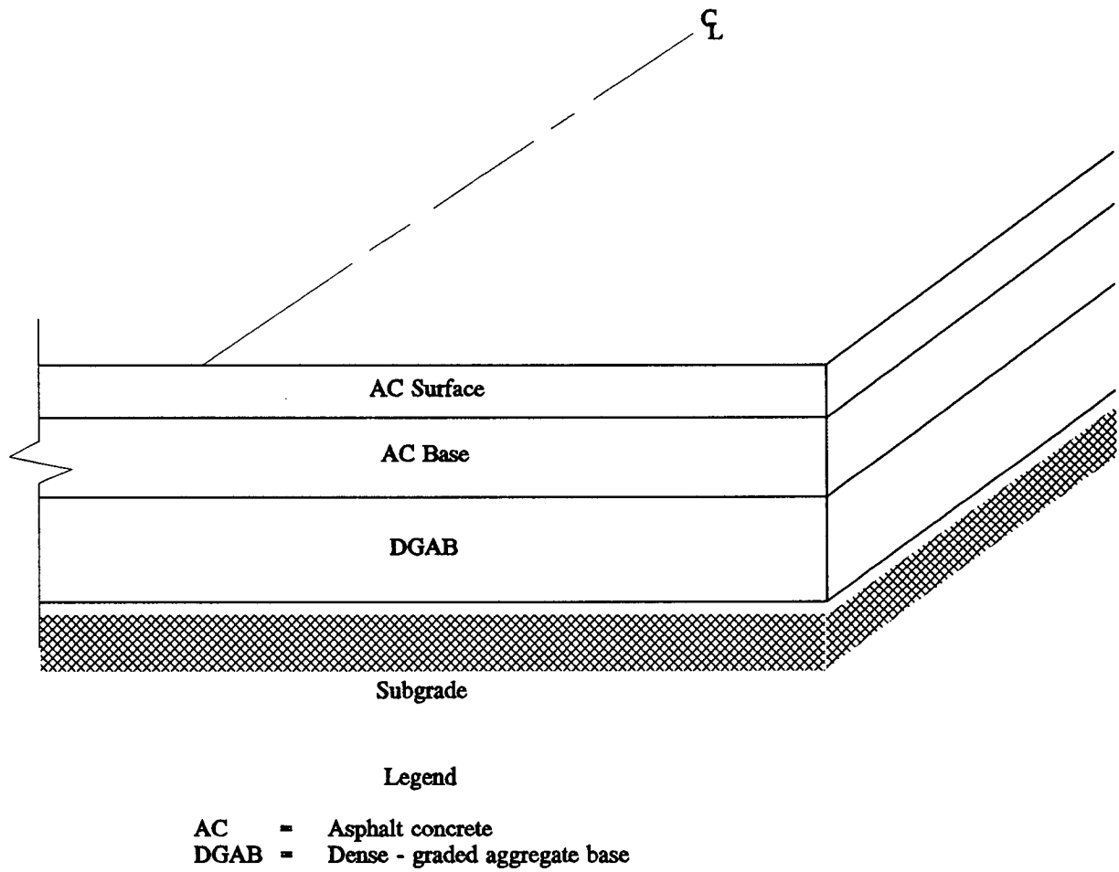
Figure 13. Example of pavement layers for a candidate project.
