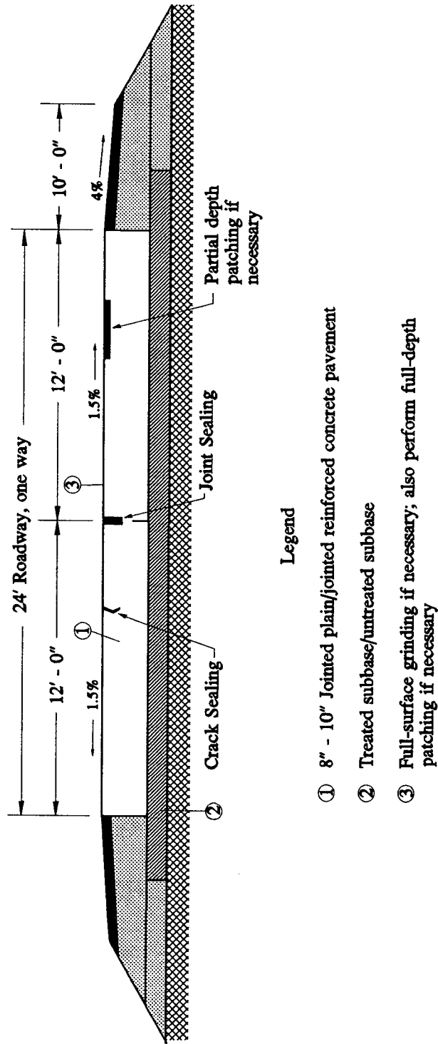
Figure 21. A test section rehabilitated with minimal restoration and no overlay.
