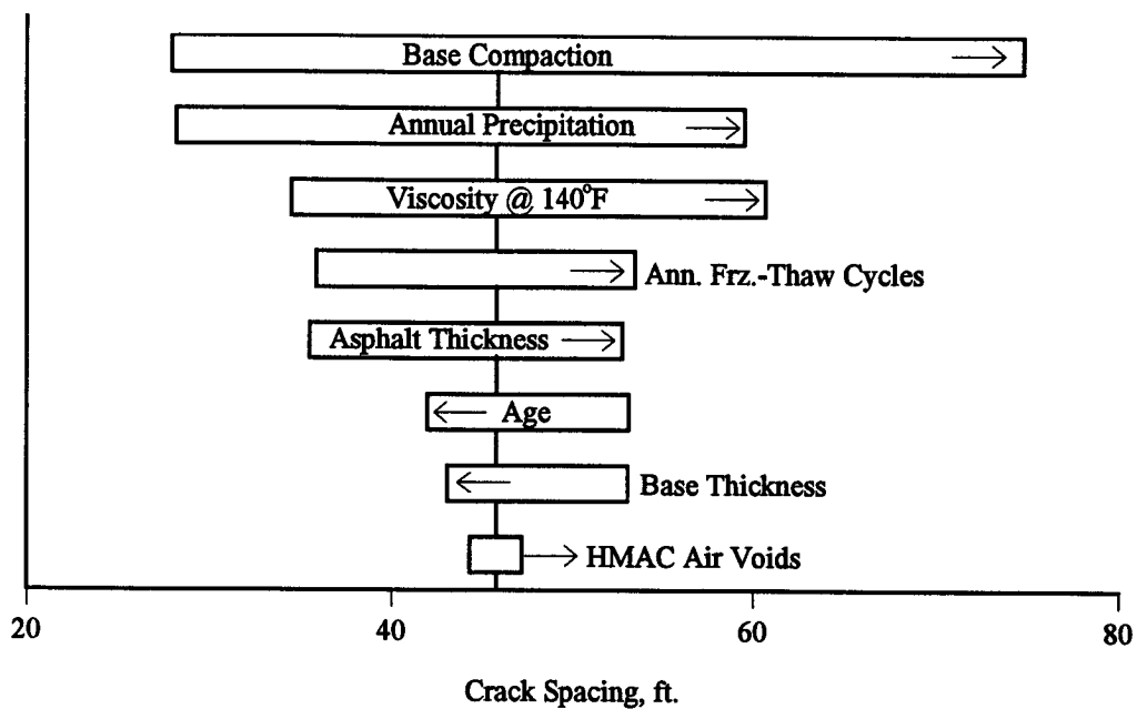
Figure 7.38. Results From Sensitivity Analyses for Transverse Crack Spacing in HMAC Pavements on Granular Base and Full-Depth HMAC Pavements, North American Data Set
