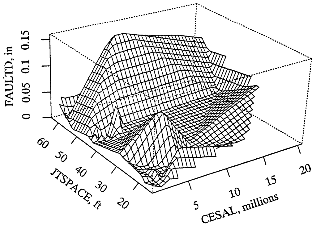
Figure 8.5. Three-Dimensional Plot (FAULTD, JTSPACE, CESAL) of Doweled Joint Faulting
