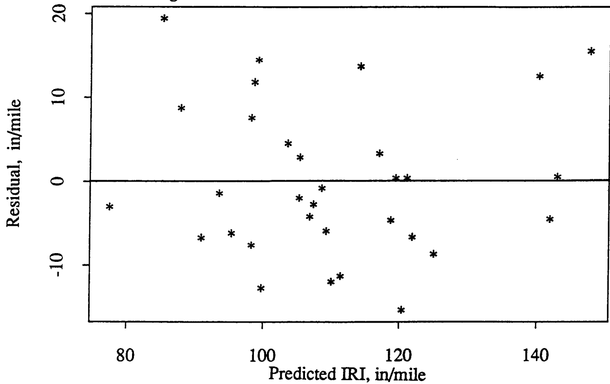
Figure 8.47. Plot of Residuals vs. Predicted IRI for JRCP
