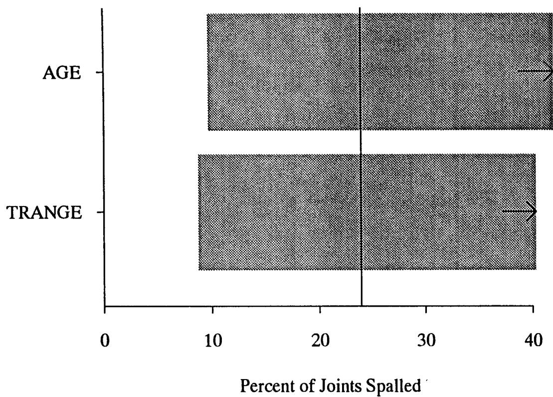
Figure 8.33. Sensitivity Analysis for Joint Spalling of JRCP (SPALLJR) Model
