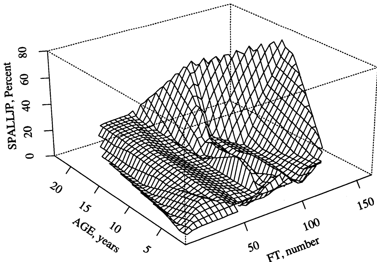
Figure 8.25. Three-Dimensional Plot (SPALLJP, AGE, FT) for JPCP Joint Spalling
