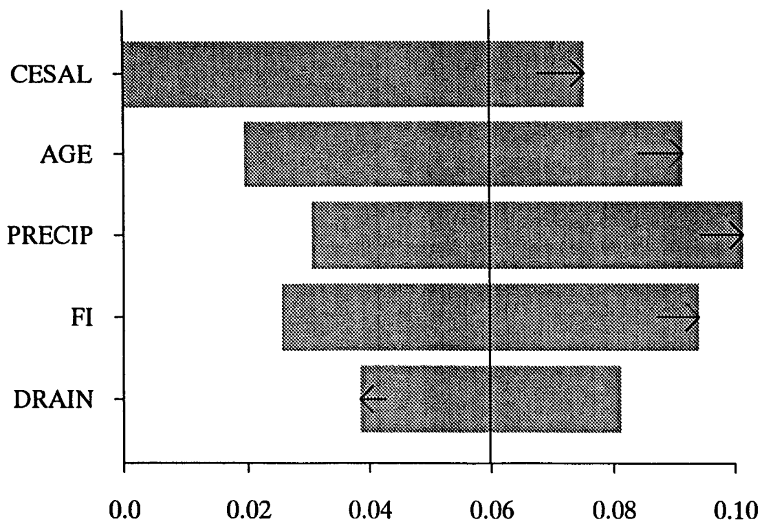
Figure 8.14. Sensitivity Analysis for Non-Doweled Joint Faulting Model
