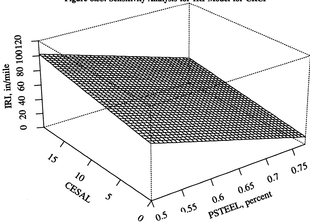
Figure 8.54. Three-Dimensional Plot of IRI Model for CRCP
