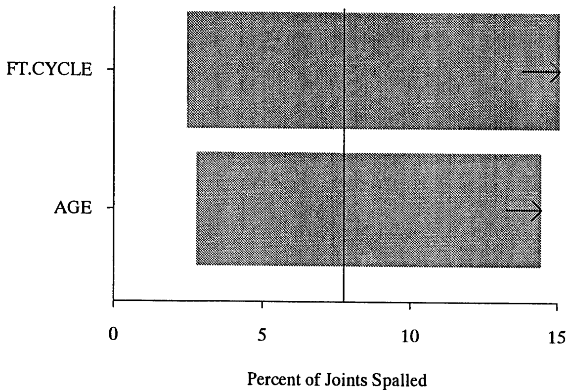
Figure 8.28. Sensitivity Analysis for Joint Spalling of JPCP (SPALLJP) Model
