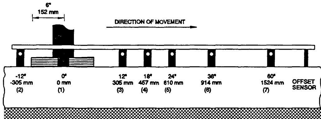
FIGURE 2B. SENSOR CONFIGURATION FOR LOAD TRANSFER TESTING
