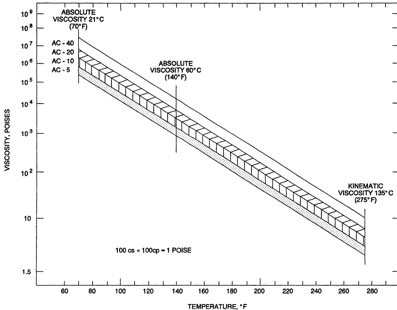
FIGURE 1. Typical Viscosity - Temperature Relationships.
