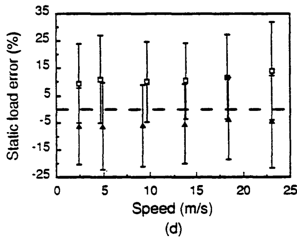
Fig. 3.3 Static load error vs speed, Vehicle S2 (a) Axle 1 (b) Axle 2 (c) Axle 3 (d) Axle 4 (e) Axle 5 Error bars indicate \pm 1 standard deviation
