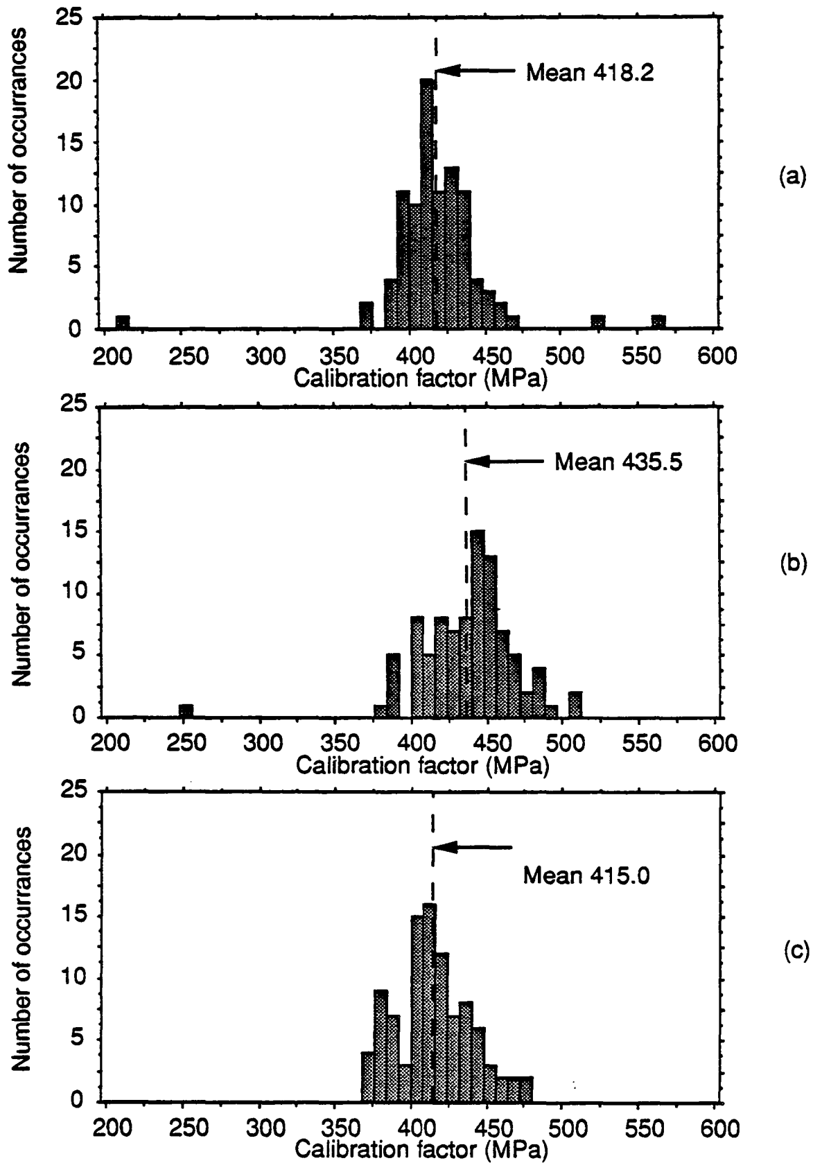
Fig. 2.3 Histograms of sensor calibration factors (a) Bare sensor calibrator (b) 'In-situ' calibrator (c) Field calibration with steer axles of 6 vehicles
