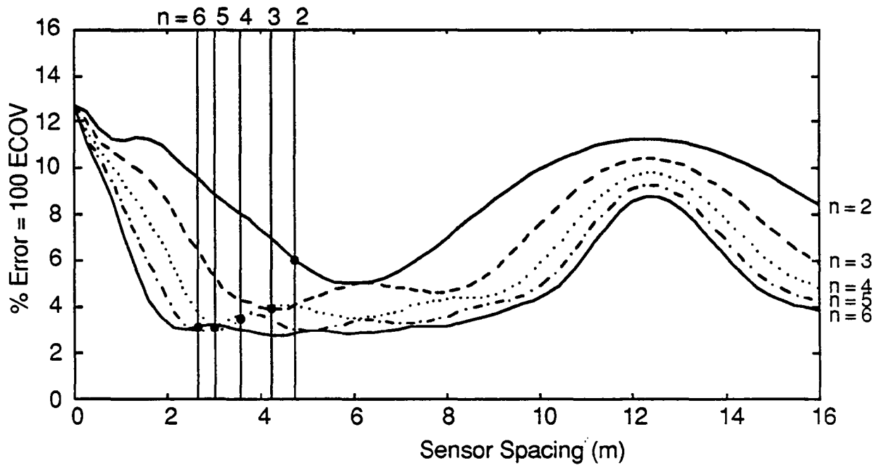
Fig. 5.8 Theoretical WIM array Error Coefficient of Variation \rho vs sensor spacing \Delta , 1/4-car model, speed = 85 km/h. Vertical lines denote design spacings according to eq 4.22.
