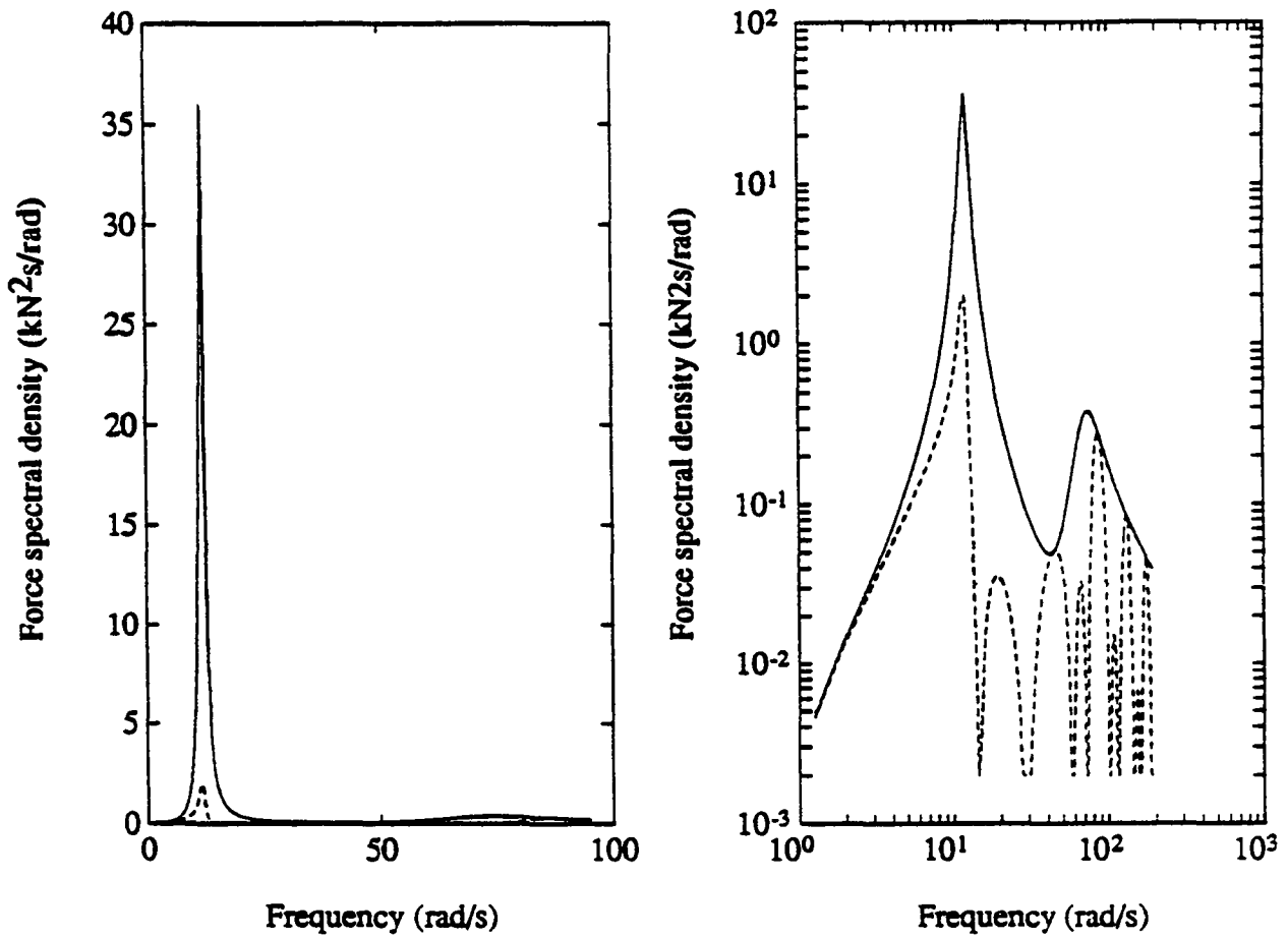
Fig. 4.6 Tyre force spectral density S_{pp}(\omega) and the WIM array error spectral density S_{ee}(\omega) for vehicle model 1 travelling at 100 km/h over a WIM array with n=3 and \Delta = 4 m. — = S_{pp}(\omega) , - - - = S_{ee}(\omega) .
