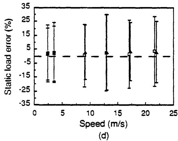
Fig. 3.4 Static load error vs speed, Vehicle S3 (a) Axle 1 (b) Axle 2 (c) Axle 3 (d) Axle 4 (e) Axle 5 Error bars indicate \pm 1 standard deviation
