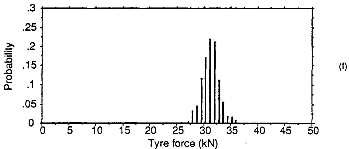
Fig. 5.2 Histograms of WIM average force, Vehicle S4, Axle 5, Speed = 23.7 m/s (85 km/h). (d) single sensor (e) 3 sensors, \Delta = 4.0 m (f) 6 sensors, \Delta = 2.4 m.
