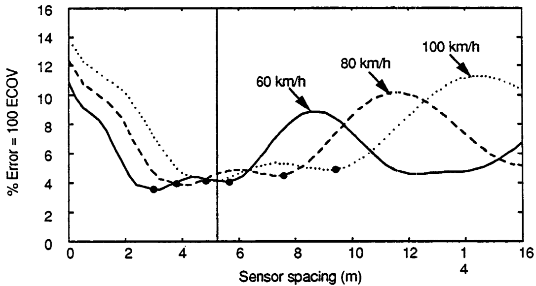
Fig. 5.9 Theoretical graph of \rho vs \Delta , for n = 3 and speeds of 60, 80 and 100 km/h. The design spacing was calculated using an average speed of 80 km/h and an average frequency of 1.9 Hz. The 'solid' circles on each curve correspond to \delta = 1/3 and \delta = 2/3 .
