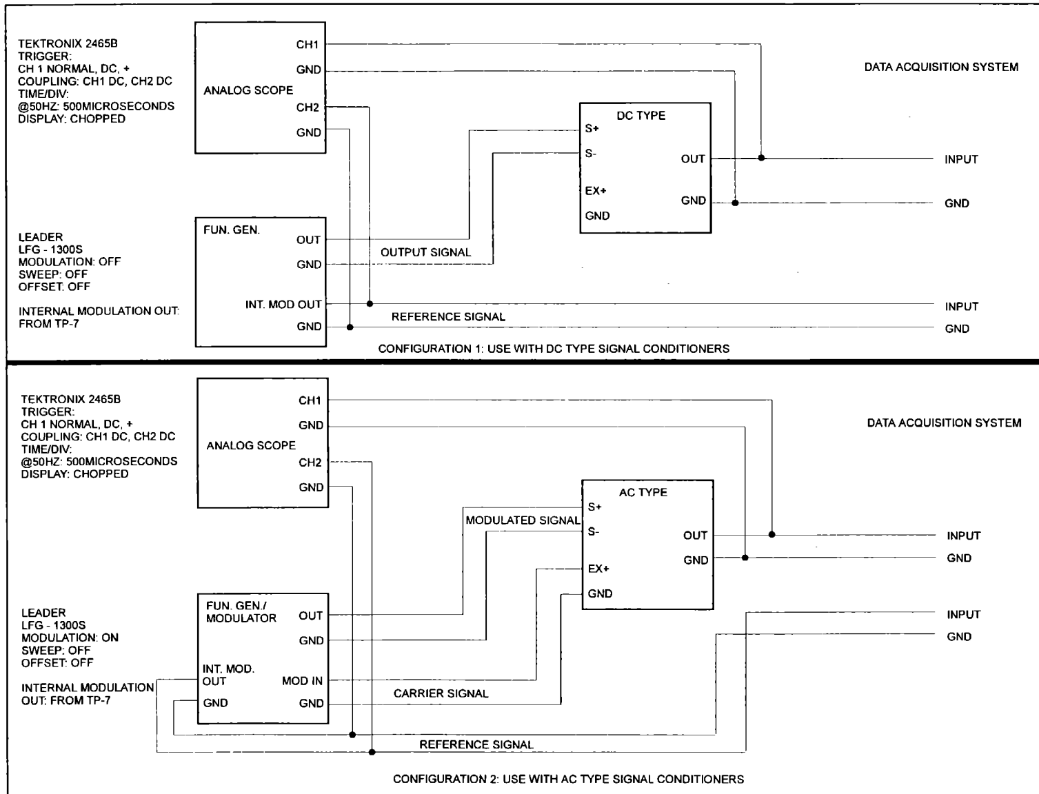
Figure 3. Frequency response test setup (simplified wiring).
