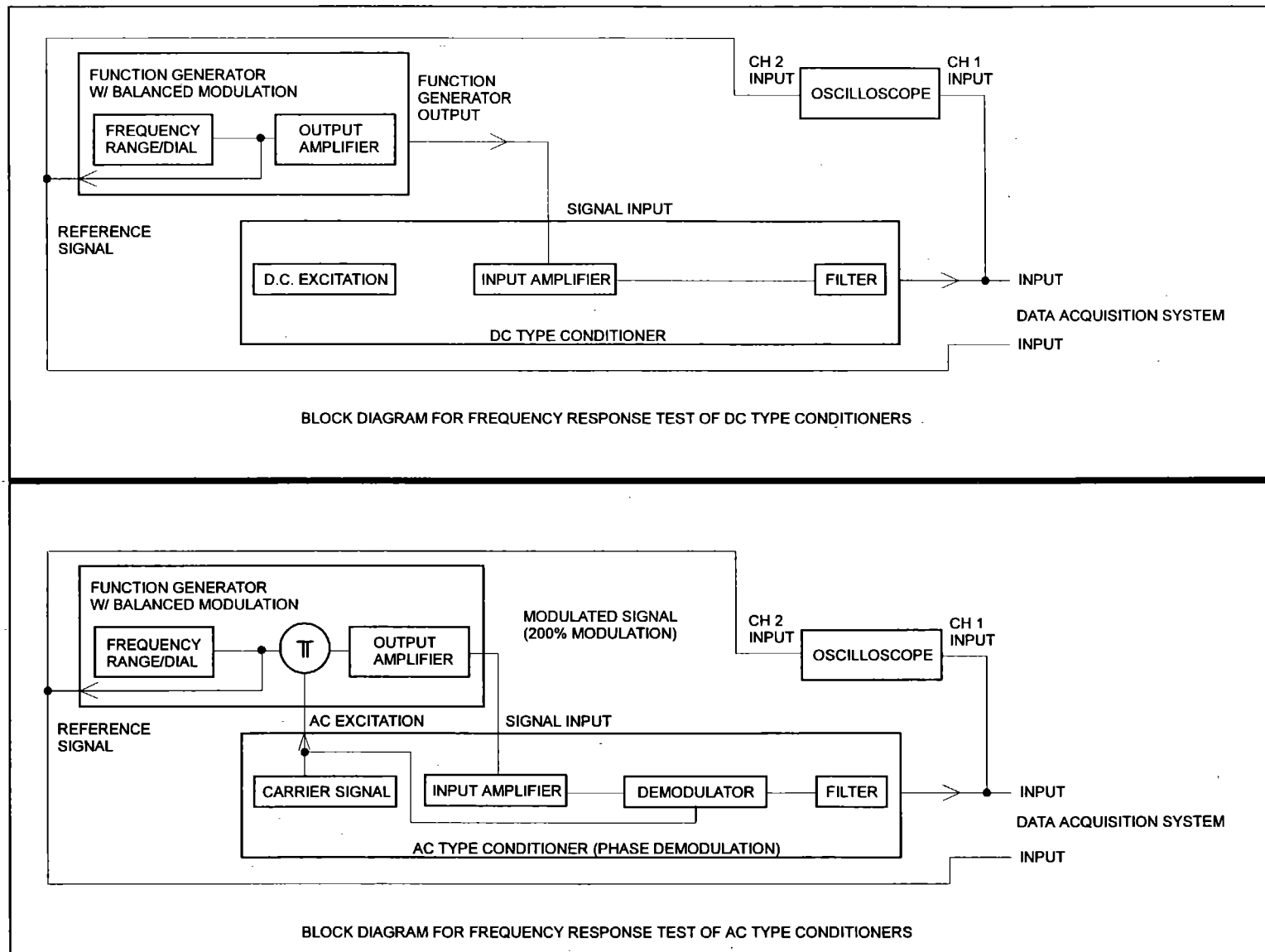
Figure 2. Frequency response test setup block diagram.
