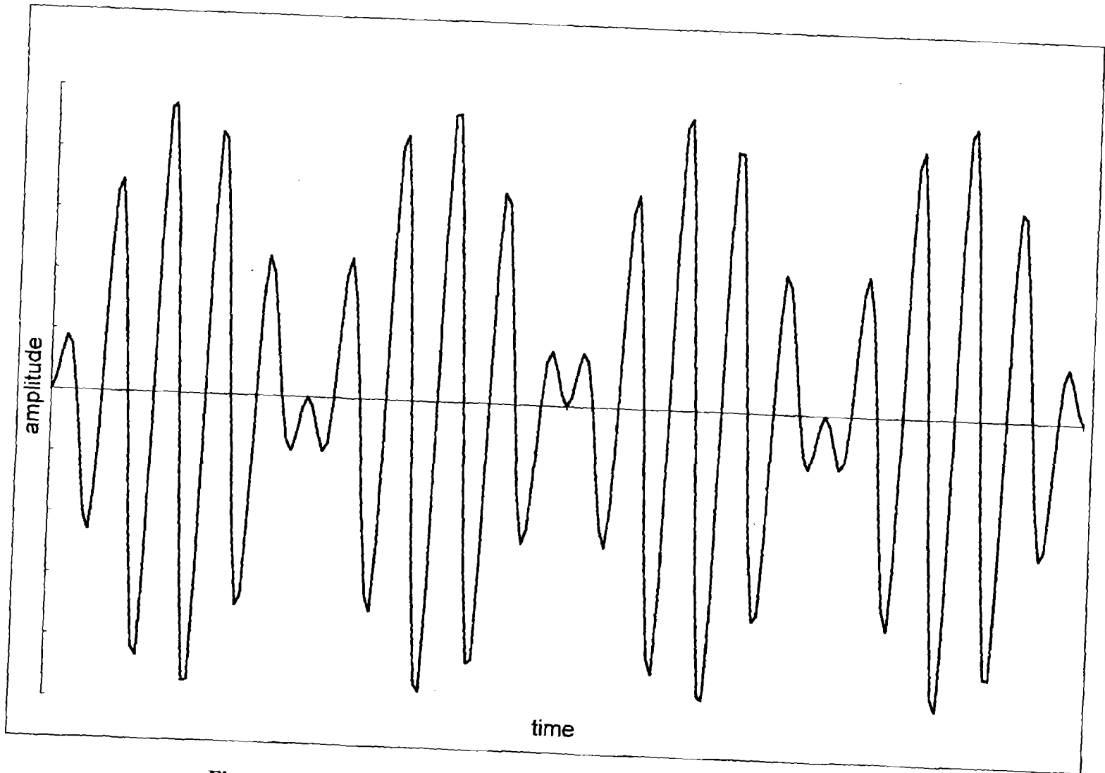
Figure 4. Example of double sideband suppressed carrier modulation.
