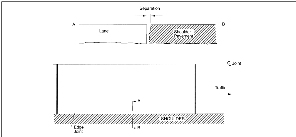
FIGURE 81 Distress Type JCP 14—Lane-to-Shoulder Separation.
