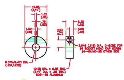
6 CLAMPING COLLAR
