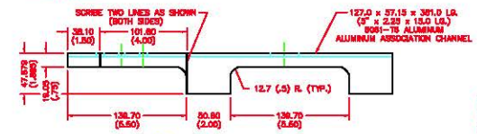
1 BASE PLATE
