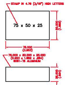
PRECISION CALIBRATING BLOCK
