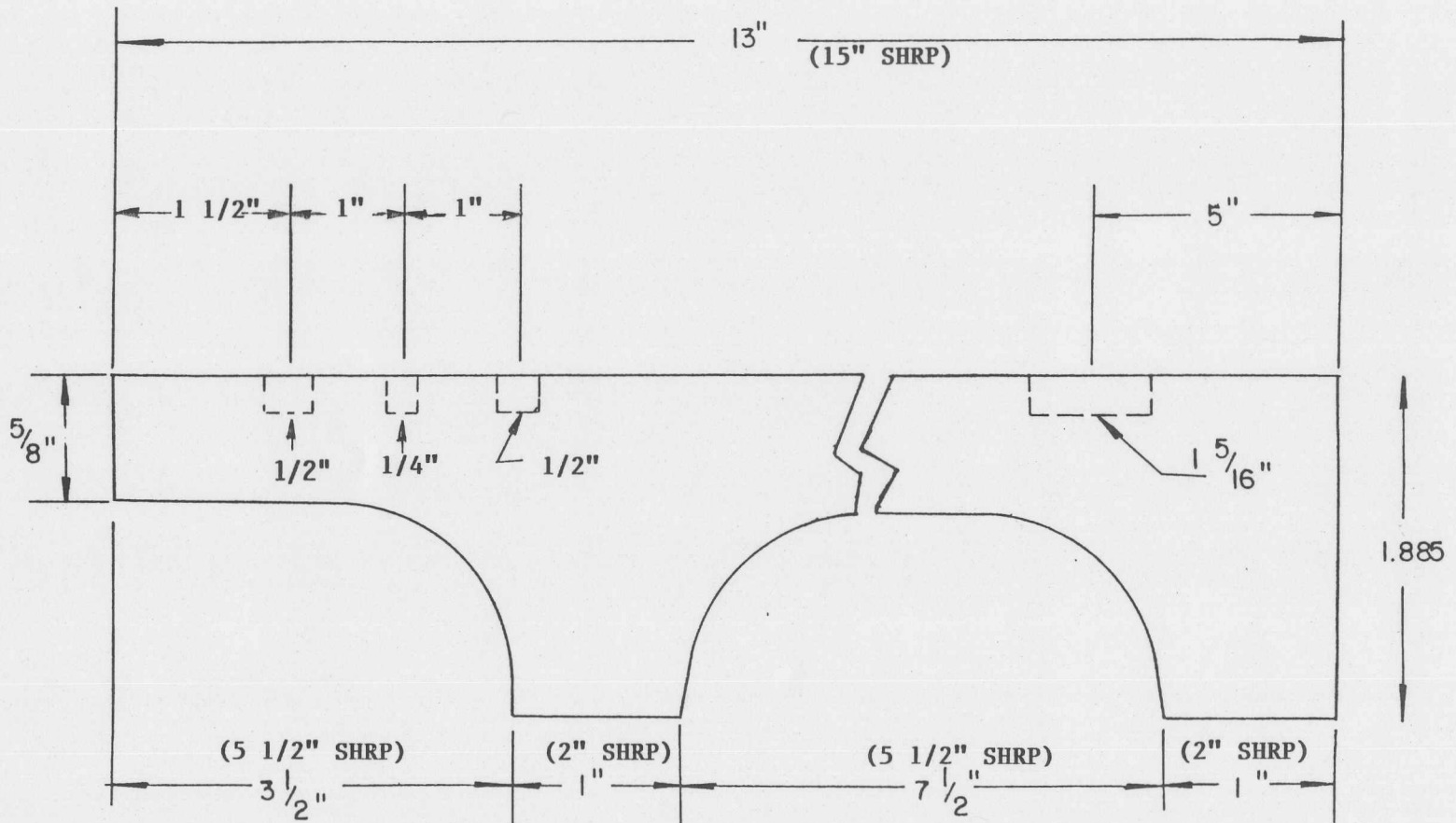
Figure 20. Drawing B-FM, Side View of Base Plate
