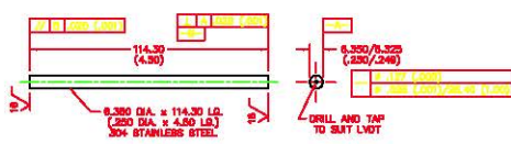
5 MEASURING ROD
