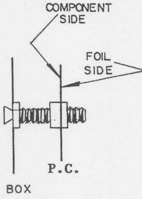
P.C. MOUNT-USE 4 - 1 1/4" SCREWS
