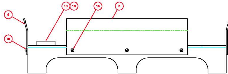
CALIBRATOR ASSEMBLY
