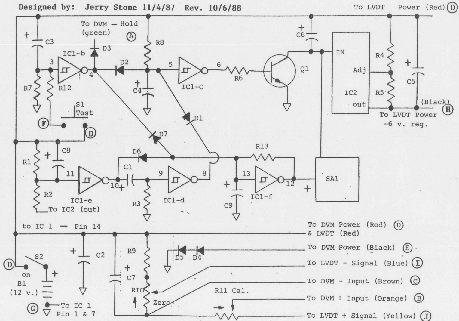
Figure 11. Schematic Diagram For Control P.C. Board
