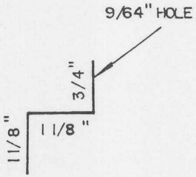
"Z" CLAMPS FOR METER & BATTERY- MAKE OUT OF SHEET METAL 3/4" WIDE
