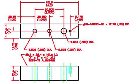
3 MEASURING ROD HOLDER
