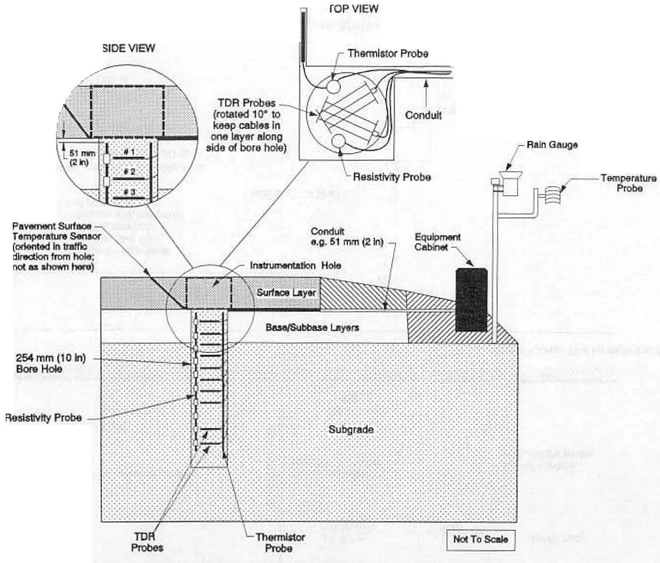
Figure II-13 - Illustration of Instrumentation Installation
