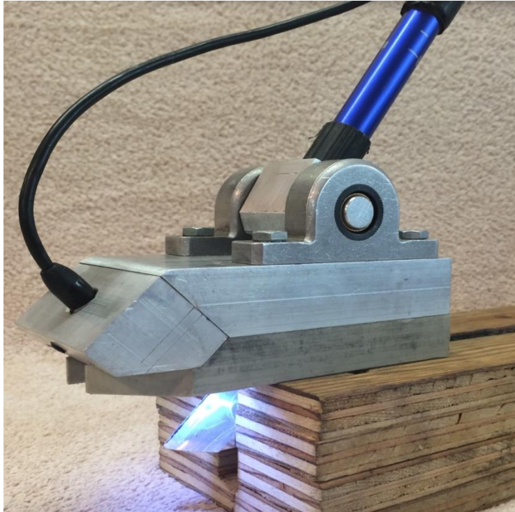
Figure 25. Photo. Joint inspection assembly - (JIS-QC), production prototype.
