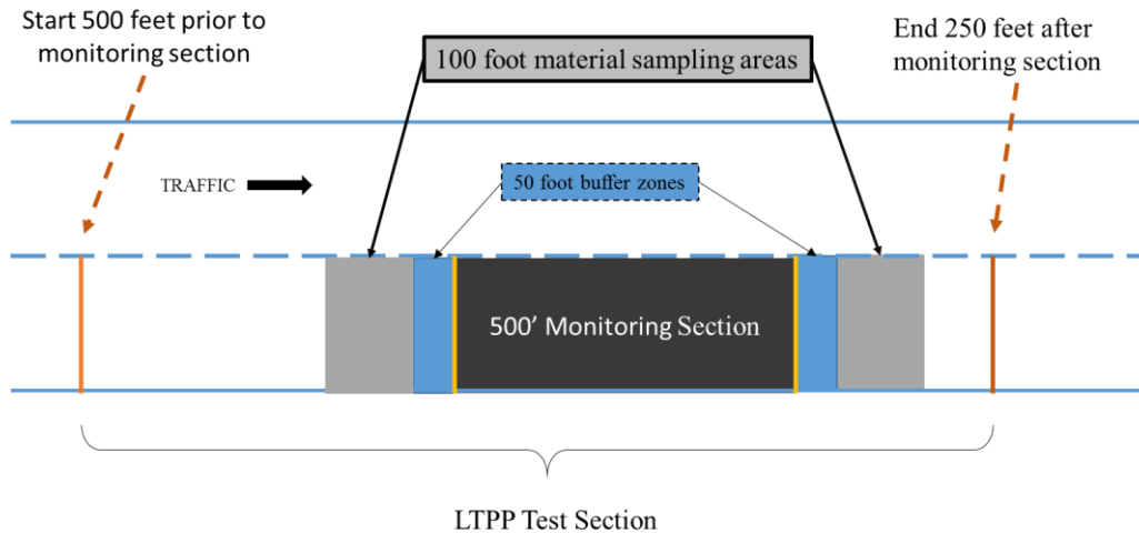
Figure 6. Illustration. Typical SPS-12 test section.
