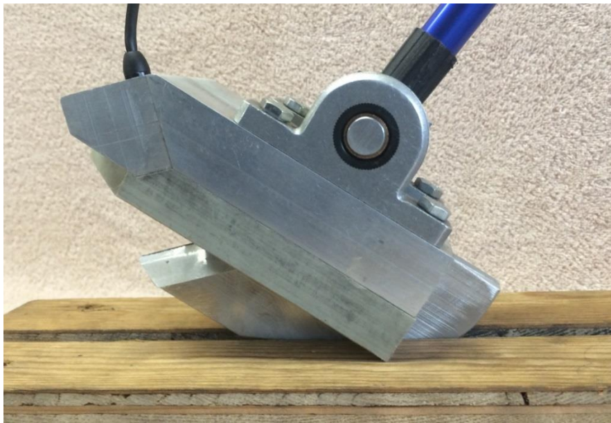
Figure 28. Photo. Insertion of the “Joint Inspection Unit.”
