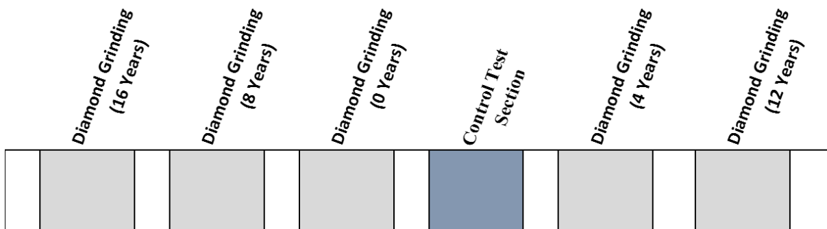
Figure 7. Illustration. Typical SPS-12G project layout: diamond grinding experiment.
