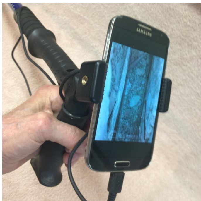
Figure 24. Photo. Handle-smart phone assembly, production prototype.
