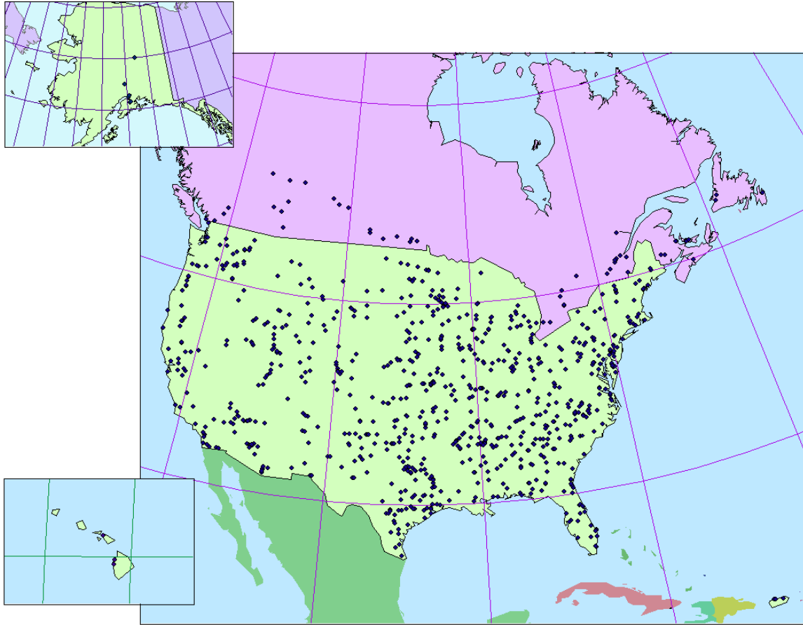
Figure 1. Map. Geographic distribution of LTPP test sections. (1)
