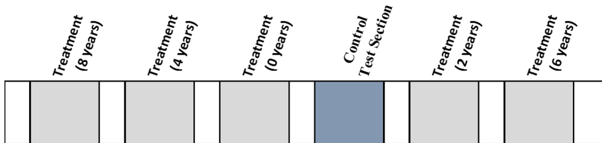
Figure 8. Illustration. Typical SPS-11T/11C/11M project layout: all experiments.
