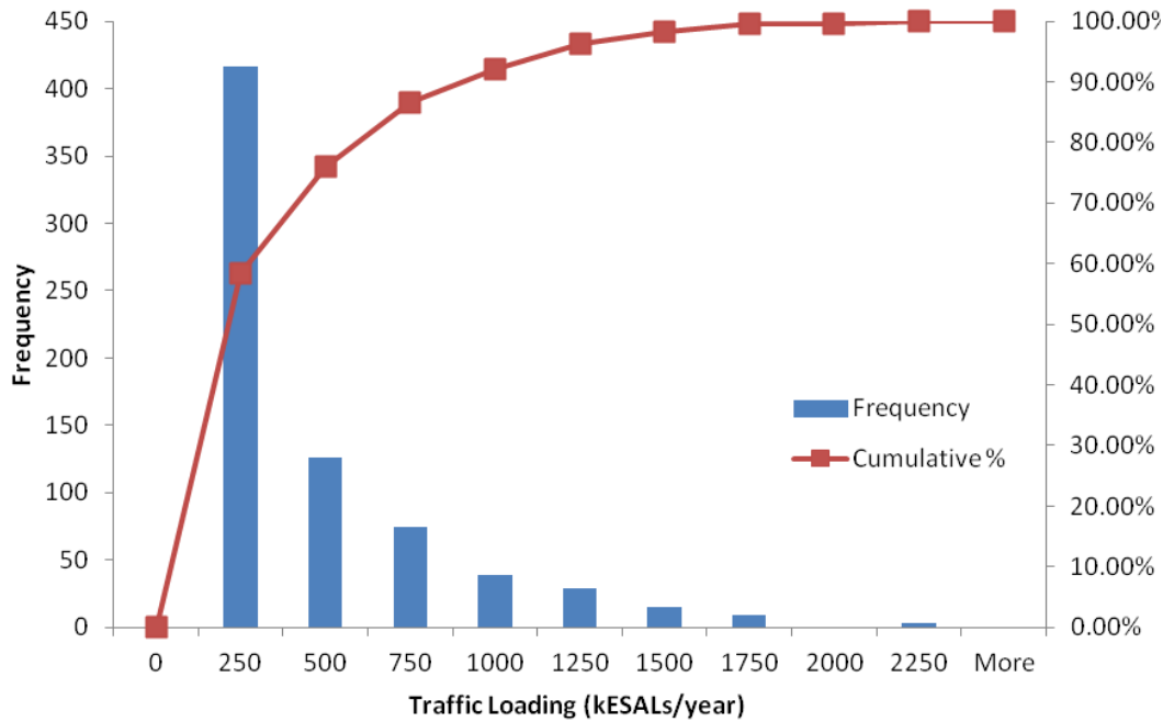
Figure 2. Graph. Distribution of annual traffic loading at LTPP sites.
