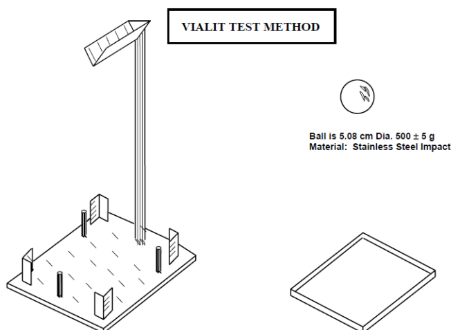
Figure 24. Illustration. Vialit testing apparatus.
