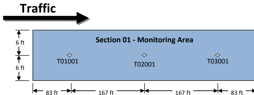
Figure 13. Illustration. In situ density/moisture measurements using nuclear density/moisture gauge for a typical section.
