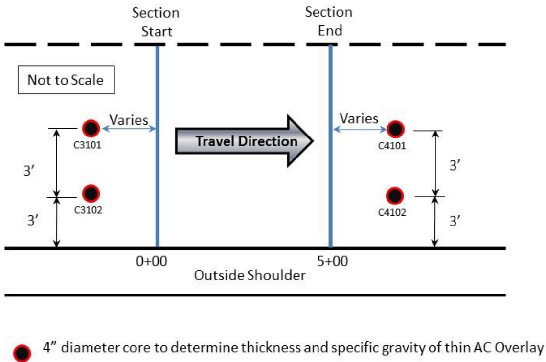
Figure 14. Illustration. Location of 4-inch cores of thin overlay on test section receiving thin overlay during each construction treatment.
