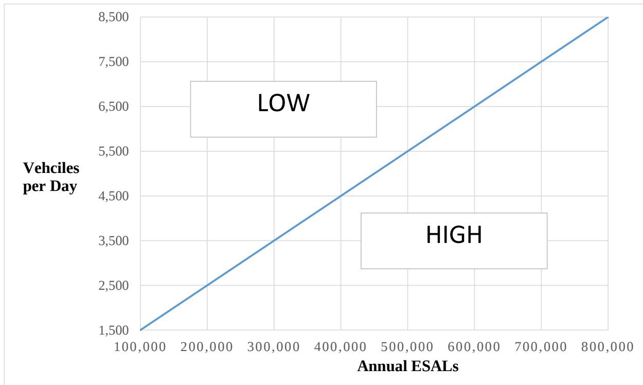
Figure 3. Graph. Chart for definition of SPS-11 traffic level.
