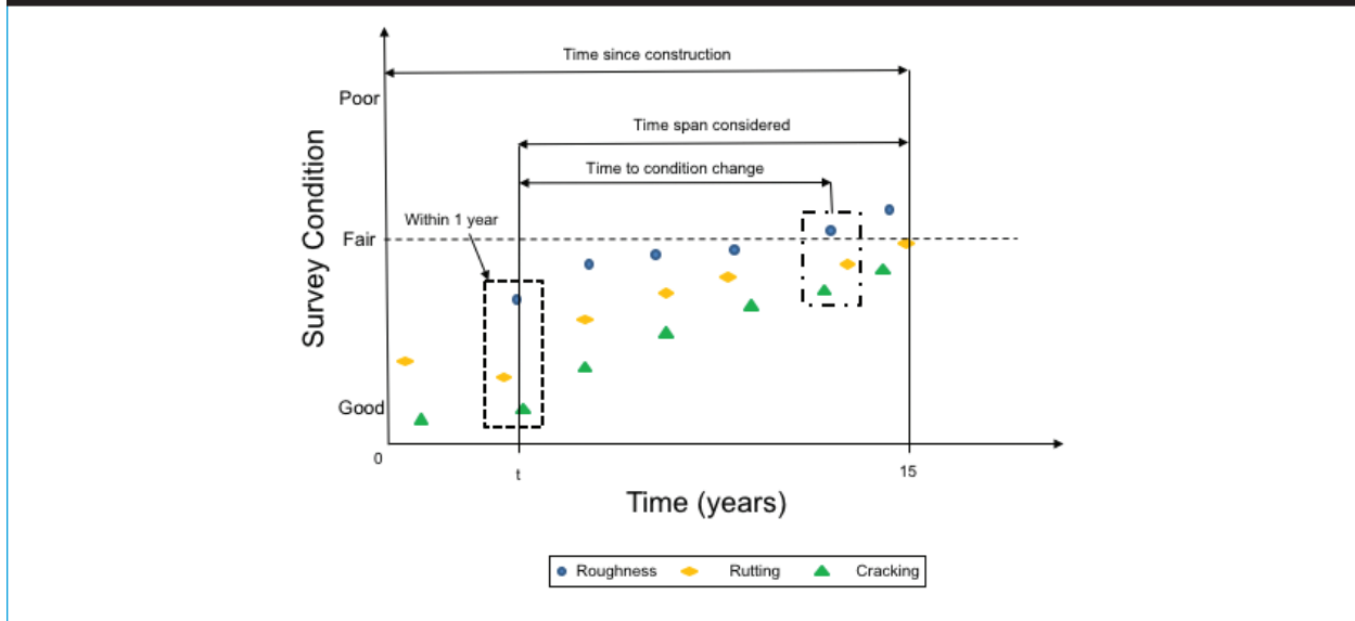
Figure 3. Temporal groupings.
