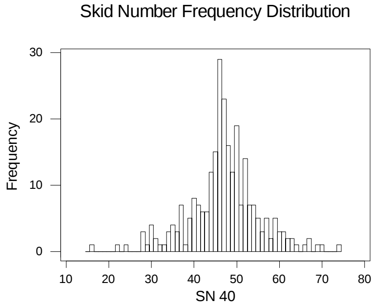
Figure 2. Skid number frequency distribution.
