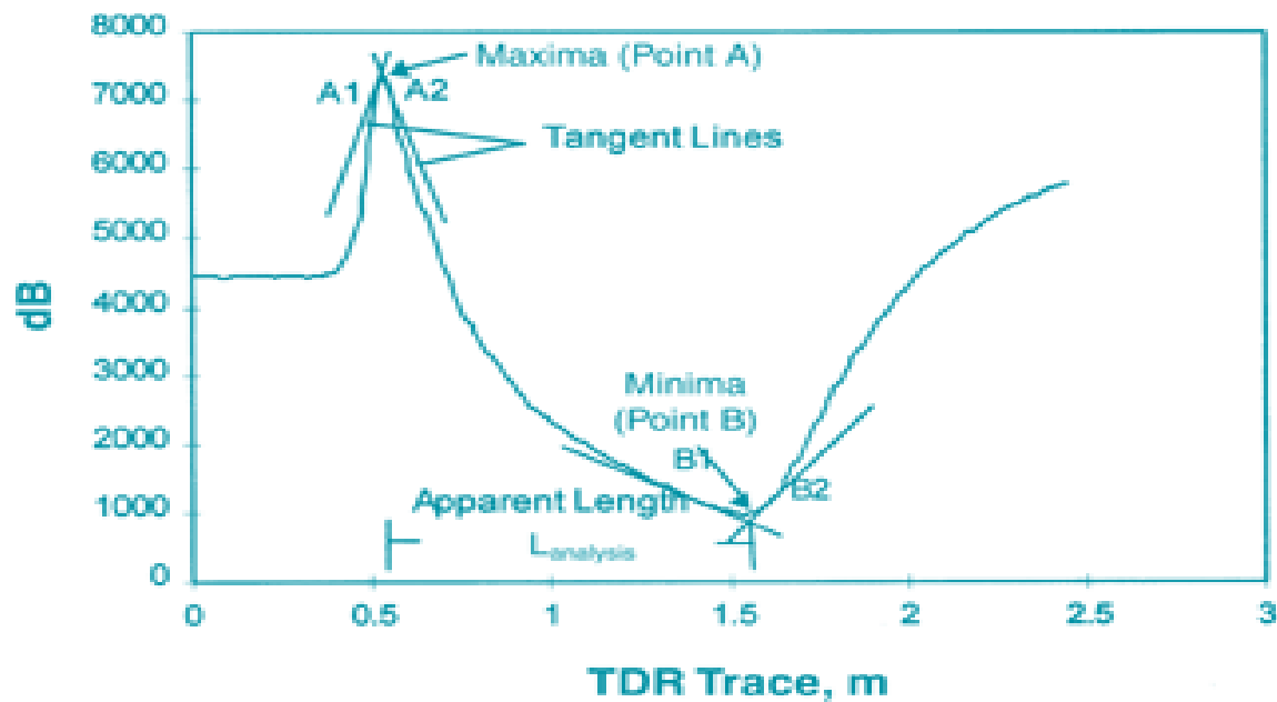
Figure 3. Illustration of the Method of Peaks.
