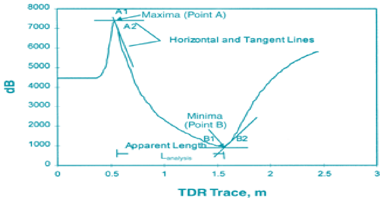
Figure 2. Illustration of the Method of Tangents.
