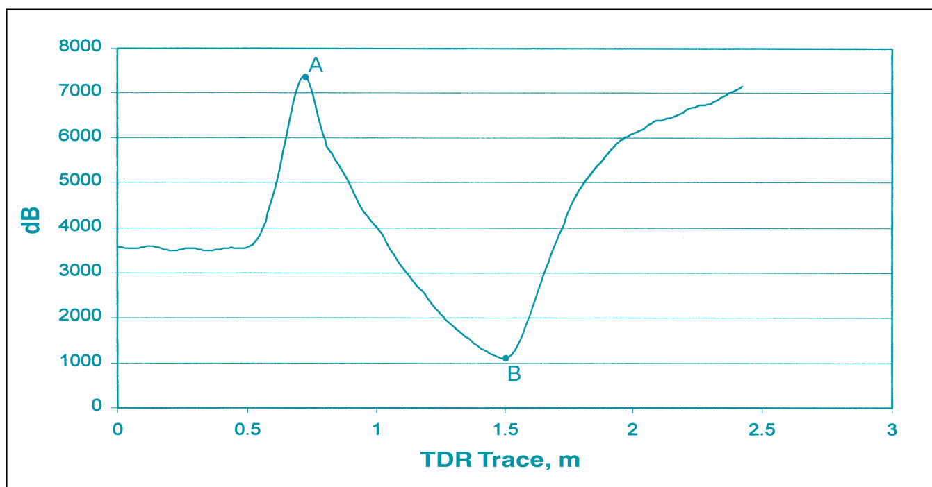
Figure 1. A classic recorded TDR trace.
