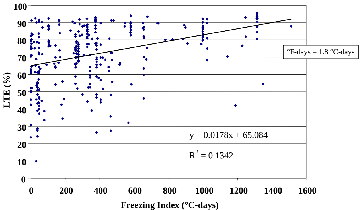
Figure 46. Freezing index versus LTE of doweled JCP.
