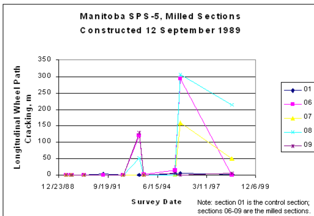
Figure 15. Graphs. Longitudinal cracking within the wheel path time-series data for the Manitoba project.
