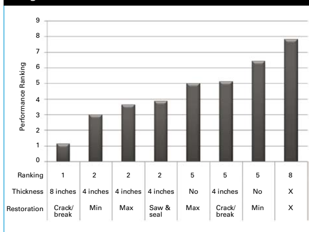
Figure 3. Performance ranking based on long-term roughness for SPS-6 JPCP sections.
