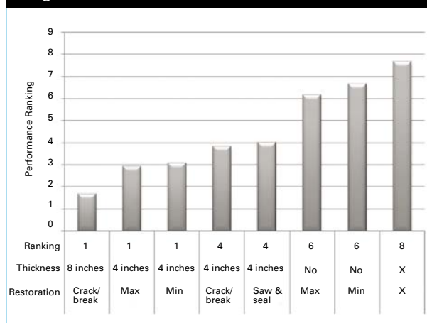
Figure 4. Performance ranking based on long-term roughness for SPS-6 JRCP sections.
