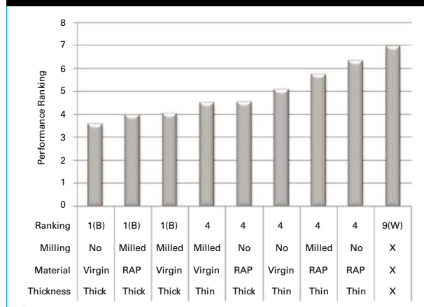
Figure 2. Performance ranking based on fatigue cracking for SPS-5 experiment.
