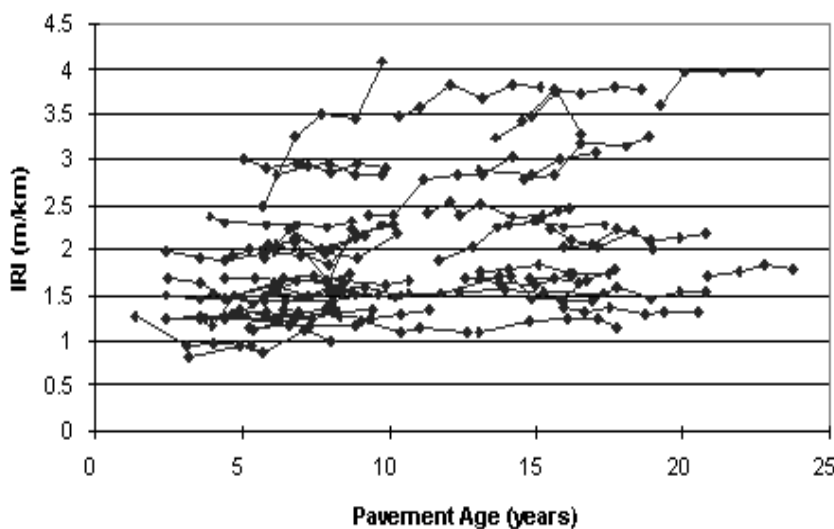
Figure 2. Roughness vs. pavement age JPCPs in wet no-freeze areas.
