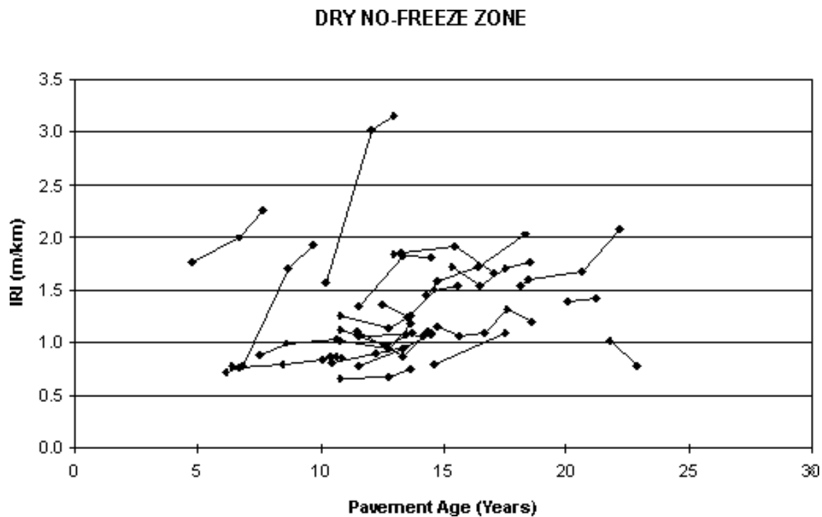
Figure 2. Roughness trends for GPS-1 sections in dry no-freeze environmental zone.
