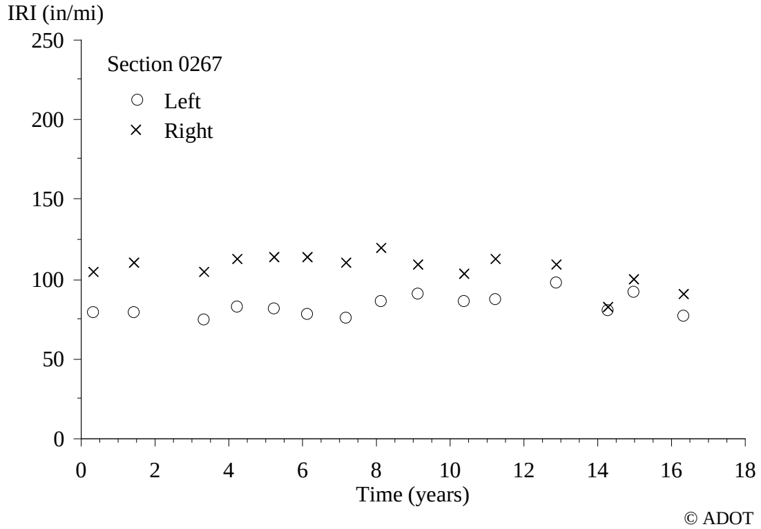
Figure 45. Graph. IRI Progression for Section 0267.
