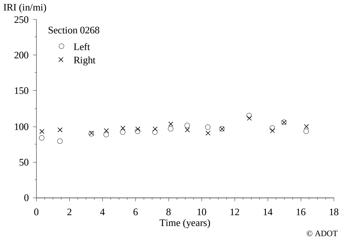
Figure 46. Graph. IRI Progression for Section 0268.
