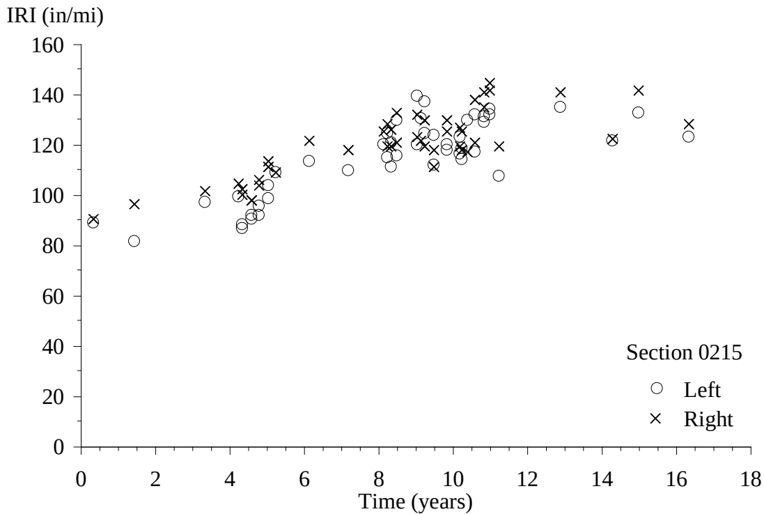
Figure 2. Graph. IRI Progression for Section 0215.
