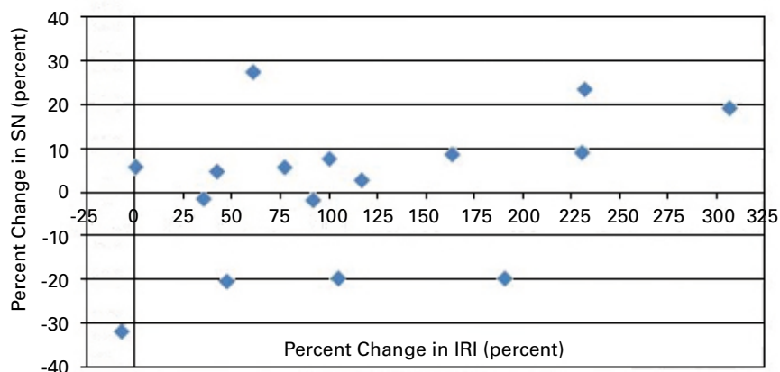
Figure 2. Relationship between percent change in IRI and SN.
