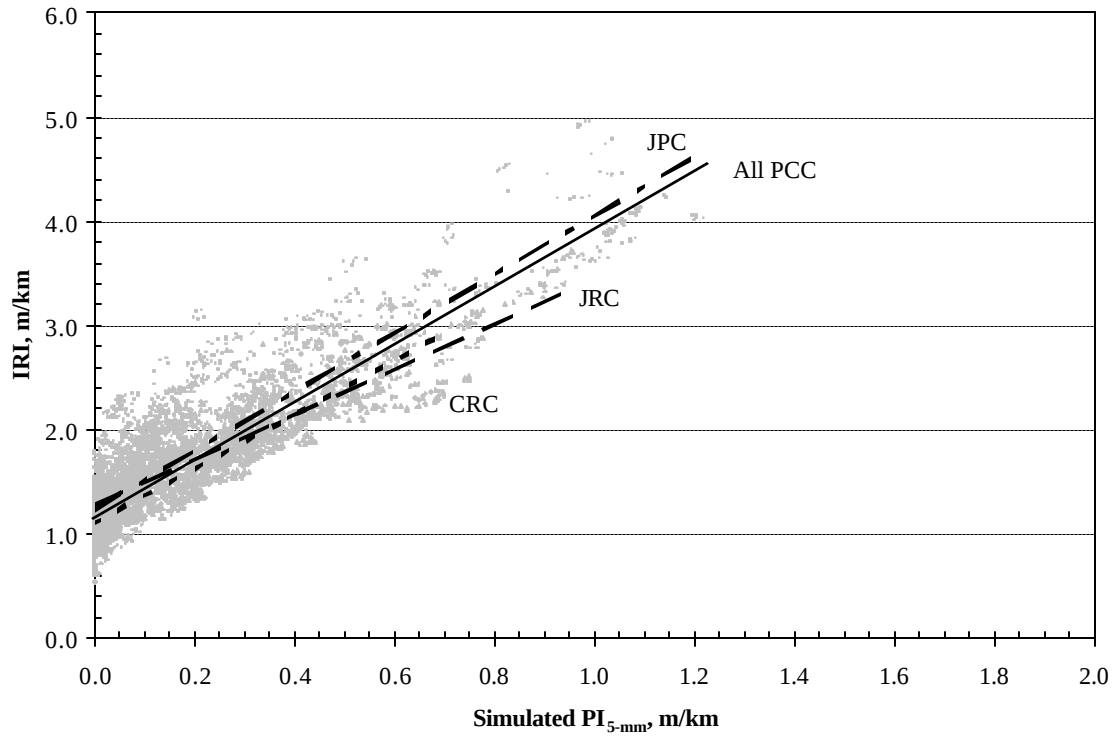
Figure B-7. IRI vs. PI_{5\text{-mm}} by PCC pavement type for all climatic zones.
