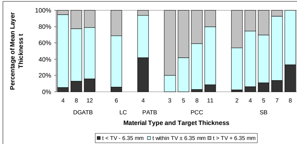
Figure 73: Chart. Results of one-sided t-tests for the differences between core measurements and design thicknesses for tolerance level of 6.35 mm (0.25 in).
