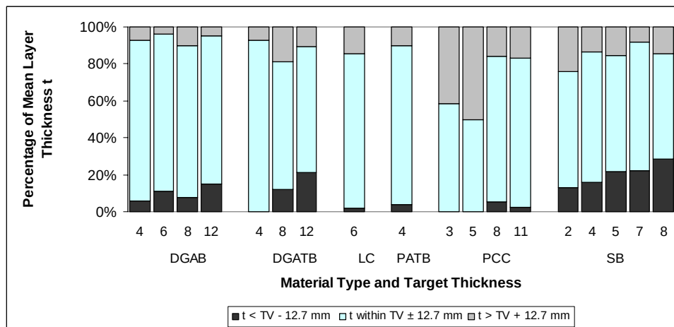
Figure 68: Chart. Results of one-sided t-tests for the differences between mean elevation and design thicknesses for a tolerance level of 12.7 mm (0.5 in).
