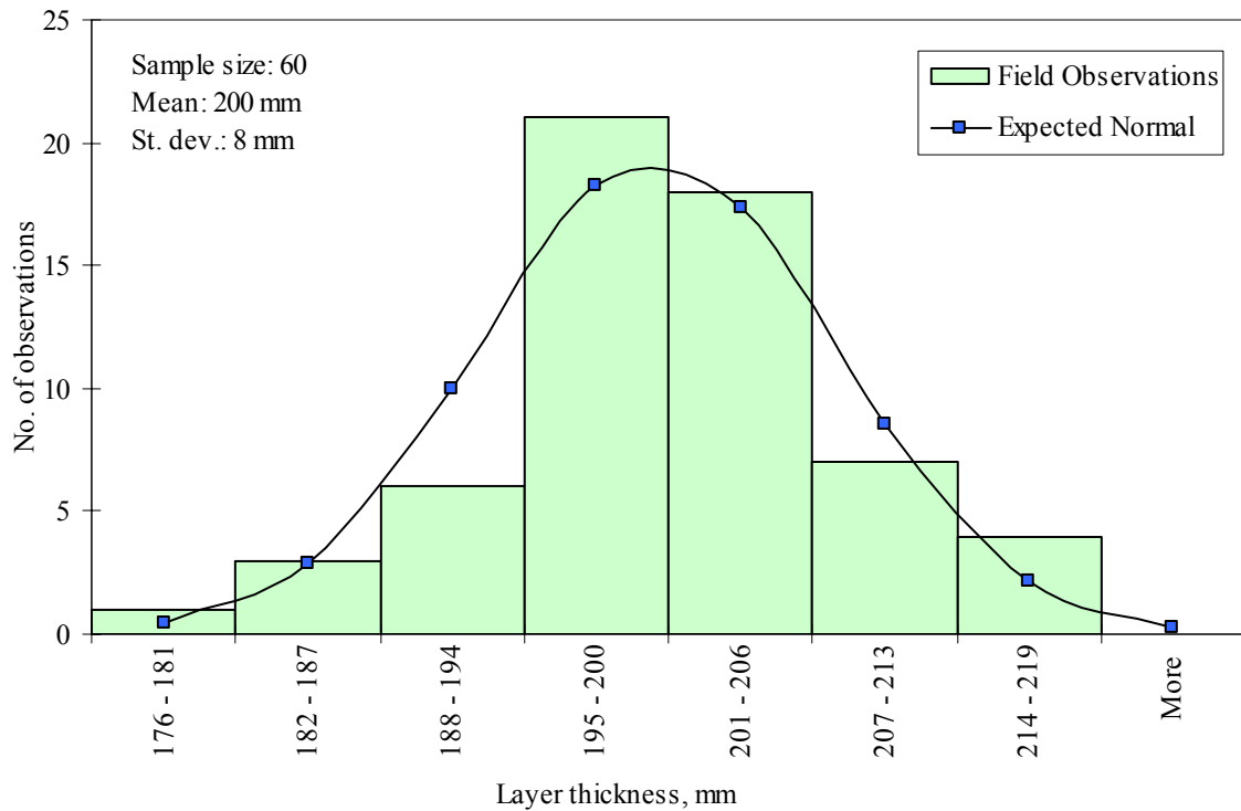
Figure 37: Chart. Example distribution of layer thickness measurements along the section for the PCC surface layer for the SPS-8 Section 39-0809.
