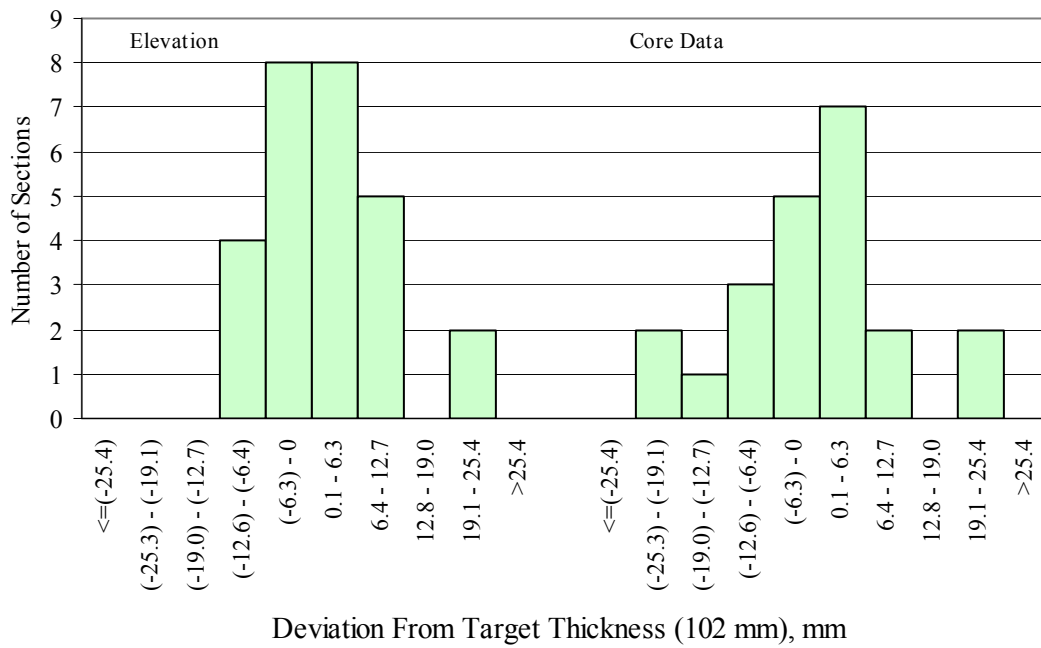
Figure 48: Chart. Frequency distribution of elevation and core thickness measurements deviations for DGATB with 102-mm (4-in) target thickness.
