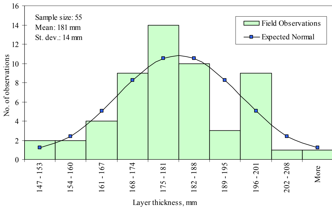
Figure 32: Chart. Example distribution of layer thickness measurements along the section for the DGATB layer for the SPS-1 Section 22-0118.
