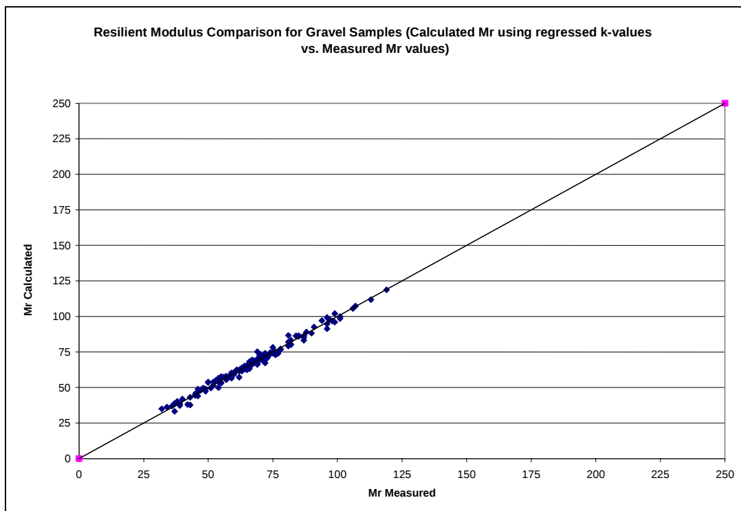
Figure 7. Graphical comparison of the calculated M_R (using the regressed k-coefficients from the LTPP test results) to the measured M_R for the gravel soils.
