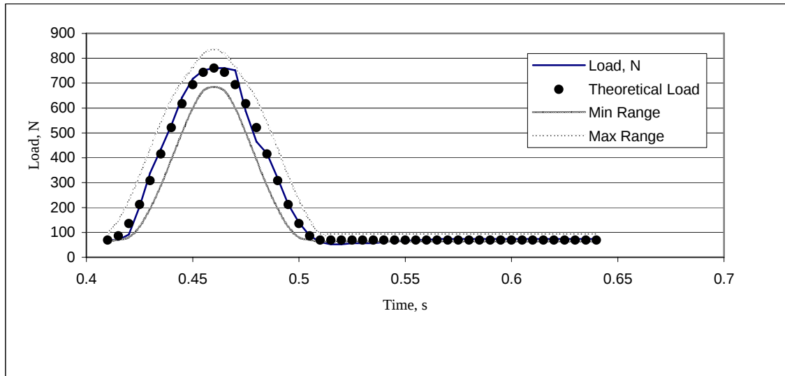
Figure 10. Graph. Example of load versus time check.
