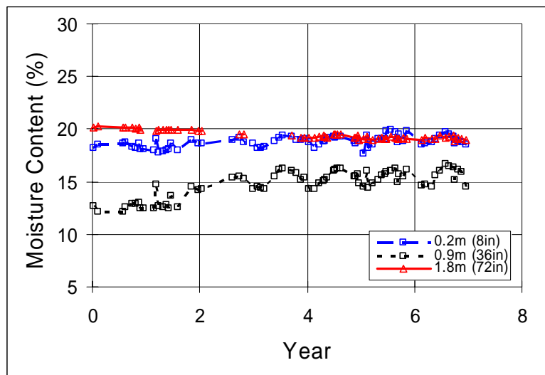
Figure 9. Moisture Variations in OH Section 390108 with PATB and GB
