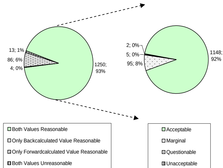
Figure 61. Charts. Screening results of the section average elastic moduli of the PCC slab for the rigid sections in the MON_DEFL_FLX_BAKCALC_SECT table based on the linear elastic model using MODCOMP.
