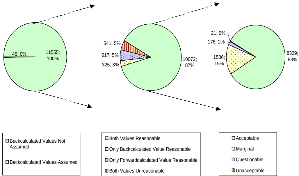
Figure 36. Charts. Screening results of elastic moduli of the interior concrete slab for the rigid sections in the MON_DEFL_FLX_BAKCALC_POINT table based on the linear elastic model for backcalculation and an unbonded condition between the slab and base for forwardcalculation.
