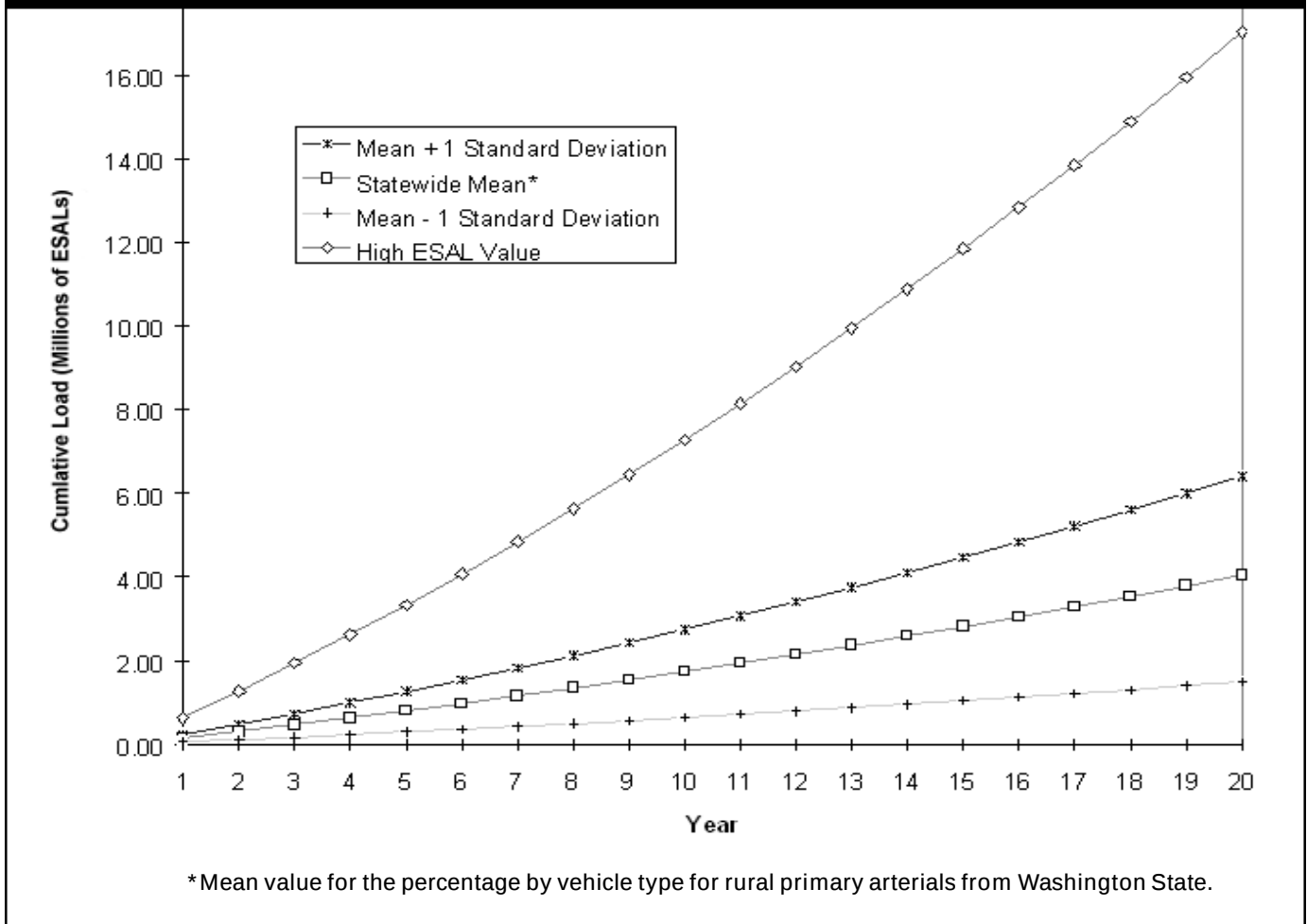
Figure 1. Cumulative ESAL loading as a function of truck percentage over time.
