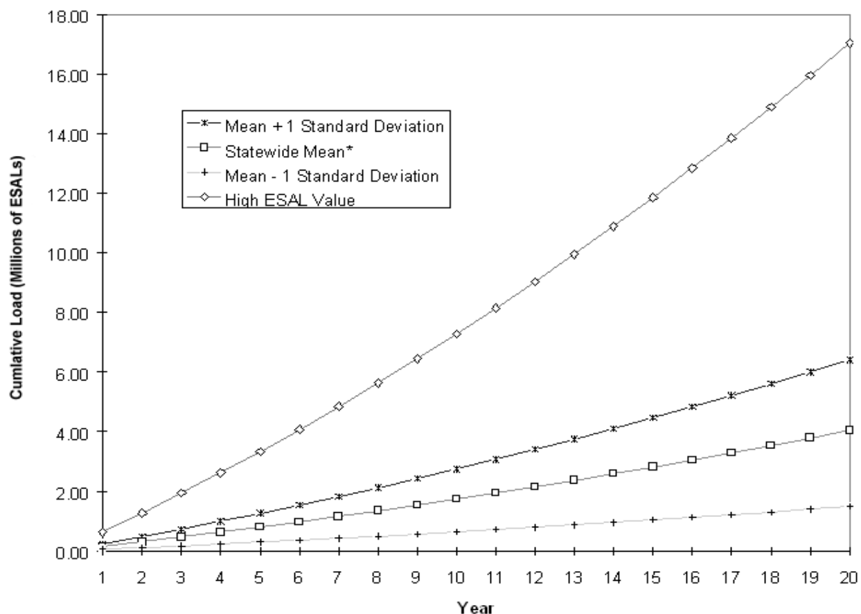
Figure 2. Effect of load and vehicle percentage on design ESALs.
