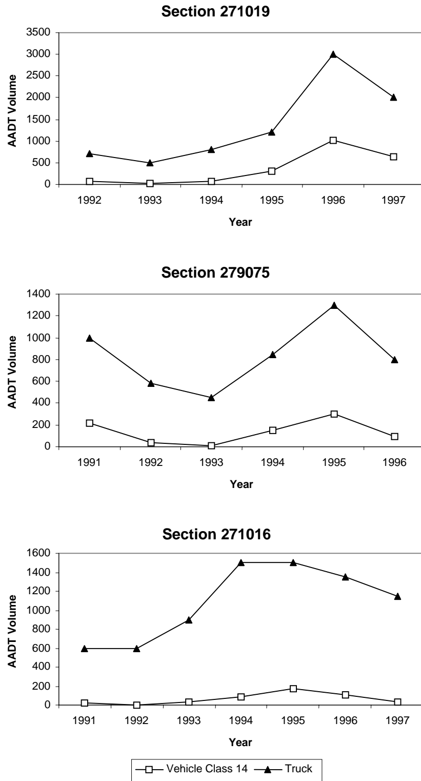
Figure 12. Comparison of AADT volumes for Class 14 vehicles with AADT volumes for all trucks.
